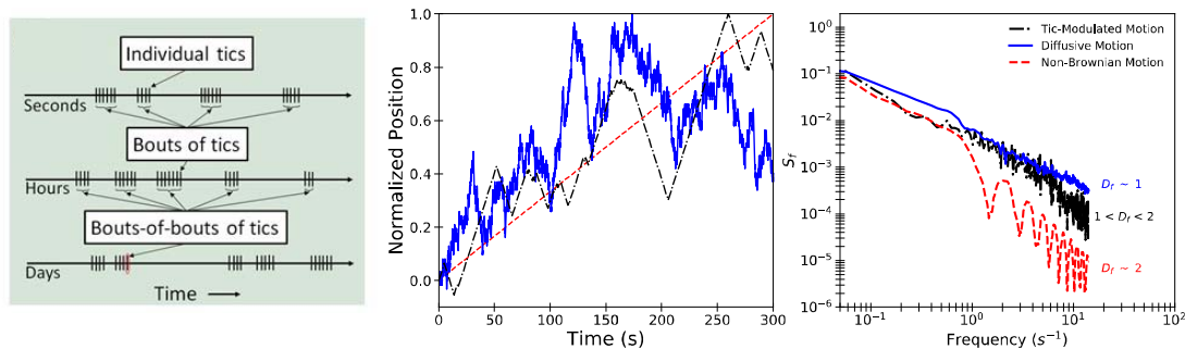
Figure 1. (left) Fractal pattern in the occurrence of tics, adapted from (7). (center) Trajectory of a tic-modulated random walk (black) is compared with that of normal diffusion (blue) and non-Brownian motion (red). The position of each walker at time t is normalized by the maximum displacement of the walker from t = 0 to t = 300 , rendering the trajectories in one-dimensional space as a function of time. (right) Estimation of D_f ( 1 < D_f < 2 ) for a walker undergoing diffusive motion (blue), non-Brownian motion (red), and tic-modulated motion (black).
