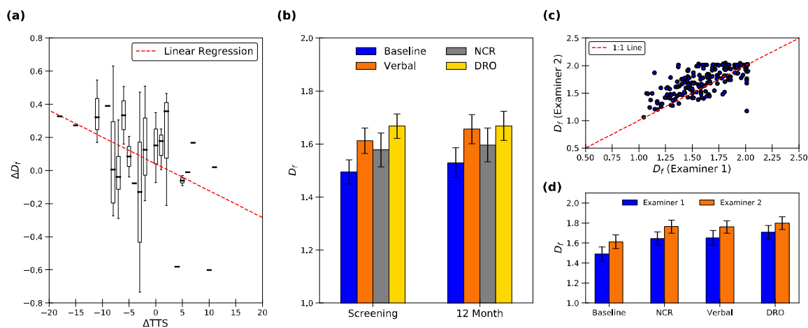
Figure 2. (a) Change in fractal dimension ( D_f ) between screening and 12 month visit as a function of change in YGTSS total tic score (TTS). The red dashed line shows linear regression of \Delta D_f vs \Delta TTS , r = -0.333 (b) Comparison of average D_f for the patients under various suppression conditions during screening visits shows that DRO led to the most effective tic suppression (largest D_f ). Additionally, the fractal dimension of all suppression conditions increased at 12 months (when most patients met diagnostic criteria for TS). (c-d) Comparison of D_f for tic time series generated by 2 examiners, with examiner 2 being blind to visit and condition. Good agreement is observed between examiners, verifying inter-rater reliability of results. All error bars show 95% confidence intervals.
