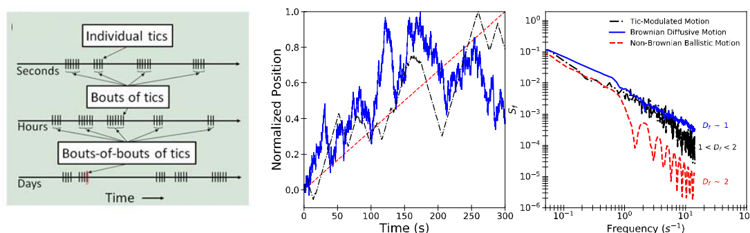
Figure 1. (left) Fractal pattern in the occurrence of tics, adapted from (7). (center) Trajectory of a tic-modulated random walk (black) is compared with that of Brownian diffusive motion (blue) and non-Brownian ballistic motion (red). The position of each walker at time t is normalized by the maximum displacement of the walker from t = 0 to t = 300 , rendering the trajectories in one-dimensional space as a function of time. (right) Estimation of D_f ( 1 < D_f < 2 ) for a walker undergoing diffusive motion (blue), non-Brownian motion (red), and tic-modulated motion (black).
