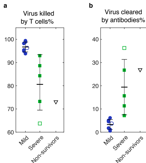
Figure 3. An overall statistic of the fraction of virus killed by T cells (a) and antibodies (b) for all cases. Solid markers are individual data, and hollow markers are group data. Error bars represent standard errors.
