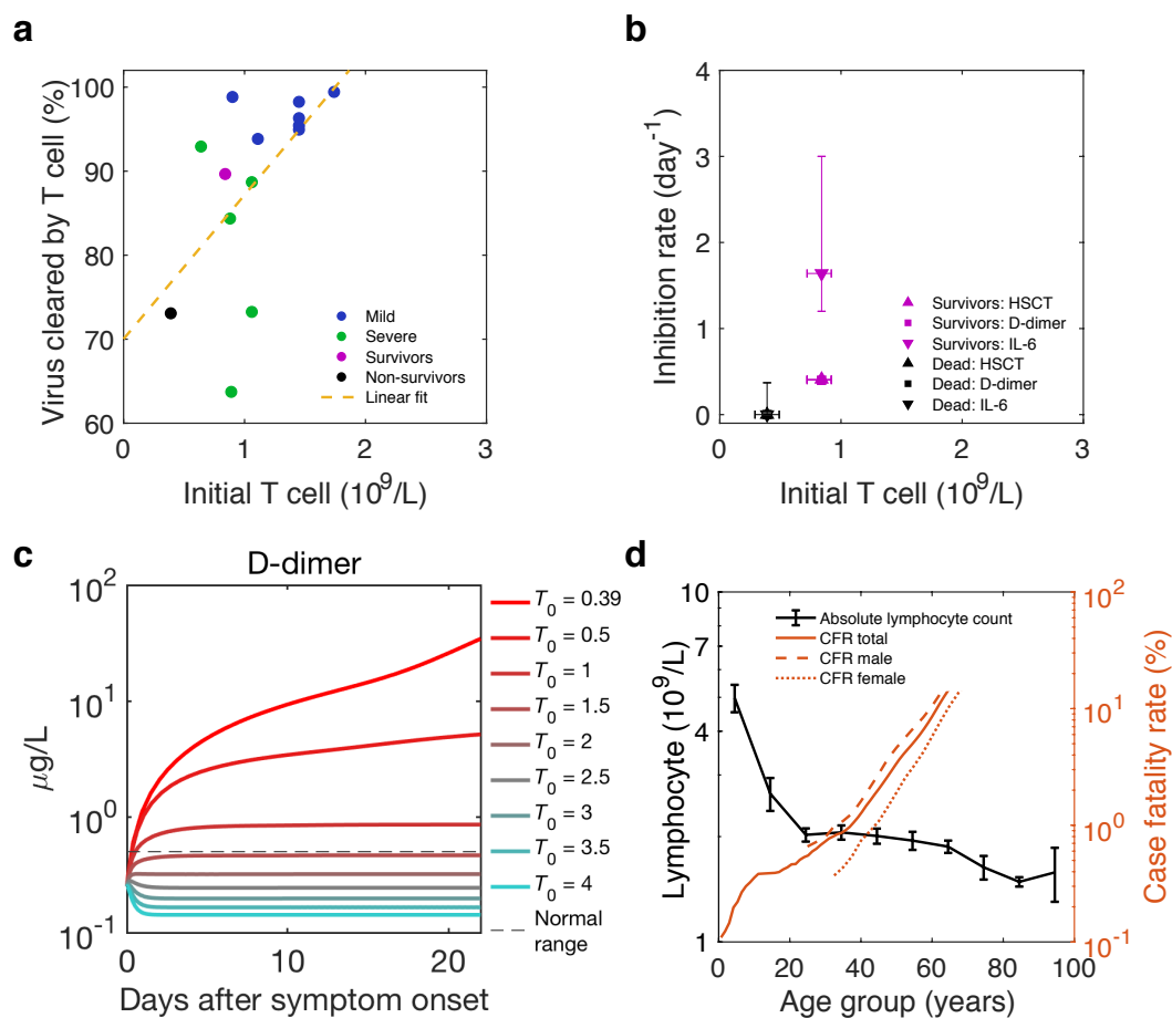
Figure 5. Initial T cell concentration as the background immunity of individuals against SARS-CoV-2 and reduces mortality. a and b: T cell’s antiviral contribution, IL-6, D-dimer, and high sensitive cardiac troponin (HSCT) inhibition rates are positively correlated with initial T cell concentration. R square of the linear fit in Figure 5a is 0.33. c: D-dimer dynamics of non-survivors with an increase of initial T cell concentration ( T_0 ) reduces organ damage at the late stage. The Red dashed line is the normal upper limit of the D-dimer, and the grey dashed line is the median value of the non-survivor group from reference 35 . For parameters of the simulation, see Methods. d. Lymphocyte count decreases with age and mortality (case fatality rate, CFR) increases with age. Male (dashed line) have higher mortality than female (solid line).
