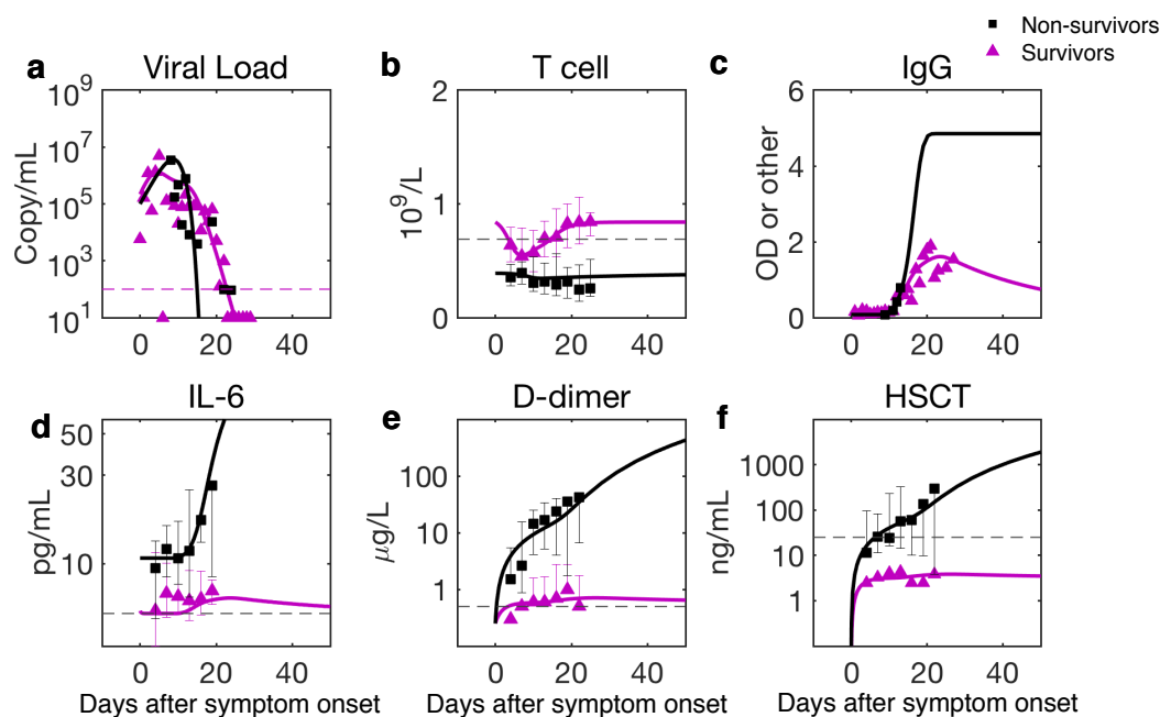
Figure 4. Comparison of predictions to clinical data of survivors and non-survivors. The data are the median of the group with error bars 35 . For parameter estimation, see Methods and SI. The saturation value of Anti-RBD IgG for non-survivors is estimated by assuming its ratio to the maximum of survivors' (18 non-critical and three critical) data is close to the ratio of maximums of neutralizing antibodies between critical and non-critical patients 40 .
