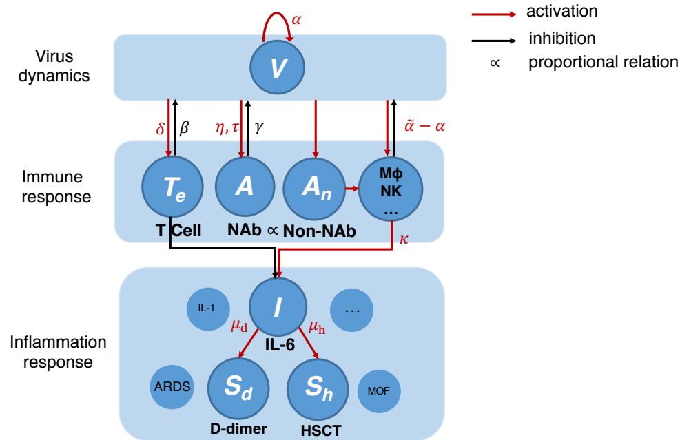
Figure 1. Graphical scheme of COVID-19 antiviral-inflammation model. Key components are highlighted. The red arrows mean activation, and the black arrows represent inhibition. Greek letters mean the activation/inhibition rates or characteristic time associated with each interaction NAB: neutralizing antibody. Non-NAB: non-neutralizing antibody of which the concentration is assumed proportional to NAB. M\phi , NK: macrophage and natural killer cells. IL-6: interleukin 6. IL-1: interleukin 1. D-dimer: coagulation marker. HSCT: High-sensitivity cardiac troponin I, heart injury marker. ARDS: Acute Respiratory Distress Syndrome. MOF: Multi-Organ Failure.
