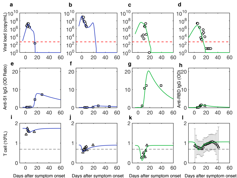
Figure 2. Viral dynamics, adaptive immune response, and contributions of T cells to antiviral responses. a, e, i are fits of the first patient (patient ID labelled as P1); b, f, j are fits of the second patient (patient ID labelled as P3); c, g, k are fits of the third patient (patient ID labelled as P5) 36 ; d, h, l are fits of the fourth patient (patient ID labelled as 902). Because the fourth patient lacks T cell data, we use T cell data from severe group 3 as the T cell value for the fourth patient. Mild patients are in blue and severe patients are in green. Red dotted lines are the limit of detection 31 . Black dotted lines are normal ranges 3 . Viral load is from the nasopharyngeal swab.
