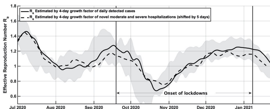
FIG. M.3: Solid line: Effective reproduction number estimated by the 4-day growth factor of either detected cases (full line), with its standard deviation (shaded area); Dashed line: moderate and severe new daily hospitalizations, shifted back 5 days to maximally correlate to the detected cases.
