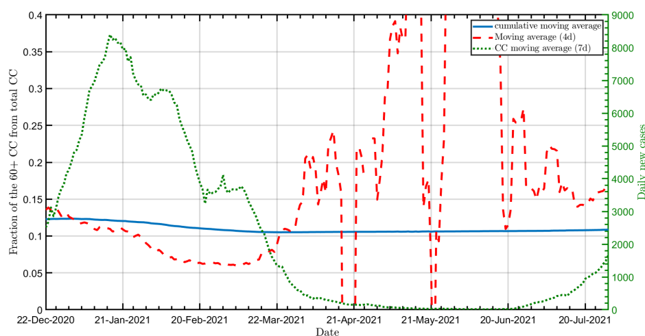
FIG. 2: Percentage of verified persons aged 60+ among all verified persons as of January 2021. Solid line: cumulative moving average dashed line: 4 days moving. Dots: the daily total confirmed cases.(all the data was taken from Refs. [2? ]
