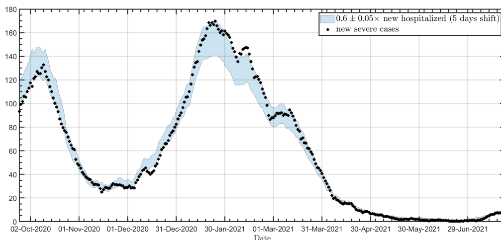
FIG. 1: The correlation between the new daily severe and moderate hospitalized and the new severe hospitalized after five days. Dots: new severe hospitalized; Solid blue band: 0.6 \pm 0.05 \times the new severe and moderate hospitalized with five days shift (all the data was taken from Refs. [1, 2])
