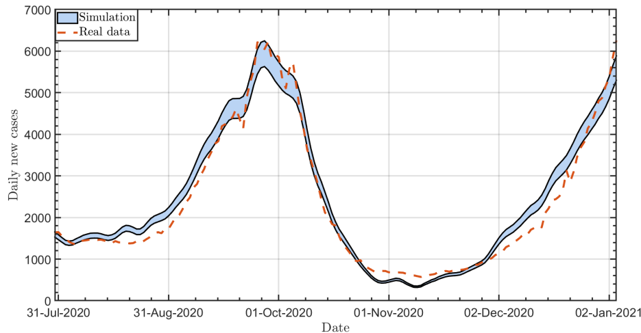
FIG. M.1: The daily new confirmed cases between Aug 1st and Jan 6th, 2021. Solid line: simulation. Dashed line: real data [1, 2]
