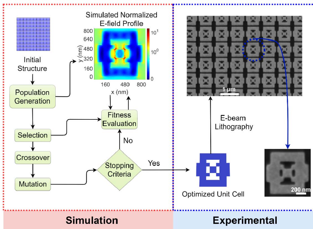
Fig. 2 | Genetic algorithm-driven computational screening and fabrication of the nanoplasmonic surface-enhanced Raman spectroscopy (SERS) biosensor chip. The genetic algorithm and the flowchart for computational screening of periodic nanostructures for maximizing the Raman cross-section of the metasurface are shown. The electron beam lithography fabrication for the optimized periodic gold nanopattern over 200 \times 200\ \mu\text{m}^2 is shown.
