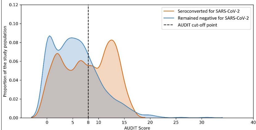
Figure 2. Kernel density estimates of AUDIT score by primary and secondary COVID-19 outcomes
