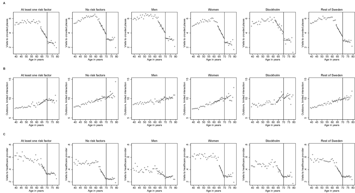
Figure S1. Regression discontinuity plots for the impact of the age-specific isolation recommendations on social distancing behaviors at the 70-year-threshold with local linear estimates in mean-squared-error-optimal bandwidths around the threshold for subgroups based on medical risk factors, sex and area (Stockholm county, rest of Sweden), for three social distancing measures:
