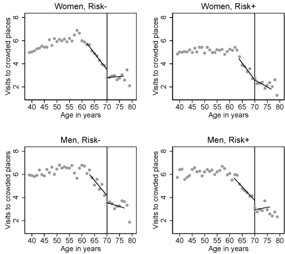
Figure S3. Regression discontinuity plots for visits to crowded places in detailed subgroups by risk factor status and sex.
