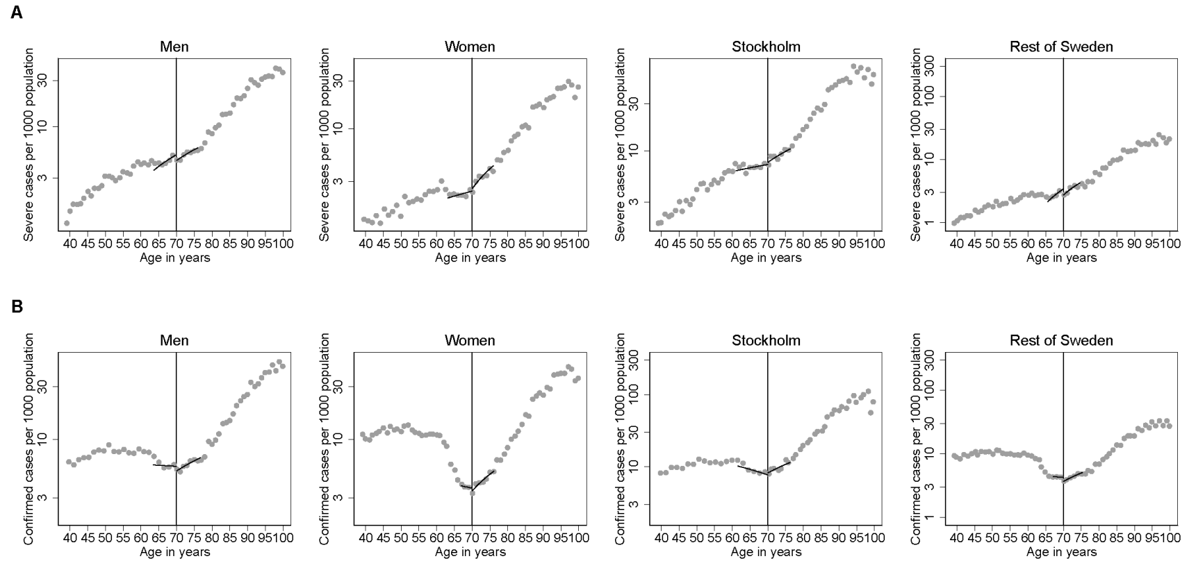
Figure S4. Regression discontinuity plots for the impact of the age-specific isolation recommendations on COVID-19 disease incidence per 1,000 population at the 70-year-threshold with local linear estimates in mean-squared-error-optimal bandwidths around the threshold in subgroups by sex and area (Stockholm county, rest of Sweden). A) Severe cases (hospitalized or dead), B) all confirmed cases. The incidence is presented on a logarithm scale to enable better visualization of the regions around the 70-year-threshold.
