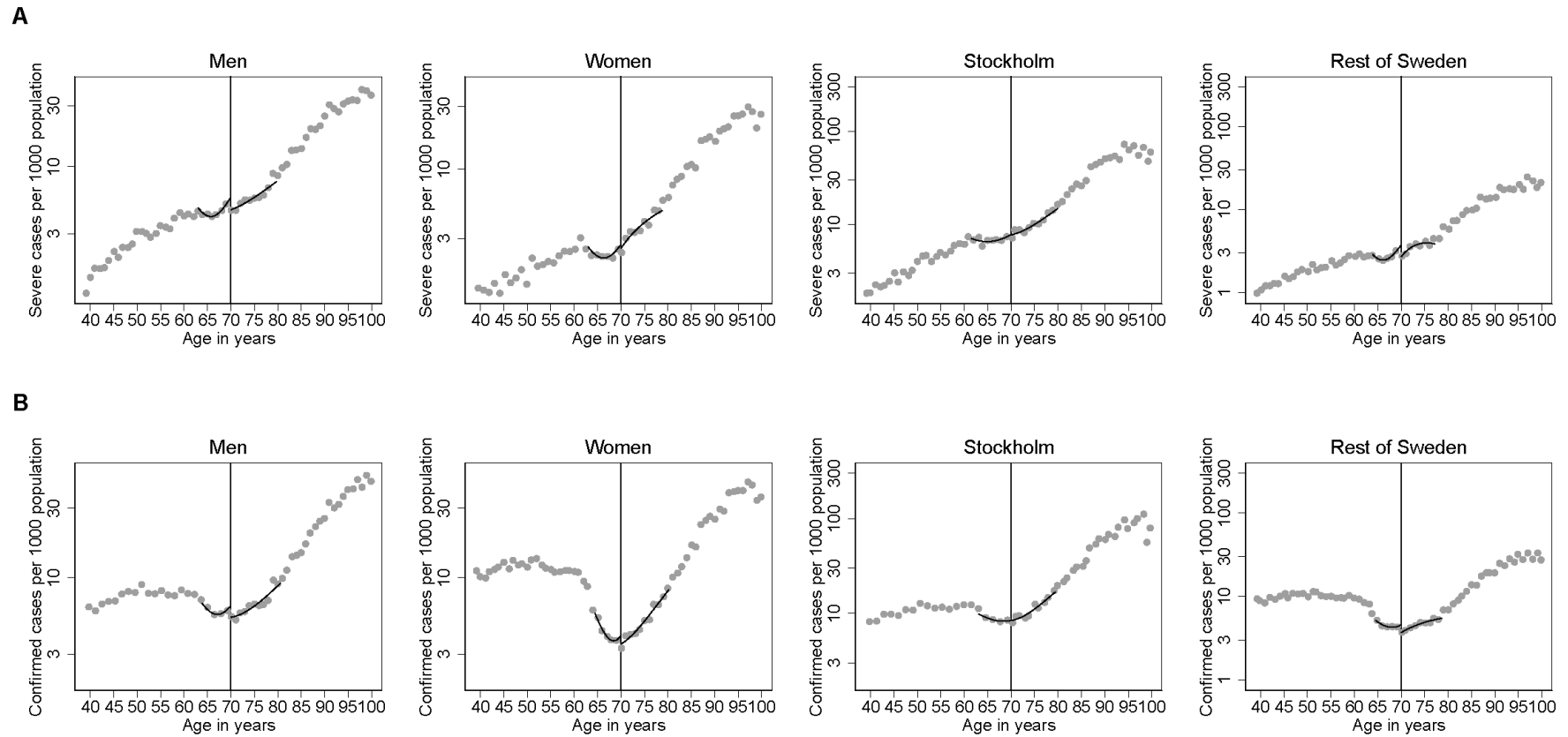
Figure S5. Regression discontinuity plots for the impact of the age-specific isolation recommendations on COVID-19 disease incidence per 1,000 population at the 70-year-threshold with local quadratic estimates in mean-squared-error-optimal bandwidths around the threshold in subgroups by sex and area (Stockholm county, rest of Sweden). A) Severe cases (hospitalized or dead), B) all confirmed cases. The incidence is presented on a logarithm scale to enable better visualization of the regions around the 70-year-threshold.
