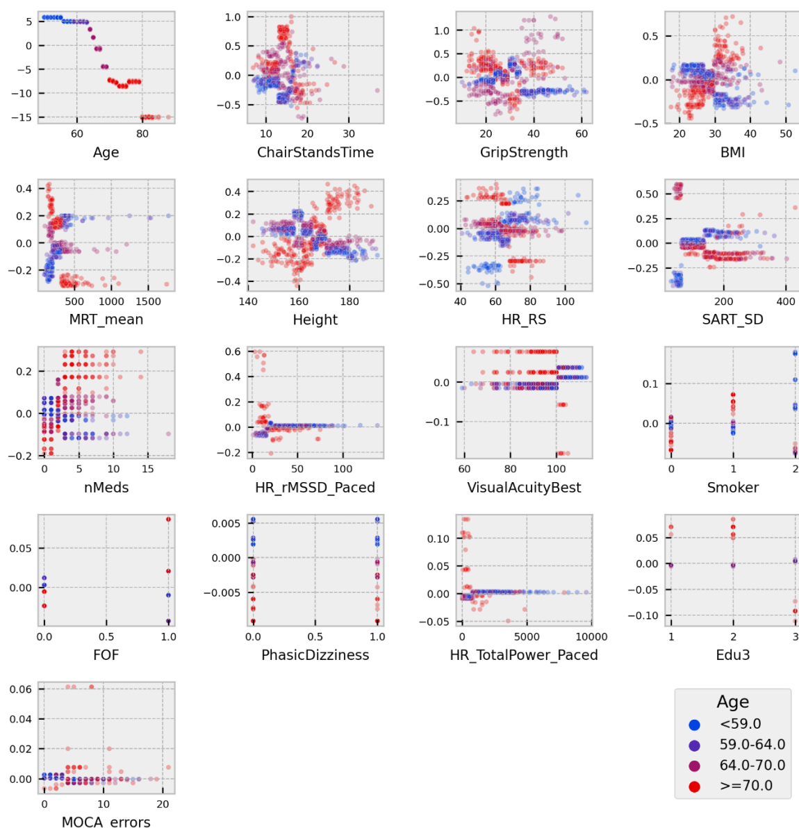
Figure 1 - SHAP values for the interaction between age and all features in the maximum speed model. The x-axes present the values of a feature in the units of that feature. The colour of a point indicates what quartile for age that sample falls in. The y-axis displays the SHAP value of the interaction.
