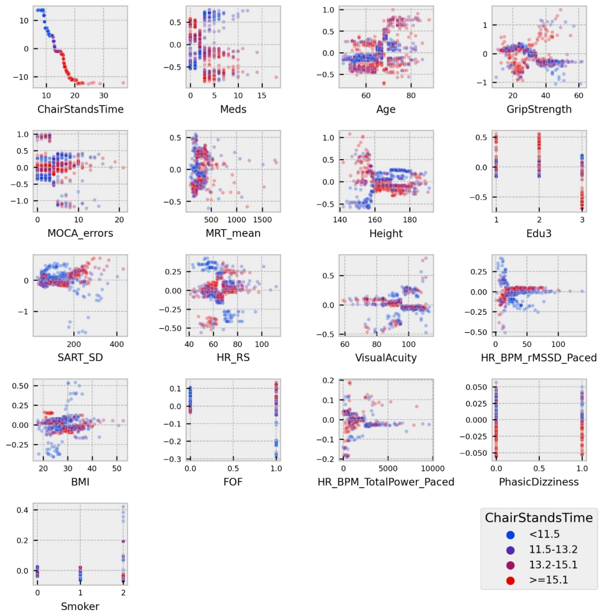
Figure 3 - SHAP values for the interaction between chair stands time and all features in the maximum speed model. The x-axes present the values of a feature in the units of that feature. The colour of a point indicates what quartile for chair stands time that sample falls in. The y-axis displays the SHAP value of the interaction.
