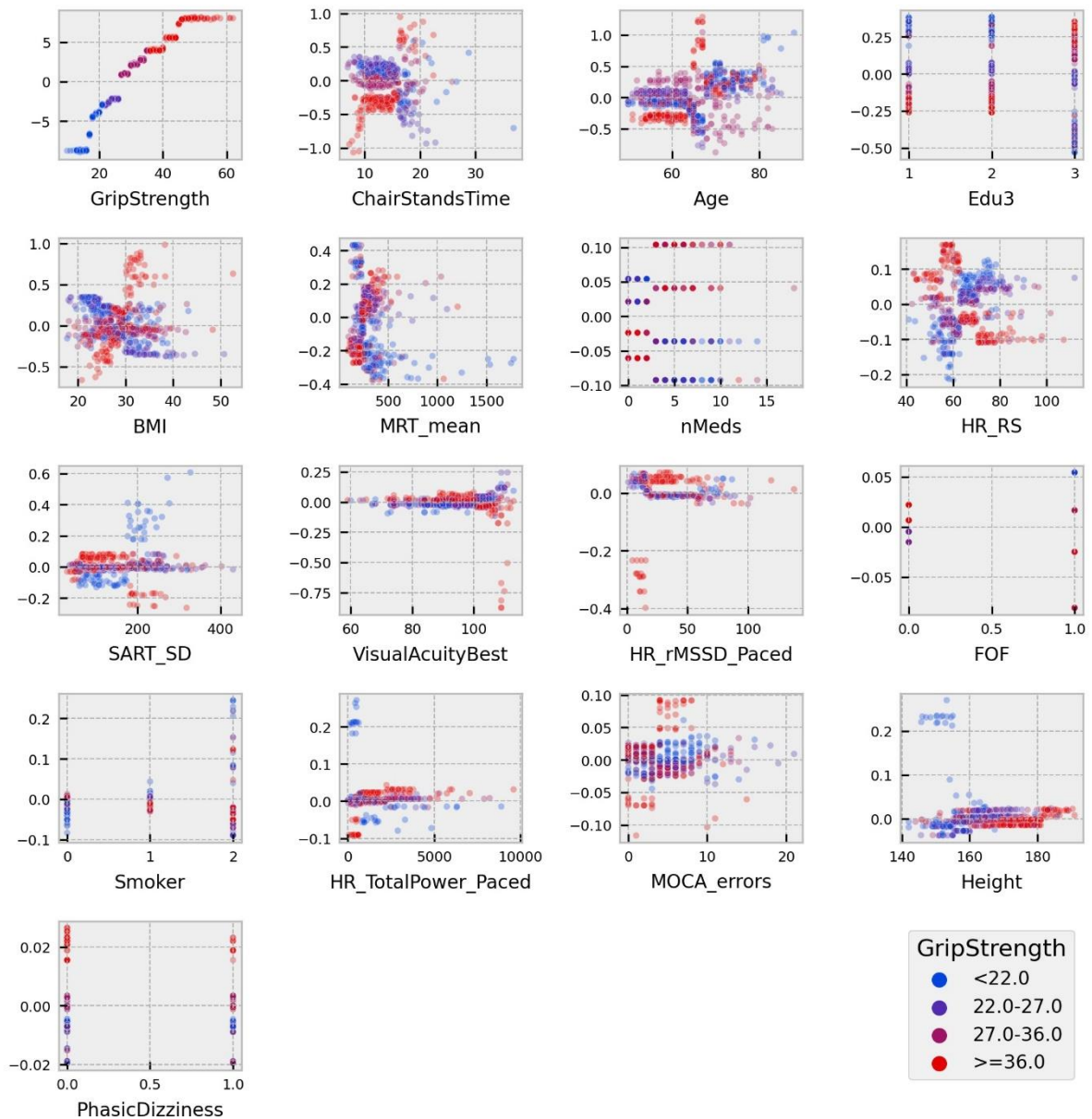
Figure 2 - SHAP values for the interaction between grip strength and all features in the maximum speed model. The x-axes present the values of a feature in the units of that feature. The colour of a point indicates what quartile for grip strength that sample falls in. The y-axis displays the SHAP value of the interaction.
