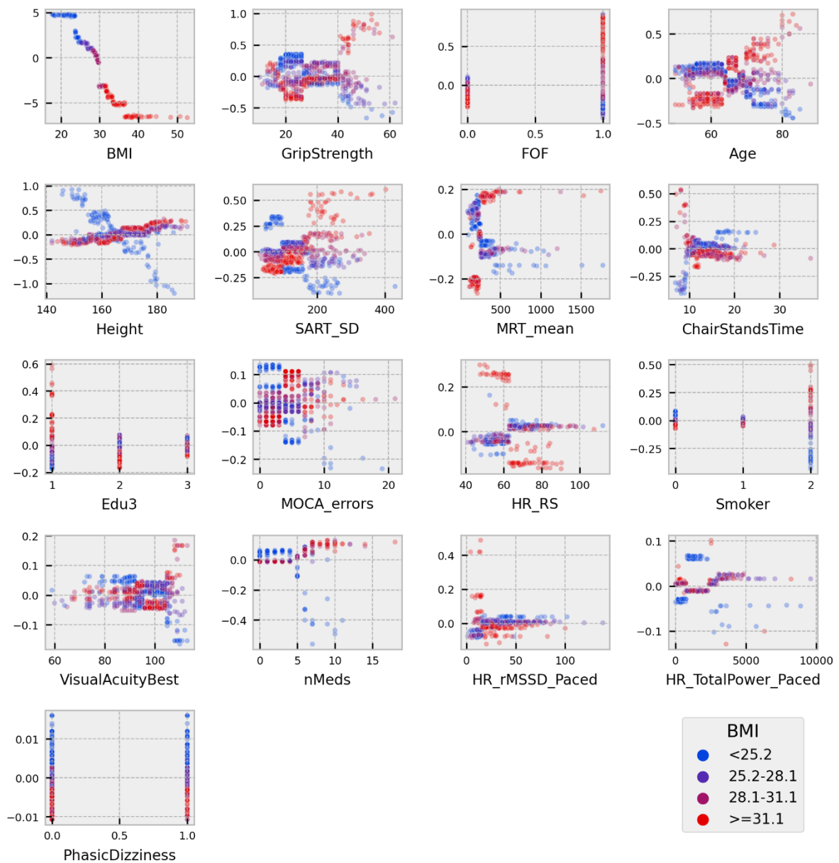
Figure 4 - SHAP values for the interaction between BMI and all features in the maximum speed model. The x-axes present the values of a feature in the units of that feature. The colour of a point indicates what quartile for BMI that sample falls in. The y-axis displays the SHAP value of the interaction.
