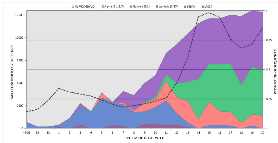
Figure 2. Number of reported cases by epidemiological week 2020-2021 since the beginning of the molecular surveillance of SARS-CoV-2 variants. Only cases that did not present a history of travel or close contact with travelers are included. Dotted line (mapped to the left y axis) indicates the average number of confirmed COVID-19 cases per week in the Metropolitan Area of Buenos Aires (MABA).
