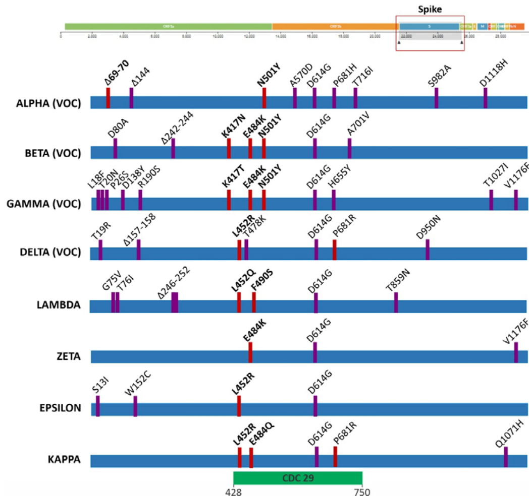
Figure 3. Representation of the amino acid changes in the S gene of SARS-CoV-2 variants of epidemiological interest. Changes indicated in red correspond to those with the greatest potential impact on viral biology or neutralization by antibodies. The location of CDC fragment 29 (codons 428 to 750) used for active surveillance of variants is indicated.
