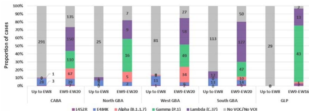
Figure 6. Cumulative number of SARS-CoV-2 variants and sequences with or without mutations of interest in the Metropolitan area of Buenos Aires (CABA, GBA and Great La Plata (GLP)). The cases were analyzed in two periods: until EW 8/2021 and from EW 9/2021 to EW 20/2021, according to the moment of change in the trend of the frequencies of the variants or mutations in each region. Only cases that did not present a history of travel or close contact with travelers are included; in cases sharing an epidemiological link, only one was considered as representative. The bars show the number of samples corresponding to variants, mutations or non-VOC/non-mutations of interest.
