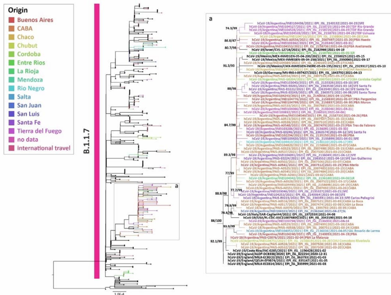
Figure 4 Phylogenetic tree of SARS-CoV-2 whole genome sequences of Alpha (lineage B.1.1.7). Dataset included sequences from Argentina, their best five BLAST hits sequences (against GISAID database on June 2 nd 2021), reference sequences of B.1.1.7 lineage, and B.1.1.1 sequences as outgroup. Only the largest group with Argentinean sequences is shown. Phylogenetic analysis was performed using IQ-TREE v. 2.1.2 COVID-edition (20). The SH-like approximate likelihood ratio test (1000 replicates) (21) and Ultrafast bootstrap Approximation (1000 replicates) (22) were used as methods to evaluate the reliability of the groups obtained. The SH-like / UFB values for the relevant groups are indicated for some groups. We gratefully acknowledge the authors from the originating laboratories responsible for obtaining the specimens and the submitting laboratories where genetic sequence data were generated and shared via the GISAID Initiative, on which part of this research is based (Table S1).
