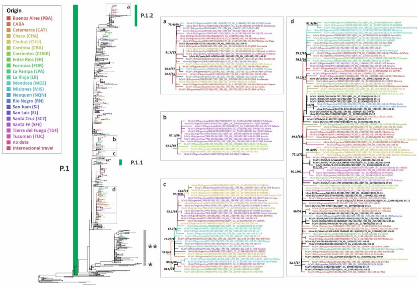
Figure 5. Phylogenetic tree of SARS-CoV-2 whole genome sequences of Gamma (lineage P.1). Dataset included sequences from Argentina, their best five BLAST hits sequences (against GISAID database on June 2 nd 2021), reference sequences of P.1 lineage, and B.1.1.28 sequences as outgroup. Only selected groups with Argentinean sequences are shown. Phylogenetic analysis was performed as previously described in Figure 5. *P.1-like-I and **P.1-like-II described by Gräf et al (9). We gratefully acknowledge the authors from the originating laboratories responsible for obtaining the specimens and the submitting laboratories where genetic sequence data were generated and shared via the GISAID Initiative, on which part of this research is based (Table S2).
