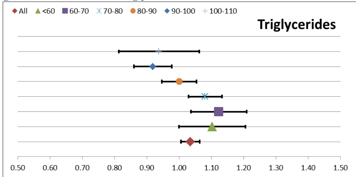
Figure S11: Associations of triglycerides levels from Deelen et al.
