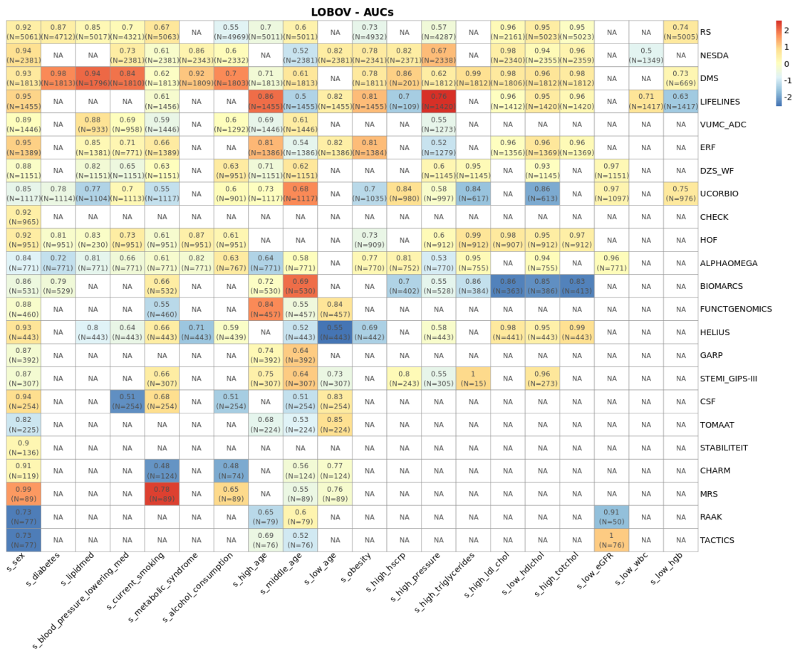
Figure S2: [A] The boxplots of the AUC obtained with LOBOV. The dots represent the AUC for each biobank, colored according to the percentage of one of the dichotomous values for the risk factor. [B] The heatmap of the AUC obtained in the LOBOV from each metabolic surrogate measure in each biobank. The AUCs are scaled based on the AUC for each metabolic model. Inside each cell we show also the available number of samples for each biobank.
