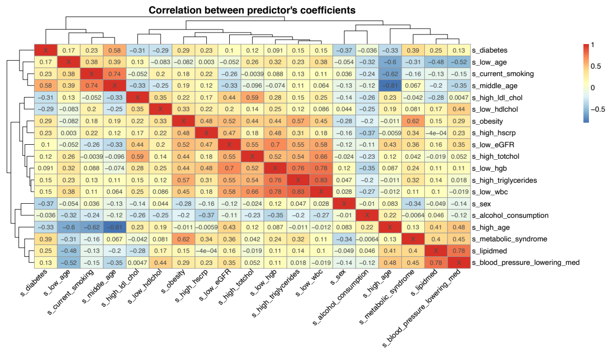
Figure S3: Correlation heatmaps between the ElasticNETs' betas of the final models.
