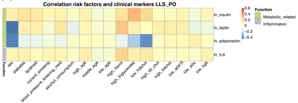
Figure S7: Correlations with additional cardio-metabolic phenotypes
