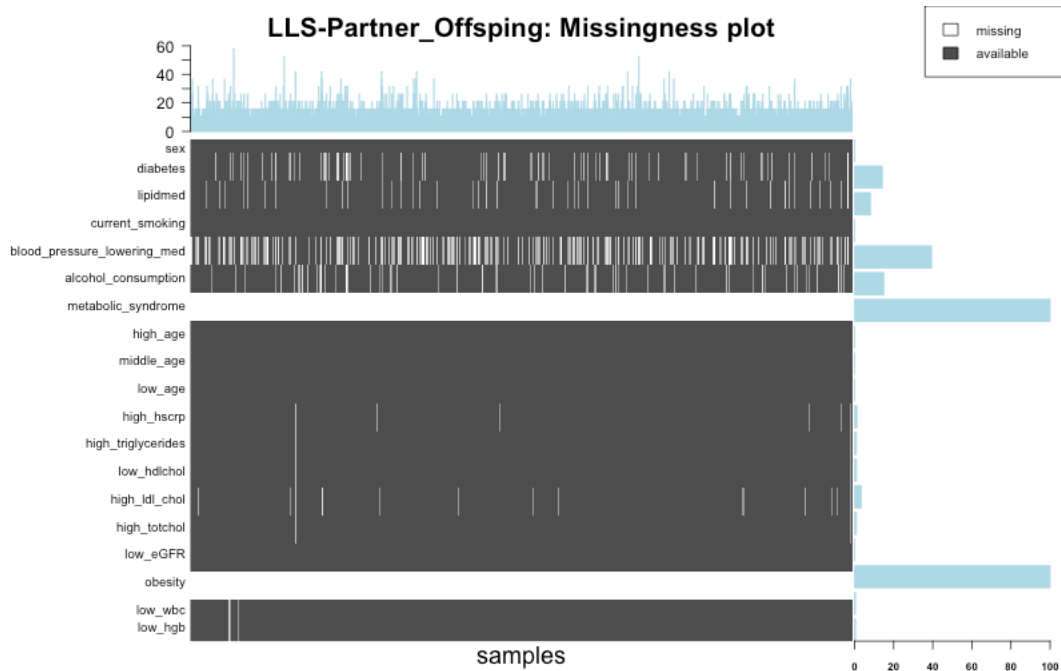
Figure S4: [A] Missing values in LLS-SIBS, [B] Missing values in LLS-PARTOFFS. The heatmaps show the status of a particular measurement (row), for a particular sample (columns). The bar plots on the sides indicate the percentage of missing measurement per clinical variable (on the right), or per sample (on the top).
