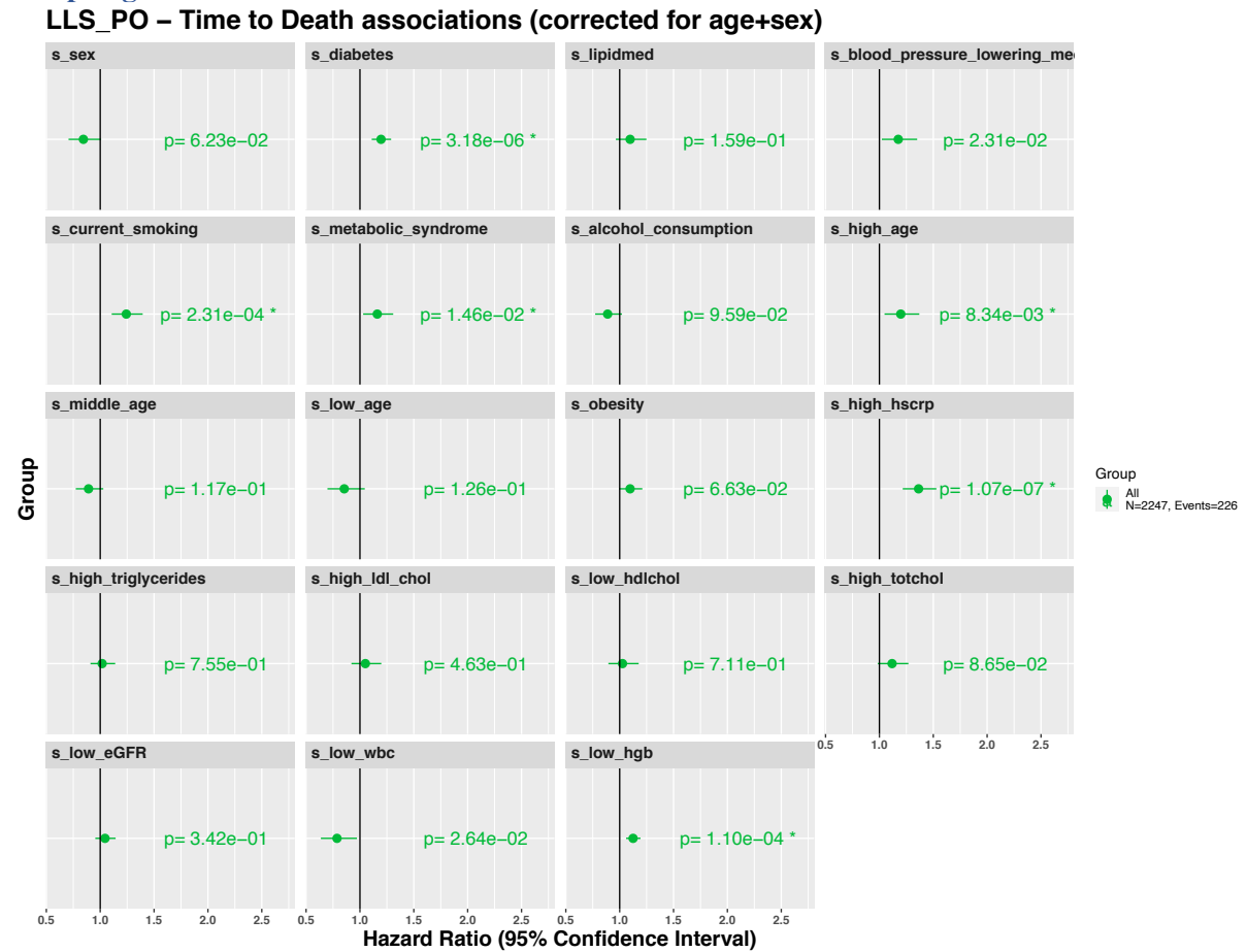
Figure S10: Associations of the surrogate metabolic with all-cause mortality in LLS Partner Offspring
