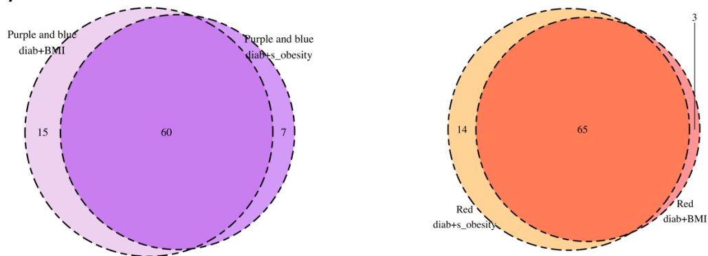
Figure S9: [A] Scree-plot of the PCA conducted in the metabolic features in LLS_PAROFFs. [B] Comparison of the coefficient estimate of 3 metaboWAS. Comparison 1: The comparison of the metaboWAS for diabetes not corrected with the metaboWAS corrected for BMI; Comparison 2: The comparison of the metaboWAS for diabetes not corrected with the metaboWAS corrected for surrogate obesity; Comparison 3: The comparison of the metaboWAS for diabetes corrected for BMI with the metaboWAS corrected for surrogate obesity. [C] On the left the Venn diagrams that shows the
