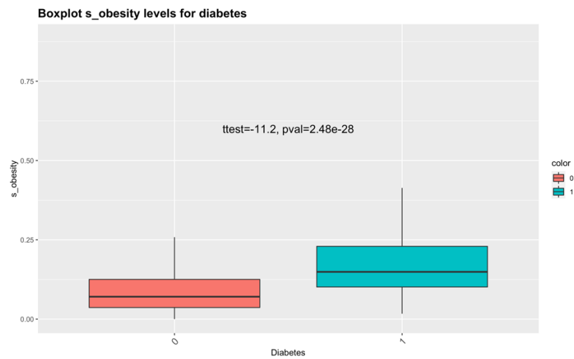
Figure S8: T-test of the association of diabetes and [A]) BMI or [B] s_obesity in LLS-PAROFF.
