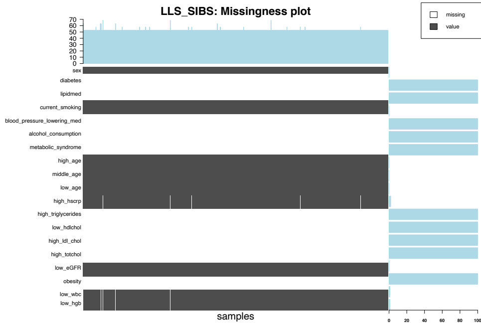
Figure S4: Missingness in LLS-SIBS and LLS_PARTOFFS
