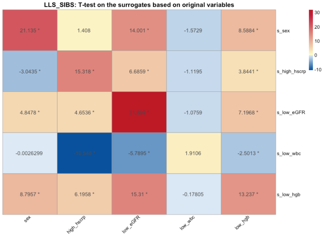
Figure S6: [A] Table reporting the results of the t -tests done on the surrogate markers to separate for each of the original variables. [B] Heatmap reporting all the t -statistics of the t -tests in Figure S5A. The numbers represent the t -statistics and there is an asterisk in case the test is significant ( p -value < 0.05).
