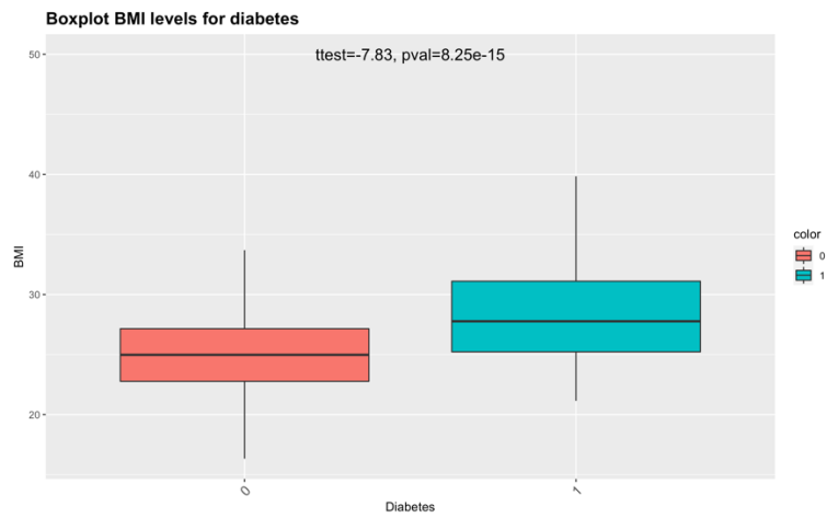
Figure S8: T-test of the association of diabetes
