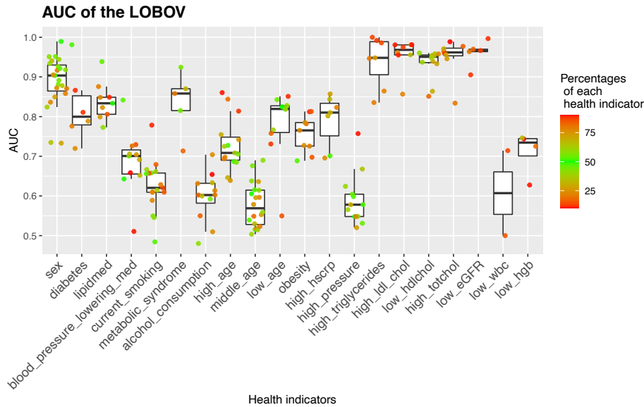
Figure S2: Leave One Biobank Out Validation
