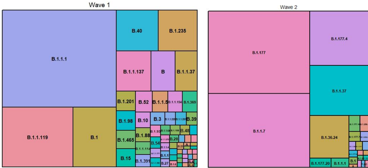
Supplementary Figure S1. Treemap of all PANGO lineages represented in the Wave 1 and Wave 2 datasets.
