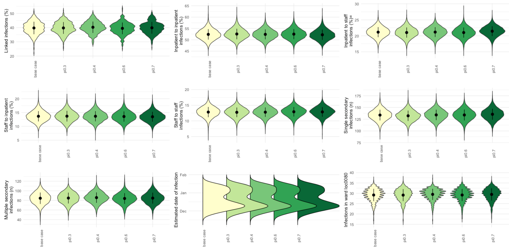
Supplementary Figure S4. Sensitivity analysis of wave 2.
