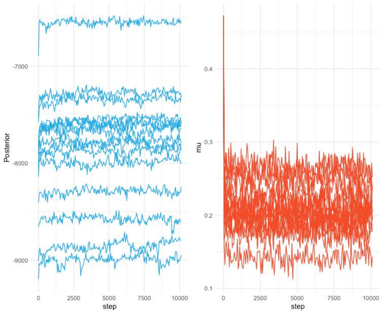
Supplementary Figure S6. Trace of the log-posterior values and \mu in exploratory runs
