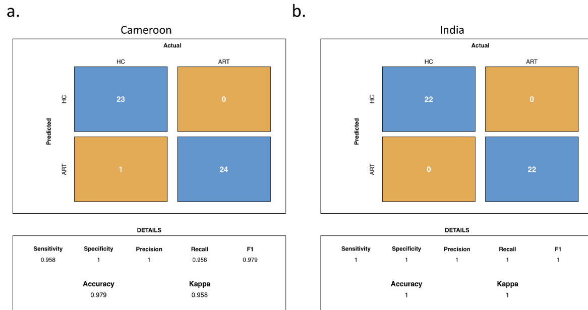
Figure S2: Confusion matrices for Cameroon (A) and India (B) random forest models.
