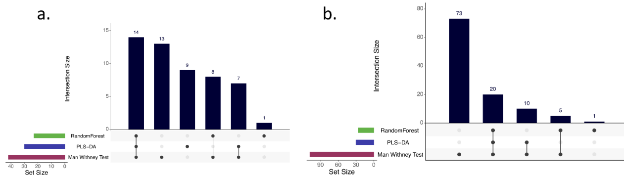
Figure S3: Upset plot of metabolites with differential abundance between HC and ART patients identified by 3 different methods in Cameroon (A) and Indian (B) cohorts. Horizontal bars show the number of metabolites found with each method. Vertical bars display intersects between methods as indicated in the matrix below the graph.
