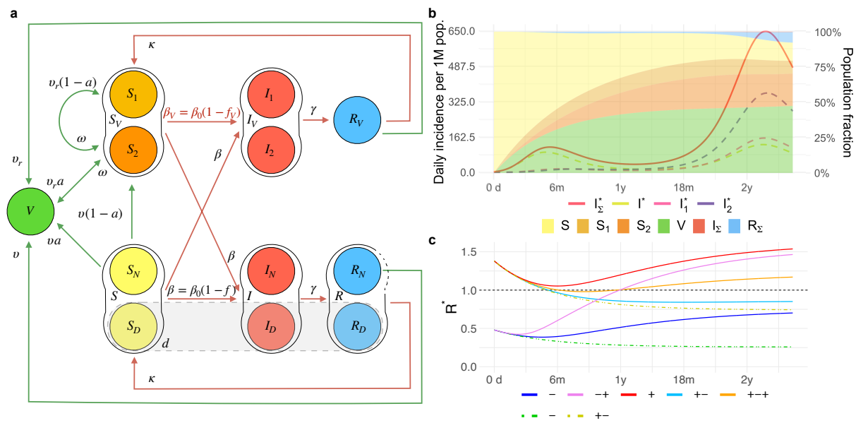
Figure 1: The VAP-SIRS model and its predicted scenarios. a . Graphical scheme of the VAP-SIRS model. b, c . Predicted scenarios for the reference setup for the Delta variant, with vaccine effectiveness a = 0.79 (corresponding to the effectiveness of the Comirnaty vaccine against infection with the Delta variant), slow (re-)vaccination rate ( v = v_r = 0.004 ; typical for many European countries), slow immunity waning \omega = 0.002 , low fraction of never-vaccinated ( d = 0.12 ; corresponding to the fraction in the United Kingdom) and proportional mixing (see Methods). b . Color curves: Timeline of daily incidence per 1 million inhabitants in different infected compartments for the combination of restrictions f = 0.77 and f_v = 0.55 . A variable with the asterisk (*) indicates that we consider a daily incidence over the corresponding variable, and by I_\Sigma^* we mean the sum of all daily infected ( I_D^* + I_N^* + I_1^* + I_2^* ). Color bands: Muller plot of the population structure (the width of the color band in the y axis) as a function of time (x axis) for the same parameter settings; by I_\Sigma and R_\Sigma we denote I + I_V and R + R_V , respectively. c . Time evolution of the instantaneous reproduction number R^* (y axis) depending on the number of days counted from the start of the vaccination program (x axis), in five different scenarios describing the epidemic evolution: overcritical (+, red, f = 0.77 and f_v = 0.38 ), subcritical (-, blue, f = 0.92 and f_v = 0.71 ), initially and eventually overcritical (+++, orange, the same restrictions as in b : f = 0.77 and f_v = 0.55 ), eventually overcritical (-+, pink, f = 0.92 and f_v = 0.38 ), and eventually subcritical (+-, cyan, with f = 0.77 and f_v = 0.71 ). As controls, two additional scenarios of the epidemic evolution are presented, corresponding to no implementation of VPs and no changes in behavior due to vaccination: subcritical (another example of - scenario, green) with f = f_v = 0.92 and eventually subcritical (another example of +- scenario, yellow) with f = f_v = 0.77 , both plotted with dot-dashed line.
