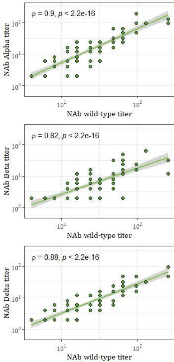
Supplementary Figure 1. Spearman correlation ( \rho ) and significance ( p ) between neutralizing antibody (NAb) titers against the wild-type virus (B.1) and variants of concern: Alpha (B.1.1.7), Beta (B.1.351) and Delta (B.1.617.2). One point may represent multiple samples ( n=78 ).
