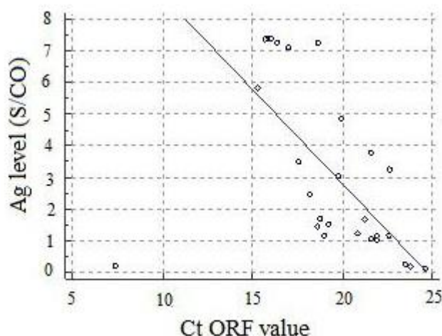
FIGURE 1: Moderate negative correlation between Ag level and Ct orf value
