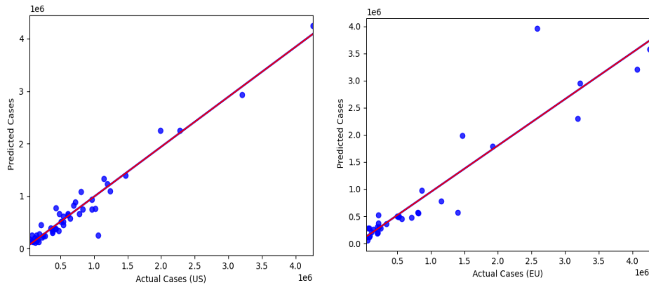
Figure 2. To the left the predictions vs observed cases for US data (Slope: 1.00 Intercept: 0 R^2 : 0.95). To the right the predictions vs observed cases for European data (Slope: 1.49 Intercept: 12K R^2 : 0.88)
