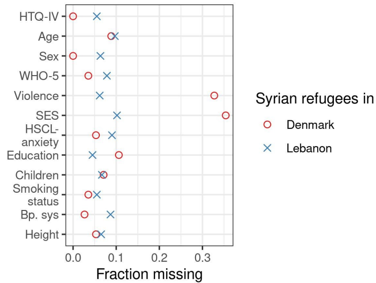
278 Figure 1: Missing fraction plot.
