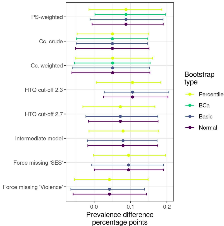
285 Figure 2: Estimate with different bootstrap confidence interval types.
