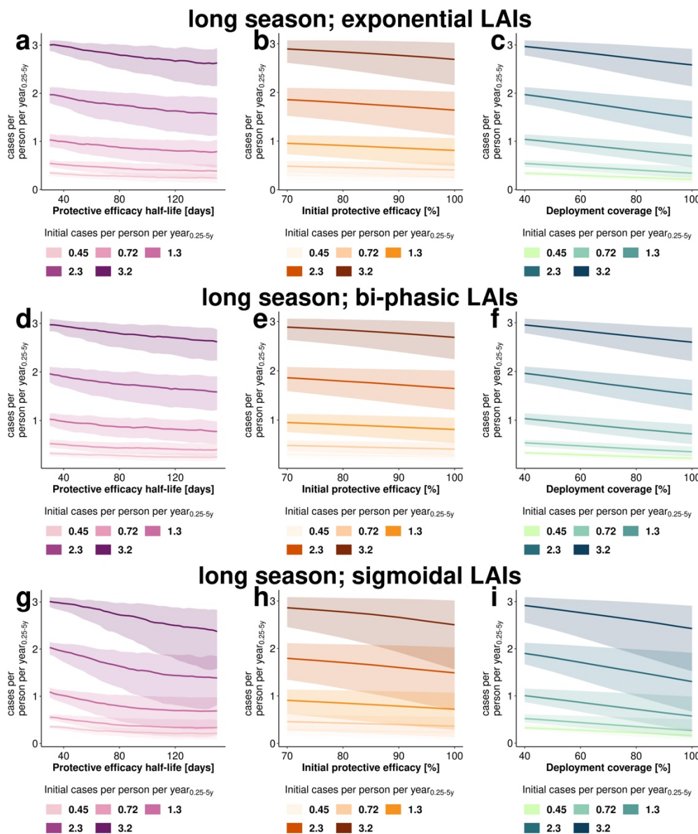
941 942 Figure S 6: Estimated impact of LAI properties and operational factors on the level of clinical 943 incidence reduction. Results are shown for the implementation stage in a setting with low access to care 944 ( E_{14}=0.1 ) and long (Mali-like) malaria transmission season, for (a-c) exponential LAIs , (d-f) bi-phasic LAIs , 945 and (g-i) sigmoidal LAIs . Changes in clinical incidence measured as cases per person per year 0.25-5y with 946 increasing tool properties or deployment coverage across the parameter space are shown for for (a, d, g) 947 half-life (30-150 d), (b, e, h) initial efficacy (80-100%) and (c, f, i) coverage (40 -100 %). The lines 948 represent the mean and the 95%- confidence bands (shaded area) capture the distribution of incidence 949 reduction across all sampled values. Increasing color intensity represents increasing initial clinical 950 incidence (cases per person per year 0.25-5y ). These results hold true for high access to healthcare settings. 951 The conversion of initial cases per person per year 0.25-5y to prevalence can be found in Table S1.
