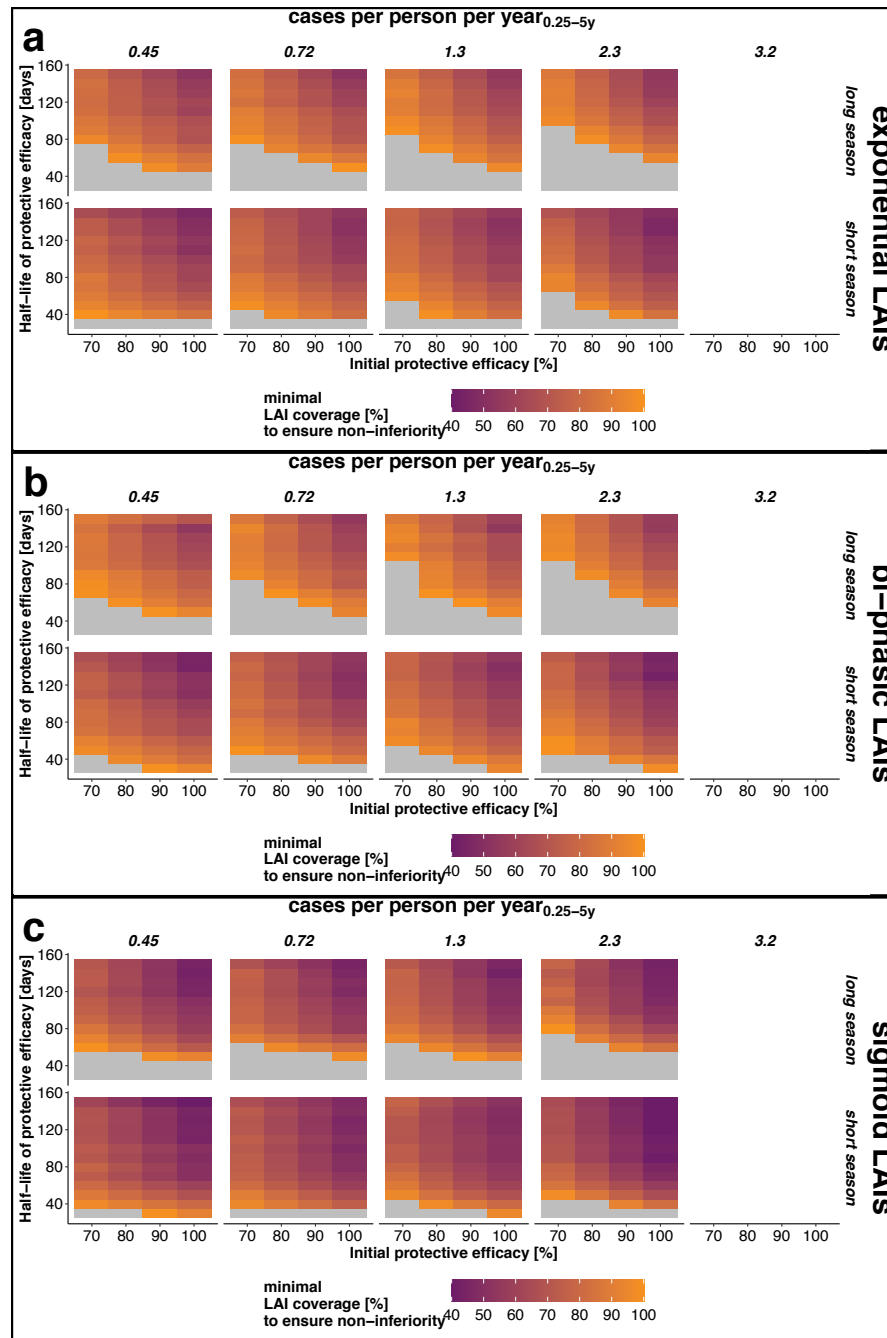
962 Figure S 8: Estimated minimal LAI coverage required during implementation stages to achieve non- 963 inferiority in a given setting. Heatmap of the estimated minimal coverage (colour) of LAIs at which non- 964 inferiority to SMC-SP+AQ (assuming a fixed SMC coverage of 60% in each of the 3 or 4 rounds) is 965 achieved for different combinations of protective efficacy decay, initial protective efficacy and protective 966 efficacy half-life. The results are displayed for intervention scenarios with a low access to care ( E_{14}=0.1 ) in 967 the two seasonal settings. In the grey area, non-inferiority could not be established for any combination of 968 tool properties. The LAI coverage could not be optimized for high transmission settings (initial cases per 969 person per year 0.25-5y =3.2) because they fail to sufficiently protect the targeted population from clinical 970 malaria even at full deployment coverage. Therefore, optimisation of the LAI deployment coverage could 971 not be conducted (Fig. S4).
