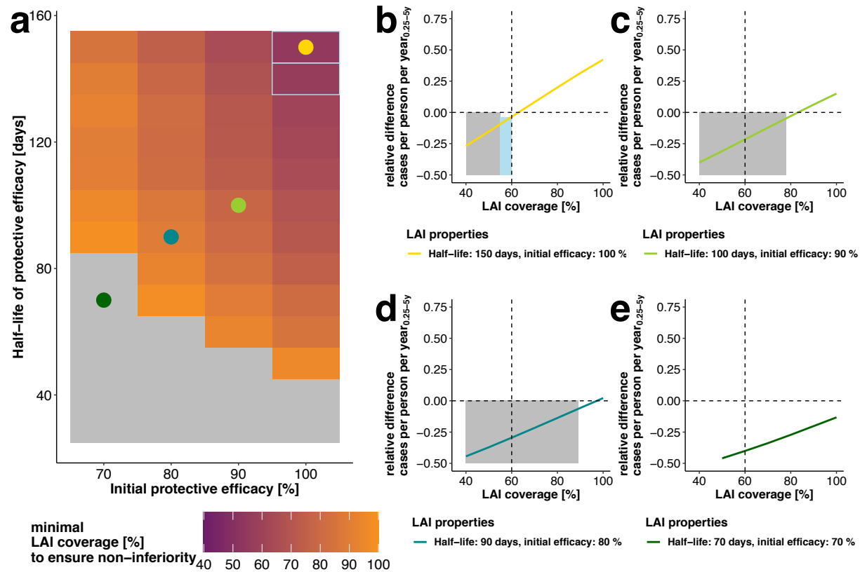
984 Figure S10: Estimated minimal LAI coverage required during implementation stages to achieve non- 985 inferiority in a given setting and predicted gains in cases averted of subsequent exponential LAI 986 coverage increments. ((a) Heatmap of the estimated minimal coverage (colour) of sigmoidal LAIs at which 987 non-inferiority to SMC-SP+AQ (assuming a fixed SMC coverage of 60%) is achieved for different 988 combinations of exponential LAI efficacy and half-life. The results are displayed for intervention scenarios 989 with an underlying disease burden of 1.4 cases per person per year 0.25-5y , long malaria transmission season 990 and low access to treatment ( E_{14}=0.1 ). In the grey area, non-inferiority could not be established for any 991 coverage. For the tool characteristics within the light-blue frames, non-inferiority could be reached with a 992 LAI coverage under the reference SMC-SP+AQ coverage of 60%. The coloured dots represent four 993 illustrative LAI profiles of (b) 150 days half-life and 100% initial efficacy (yellow), (c) 100 days half-life 994 and 90% initial efficacy (light green), (d) 90 days half-life and 80% initial efficacy (blue), and (e) 70 days 995 half-life and 70% initial efficacy (dark green, e). (b-e). Corresponding predicted relative differences in 996 cases per person per year 0.25-5y (Eq. 5) are calculated for the illustrative LAIs (coloured dots) in (a) in the 997 last implementation year (5 years after LAI introduction) over all LAI coverages as compared to SMC- 998 SP+AQ at 60% coverage (vertical dotted line). The predicted positive increase in relative difference in 999 yearly clinical cases (above the dotted horizontal line) means more clinical cases are averted with LAIs 1000 than with SMC-SP+AQ. It thus illustrates the benefit of increasing exponential LAI-coverage above the 1001 minimal required coverage to achieve non-inferiority (shown by the grey coloured area). In the light-blue 1002 area in (b), a LAI coverage lower than the SMC-SP+AQ coverage is sufficient to establish non-inferiority.
