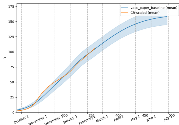
Figure 8: Calibration of Model M. The y -axis shows the model-predicted cumulative number of COVID-19-related deaths in simulation (blue, mean \pm one standard deviation) compared to the real situation in the Czech Republic scaled to the model population size (orange).
