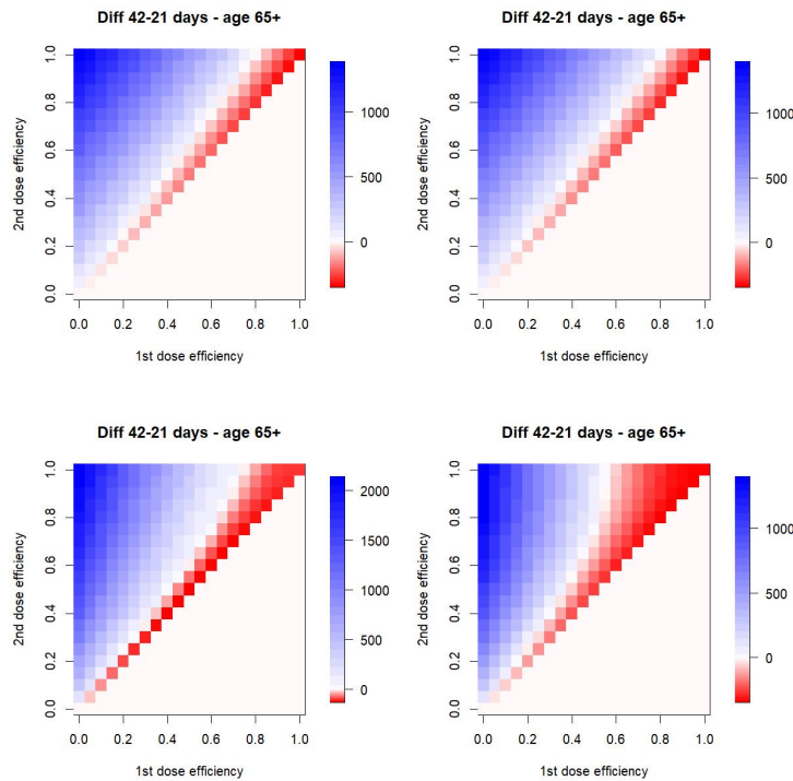
Figure 3: Efficacy of delaying the second vaccine dose by three weeks from 21 to 42 days, assuming vaccine effect on the probability that a symptomatic individual becomes hospitalized (top left), the probability that a hospitalized individual needs an ICU (top right), the probability of dying when on the ICU (bottom left), and combination of effects on the probability of needing an ICU and probability to die when on ICU (bottom right). Only model H is used here.
