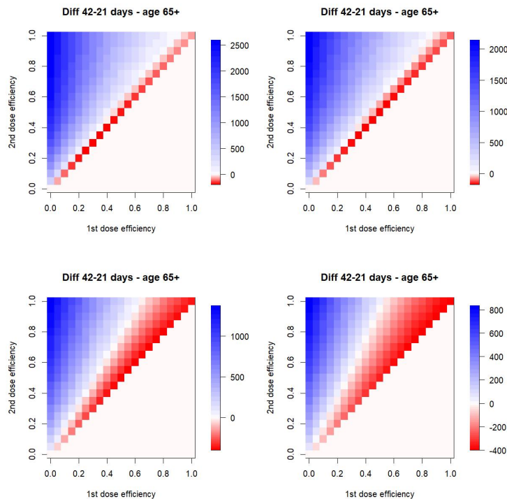
Figure 5: Efficacy of delaying the second vaccine dose by three weeks from 21 to 42 days, assuming leaky vaccine effect on the probability that a vaccinated person gets infected by contact with an infectious one, and at the same time on the probability that a vaccinated person becomes symptomatic when infected. Top left: twice more doses available, top right: actual state in Czechia, bottom left: twice less doses available, bottom right: four time less doses available. Only model H used here.
