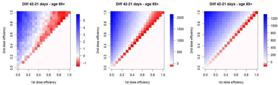
Figure 2: Efficacy of delaying the second vaccine dose by three weeks from 21 to 42 days, for all-or-nothing vaccine effect on the probability of infection transmission. Left column: model M, middle column: model H, right column: model F.
