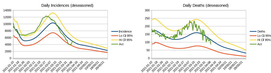
Figure 9: Model F calibration. Left panel: daily detected incidences of COVID-19. Right panel: daily deaths due to COVID-19. Legend: blue line is the mean prediction, while the yellow and red lines delimit the 95% confidence interval. Green curve represents real data.
