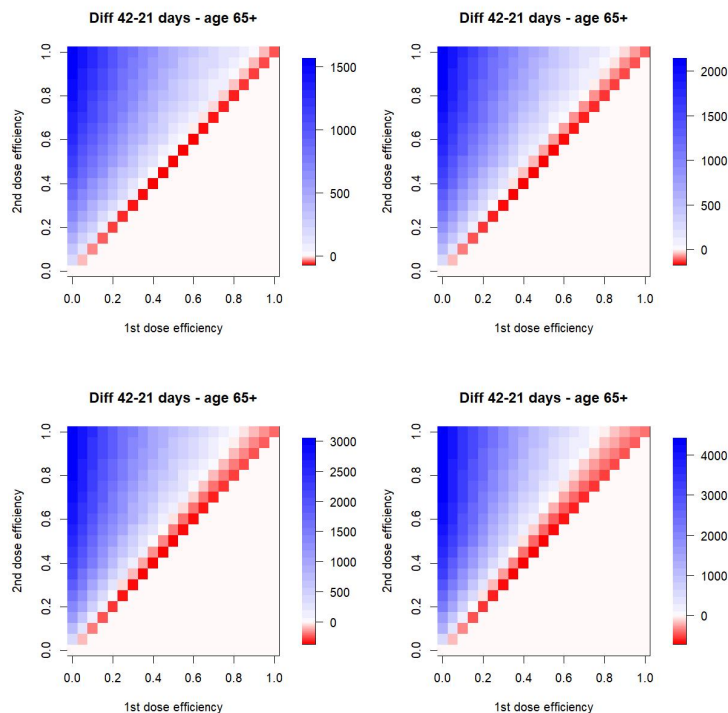
Figure 4: Efficacy of delaying the second vaccine dose by three weeks from 21 to 42 days, assuming leaky vaccine effect on the probability that a vaccinated person gets infected by contact with an infectious one, and at the same time on the probability that a vaccinated person becomes symptomatic when infected. Top left: contacts at 35% of the pre-pandemic state, top right: contacts at 45% (real situation in Czechia), bottom left: contacts at 55%, bottom right: contacts at 65%. Only model H is used here.
