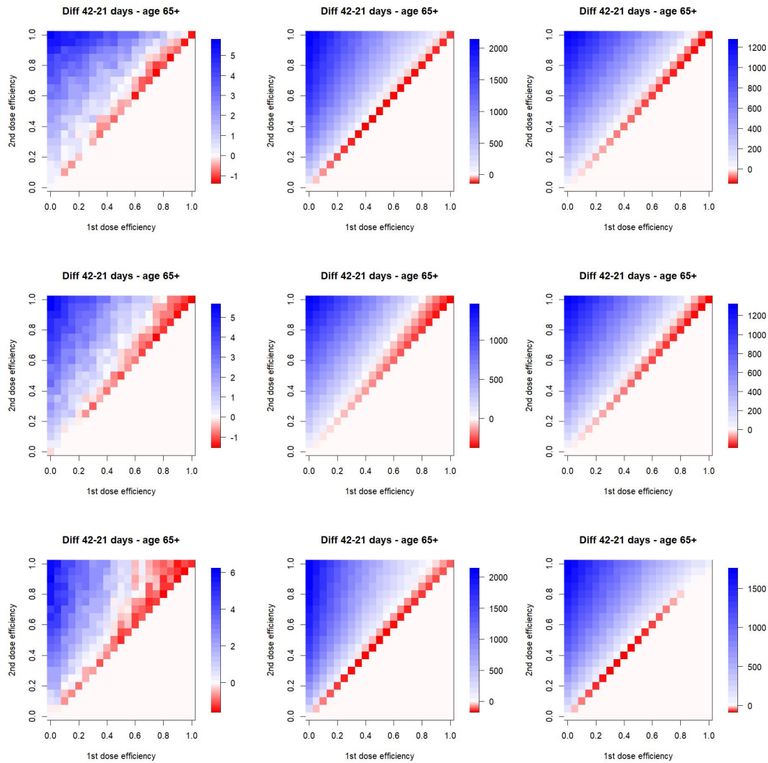
Figure 1: Efficacy of delaying the second vaccine dose by three weeks from 21 to 42 days, for different modes of vaccine action and different adopted epidemiological models. Top row: leaky vaccine effect on the probability of infection transmission, second row: vaccine effect on the probability of becoming symptomatic when infected, bottom row: combination of leaky transmission and probability of becoming symptomatic. Left column: model M, middle column: model H, right column: model F.
