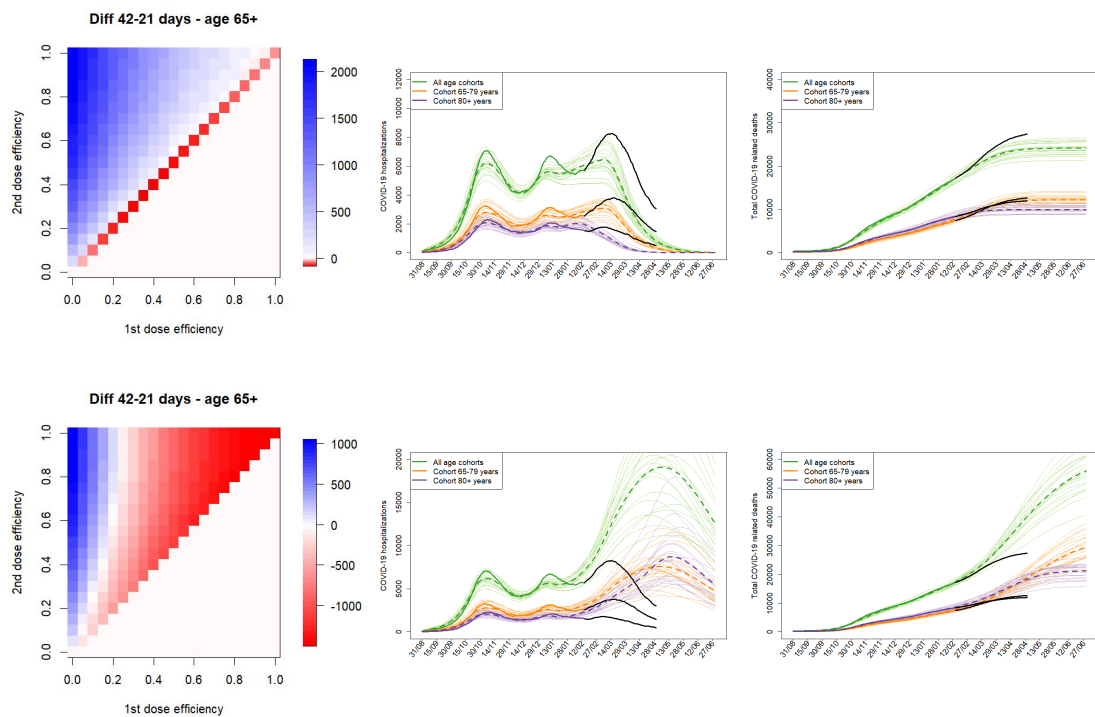
Figure 6: The extreme scenario. Efficacy of delaying the second vaccine dose by three weeks from 21 to 42 days, assuming (top row) vaccine effect on infection transmission and the probability that an infected person shows symptoms, contacts at 35% of pre-pandemic state and twice more doses available, and (bottom row) vaccine effect on the probabilities of needing an ICU and dying when on the ICU, contacts at 65% and four times less doses available. Each of these extreme scenarios is moreover supplemented by the course of the numbers of hospitalized and dead individuals (legend as in Fig. 7 in Methods). Only model H is used here, with 70% and 90% efficacy of the first and second dose, respectively.
