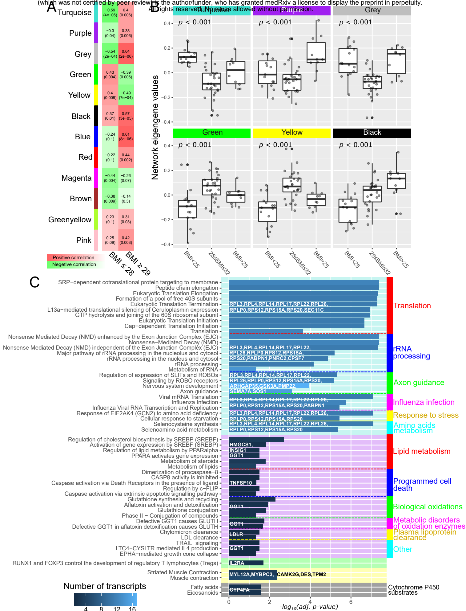
Figure 5 – (A) Correlations between transcript networks' eigengene values and BMI. Values in brackets are false discovery rate adjusted p-values. (B) Boxplots of networks' eigengene values in the BMI groups with one-way ANOVA p-values. (C) Reactome pathway enrichments with network-specific genes. Color intensity of the bars indicate number of genes from each network that enriched particular pathways. The length of the bars indicates -\log_{10}(p\text{-value}) . Only pathways with false discovery rate adjusted p-values less than 0.05 are shown.
