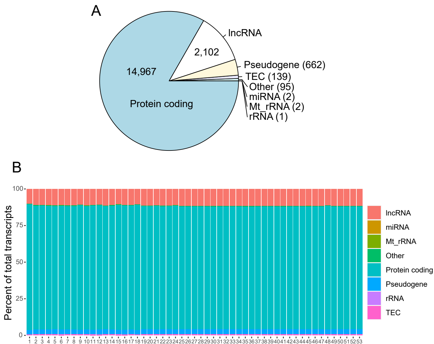
Figure 2 – (A) Summary of transcript biotypes in the whole transcriptomics dataset. (B) Biotypes percentage by sample
