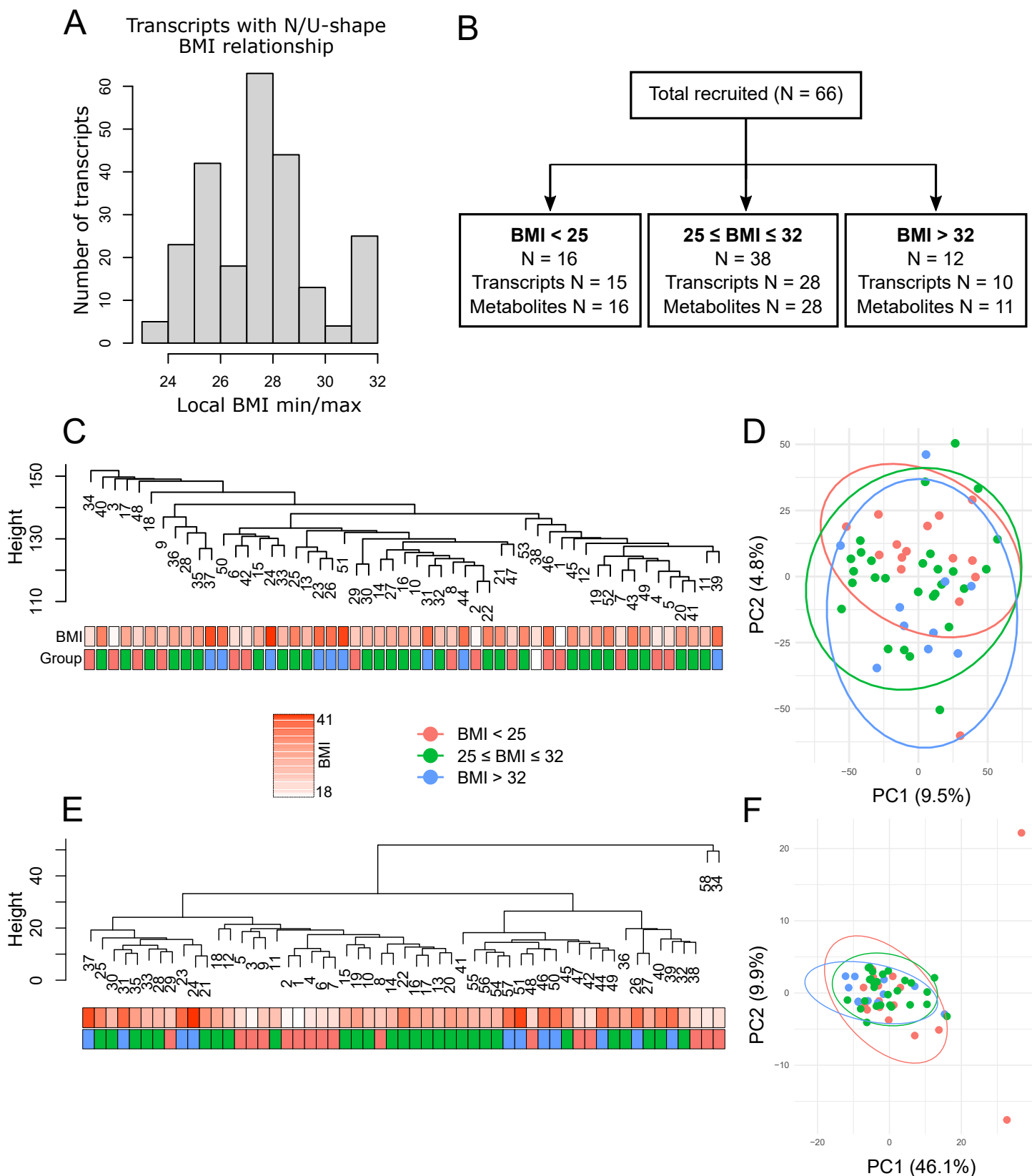
Figure 3 – (A) Distribution of local BMI minima and maxima for transcripts whose expression display U or N-shape BMI dependence. (B) BMI groups definition with numbers of samples. (C) Hierarchical clustering of samples using transcriptomics data. (D) Principal component analysis of transcriptomics data: the first two components were plotted with 95% confidence interval for each BMI group. (E) Hierarchical clustering of samples using metabolomics data. (F) Principal component analysis of metabolomics data: the first two components were plotted with 95% confidence intervals for each BMI group.
