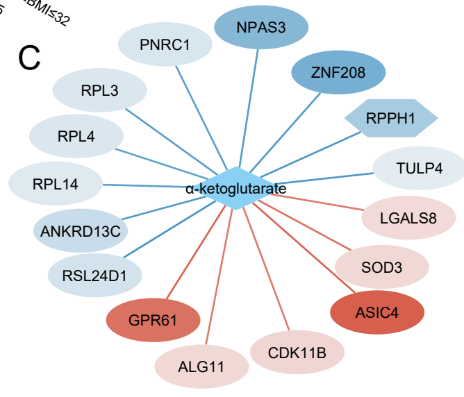
Figure 4 – (A) Significant pathways plotted as a heatmap. Green and blue color show pathways related to translation and RNA processing. Magenta indicates amino acids metabolism pathways that include -ketoglutarate. (B) Highly variable transcripts between the BMI groups with the membership in significant pathways and showing biphasic BMI relationship are plotted against BMI. \alpha -ketoglutarate that is significantly different between the 25 \geq \text{BMI} \leq 32 and \text{BMI} < 25 groups was also plotted. The red line and number indicate local minimum or maximum; p_1 and p_2 specify regression p-values before and after the local minimum/maximum. (C) \alpha -ketoglutarate – transcripts similarity network. The colour of edges indicates the interaction weight and node colour indicates log fold change in the 25 \geq \text{BMI} \leq 32 vs \text{BMI} < 25 comparison. Node shape indicates transcripts' biotype.
