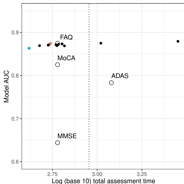
Fig. 5. Wide range of (estimated) total assessment times of accuracy-time optimised feature sets. Vertical axis: AUC values based on 3-class RF classifier. Horizontal axis: Logarithmic scale of (estimated) total assessment time. AUCs of accuracy-time optimised sets (filled circles) higher than ADAS, MMSE and MoCA complete standardised assessments while on par with FAQ complete assessment (black opened circles). Blue and orange filled circles: Optimal item sets with the shortest total assessment and highest AUC with total assessment time under 15 minutes (vertical dotted line), respectively (see Tables I and II for details on their specific items).
