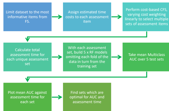
Fig. 2. Analytical pipeline for optimising accuracy-time dementia assessment items.
