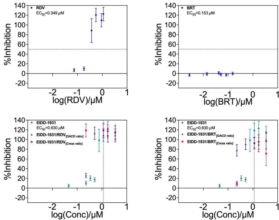
Fig. S4. Dose-response curves for EIDD-1931, remdesivir (RDV), and baricitinib (BRT) in monotherapies and in combinations against SARS-CoV-2 B.1.351 variant. Increasing concentrations of EIDD-1931, RDV, and BRT monotherapies were added to Vero E6 cells infected with SARS-CoV-2 B.1.351 variant at 100 TCID 50 and incubated for 72 h. Additionally, EIDD-1931/RDV and EIDD-1931/BRT combinations at the OACD and C max ratios (purple and pink markers, respectively) were also added to the infected Vero E6 cells and incubated for 72 h. The %Inhibition resulted from the mono- and combination therapies were measured via the luminescence signals of the cell viability in the ATP activity assay. The y-axis of each curve represent the %Inhibition for the each drug and combination. The EC 50 values for monotherapies are also summarized in the legends. Vertical dotted lines represent the 10% C max of EIDD-1931, and the horizontal dotted lines represent the EC 50 for monotherapies. No data points were excluded in dose-response curve analysis. Data points are presented as mean ± propagated SD (N = 3).
