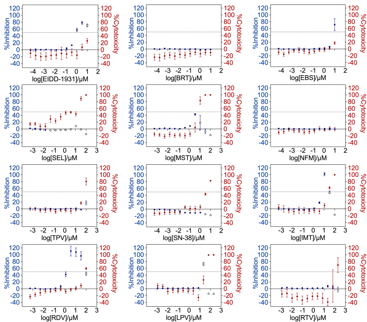
Fig. S1. Dose-response curves for all 12 selected drugs given as monotherapies. Vero E6 cells infected with SARS-CoV-2 at 100 TCID 50 were treated with each drug at different concentrations for 72 h. The viral infection %Inhibition and %Cytotoxicity resulted from these drug treatments in the Vero E6 cells were determined by measuring the luminescence signals of the cell viability in the ATP activity assay. The left and right y-axis represent the %Inhibition (blue) and %Cytotoxicity (red) of the drugs, respectively. The unfilled circles (blue) in the dose-response curves were %Inhibition data points with corresponding toxicities above 25% and were excluded from subsequent dose-response curve analysis. Dotted lines represent absolute EC 50 and CC 50 , respectively. Data points are mean ± propagated SD (N = 3). Baricitinib (BRT), ebselen (EBS), selinexor (SEL), masitinib (MST), nafamostat mesylate (NFM), telaprevir (VX-950) (TPV), imatinib mesylate (IMT), remdesivir (RDV), lopinavir (LPV), and ritonavir (RTV).
