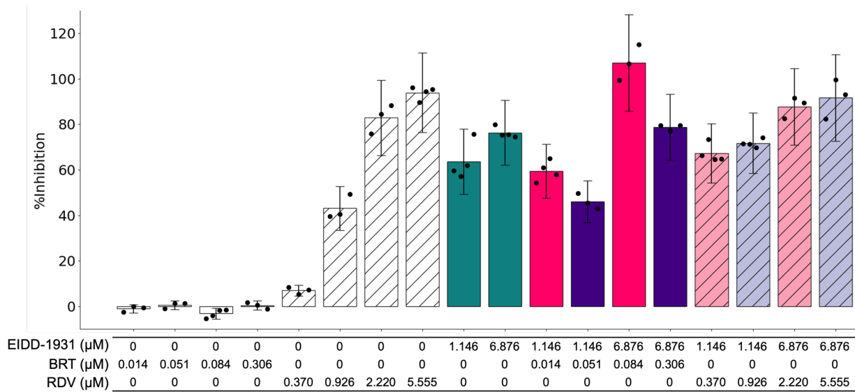
Fig. S3. Validation of EIDD-1931 interactions at 10% and 60% C_{max} with remdesivir (RDV), and baricitinib (BRT). EIDD-1931 (green), BRT (white), RDV (white, patterned) and EIDD-1931 combinations at the C_{max} ratio (pink) and at the OACD ratio (purple) at different concentrations were added to Vero E6 cells infected with SARS-CoV-2 at 100 TCID 50 and incubated for 72 h. The %Inhibition resulted from the treatments were measured via the luminescence signals of the cell viability in the ATP activity assay. Data points are presented as mean \pm propagated SD (N = 3 to 4). Of note, this propagated SD did not arise from the replicates, but from plate-to-plate variation from control SD. Black, round markers indicate individual replicates. No statistically significant difference was detected with Kruskal-Wallis test when followed by Dunn's post hoc test.
