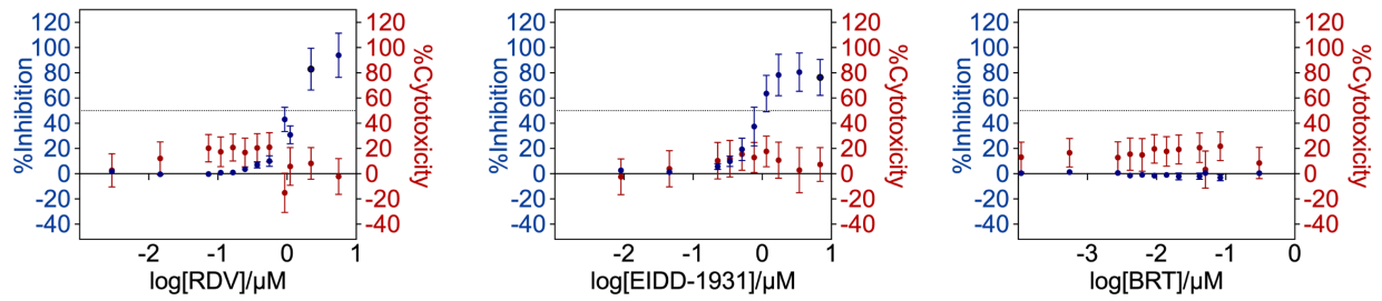
Fig. S2. Validation dose-response analysis for remdesivir (RDV), EIDD-1931, and baricitinib (BRT). RDV, EIDD-1931, and BRT at different concentrations were added to Vero E6 cells infected with SARS-CoV-2 at 100 TCID 50 and incubated for 72 h. The %Inhibition and %Cytotoxicity resulted from the treatments were measured via the luminescence signals of the cell viability in the ATP activity assay. The left and right y-axis of each curve represent the %Inhibition (blue) and %Cytotoxicity (red) for the drugs, respectively. Dotted lines represent absolute EC 50 and CC 50 , respectively. No data points were excluded in dose-response curve analysis. Data points are presented as mean ± propagated SD (N = 3 to 4).
