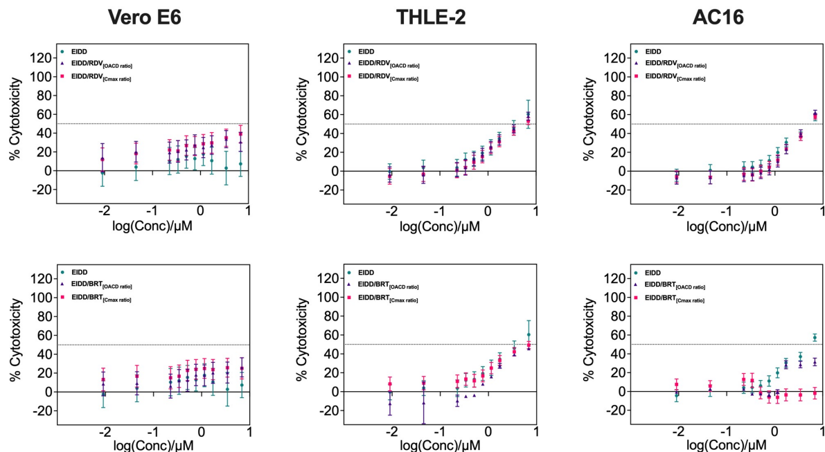
Fig. S5. %Cytotoxicity data for EIDD-1931/RDV and EIDD-1931/BRT in Vero E6, THLE-2, and AC16 cell lines. %Cytotoxicity for Vero E6 was determined after 72 h of treatment with EIDD-1931/RDV and EIDD-1931/BRT combinations at increasing concentrations using luminescence-based ATP activity assay. %Cytotoxicity data (mean \pm propagated SD, N=3 to 4) for EIDD-1931/RDV and EIDD-1931/BRT at two different ratios: OACD ratio (Level 2/Level 2 ratio for EIDD-1931/RDV and Level 1/Level 2 ratio for EIDD-1931/BRT from the IDentif.AI experimental set; purple triangles) and C_{max} ratio ( C_{max}/C_{max} ; pink squares) of the two drugs in the combination. Additionally, %Cytotoxicity was measured in THLE-2 human liver cell lines and AC16 human cardiomyocyte. EIDD-1931/RDV and EIDD-1931/BRT were added to the cells for 72 h before measuring the cell viability via luminescence-based ATP activity assay. Remdesivir (RDV), and baricitinib (BRT).
