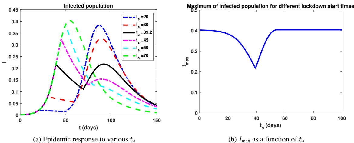
Figure 2: Response of infected population to a single lockdown as characterized by (4). The following parameters were utilized in the above simulation: \beta = 0.2, p = 0.2252, \nu = 0.05, I_0 = 10^{-4} , and S_0 = 1 - I_0 . Note that according to (7), \mathcal{R}_0 = 4 prior to lockdown, while \mathcal{R}_0 \approx 0.9 during the lockdown. We observe a global minimum of I_{\max} at t_s \approx 39.2 days, which corresponds to the black curve in Figure 2a. Note that both relative maxima appear to be equal for this minimizing t_s .
