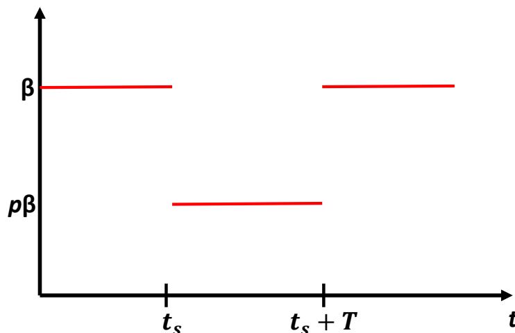
Figure 1: Visualization of idealized lockdown (4). We assume that transmission is reduced by an effective amount p during the lockdown, where 0 < p < 1 . The lockdown is initiated at t_s and is enacted for T units of time.
