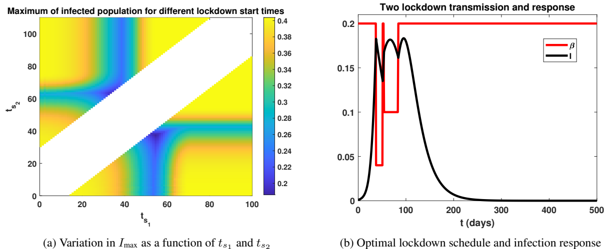
Figure 4: Numerical investigation of optimal lockdown schedule of the form (17) with n = 2 . Parameters utilized are \beta = 0.2, p_1 = 0.5, p_2 = 0.2, T_1 = 30, T_2 = 14, \nu = 0.05, I_0 = 10^{-4} , and S_0 = 1 - I_0 . As in Figure 2, our goal is to minimize the peak of the infected population, which corresponds to bluer shades in Figure 4a. The white region is prohibited, as it would correspond to overlapping lockdowns. The optimal initiation times t_{s_1} \approx 54.1 days and t_{s_2} \approx 37.4 days is provided in Figure 4b. Note that the response I exhibits 3 = n + 1 relative maxima (peaks) of equal size.
