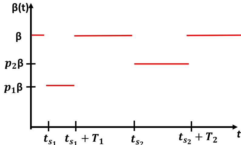
Figure 3: Visualization of n = 2 lockdowns (17). We assume that transmission is reduced by an effective amount p_1 during [t_{s_1}, t_{s_1} + T_1] and p_2 during [t_{s_2}, t_{s_2} + T_2] , where 0 < p_1, p_2 < 1 .
