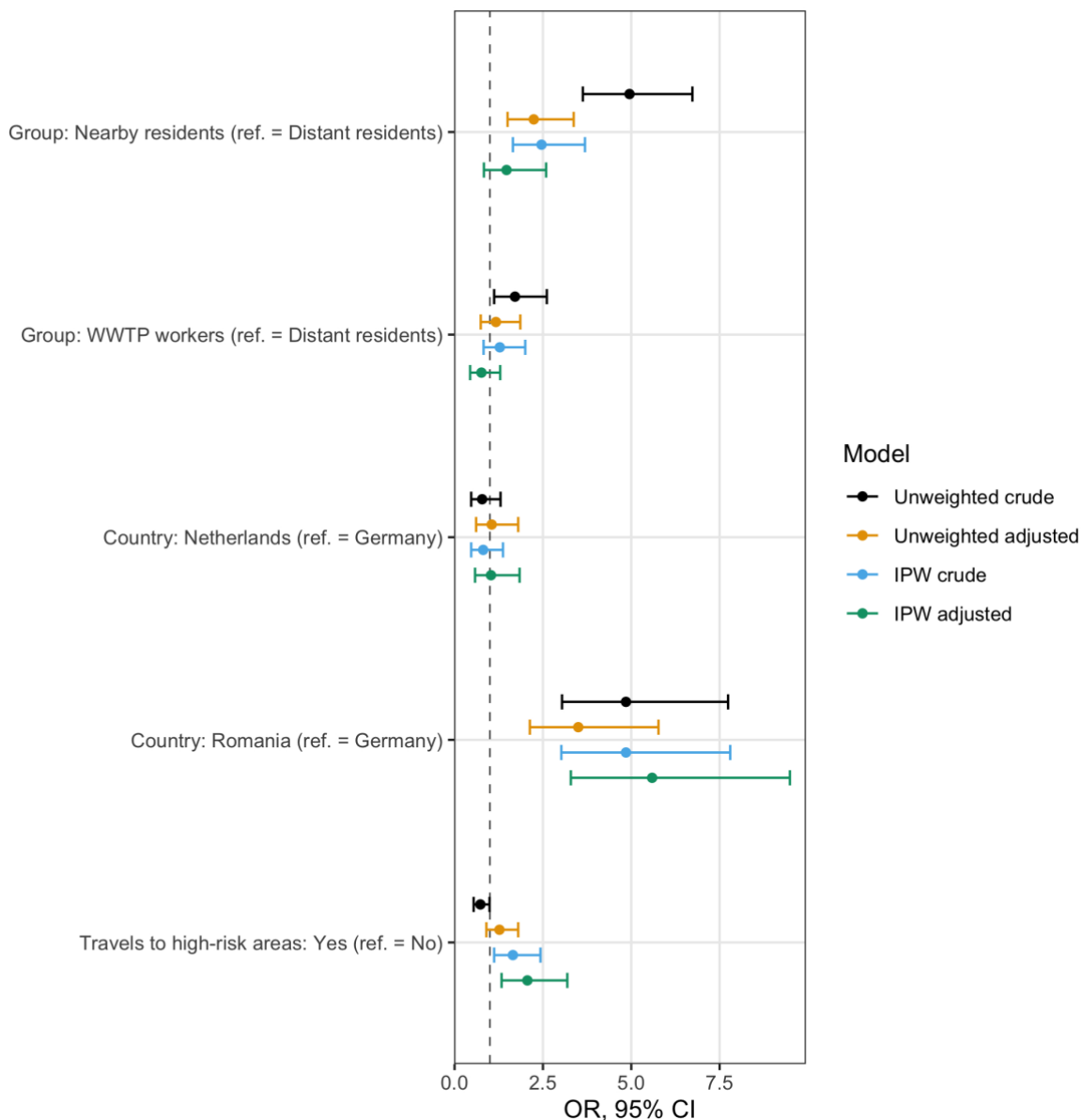
Fig. 3: Comparison of models estimating the effect of participation group (wastewater treatment plant - WWTP- worker, nearby resident, distant resident) as a proxy for exposure routes (ingestion of droplets, hand-to-mouth contact, or inhalation of aerosols) in and around the local WWTP on the presence of ESBL-producing E. coli in stool samples, AWARE Study, 2021.
