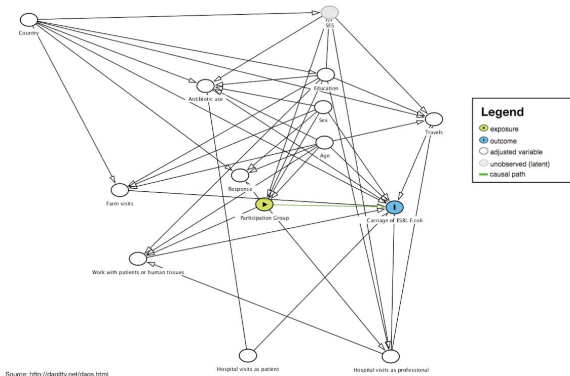
Fig. 2: Directed Acyclic Graph (DAG) for the direct effect of participation group (wastewater treatment plant -WWTP- worker, nearby resident, distant resident) as a proxy for exposure routes (ingestion of droplets, hand-to-mouth contact, or inhalation of aerosols) in and around the local WWTP on the presence of ESBL-producing E. coli in stool samples, AWARE Study, 2021
