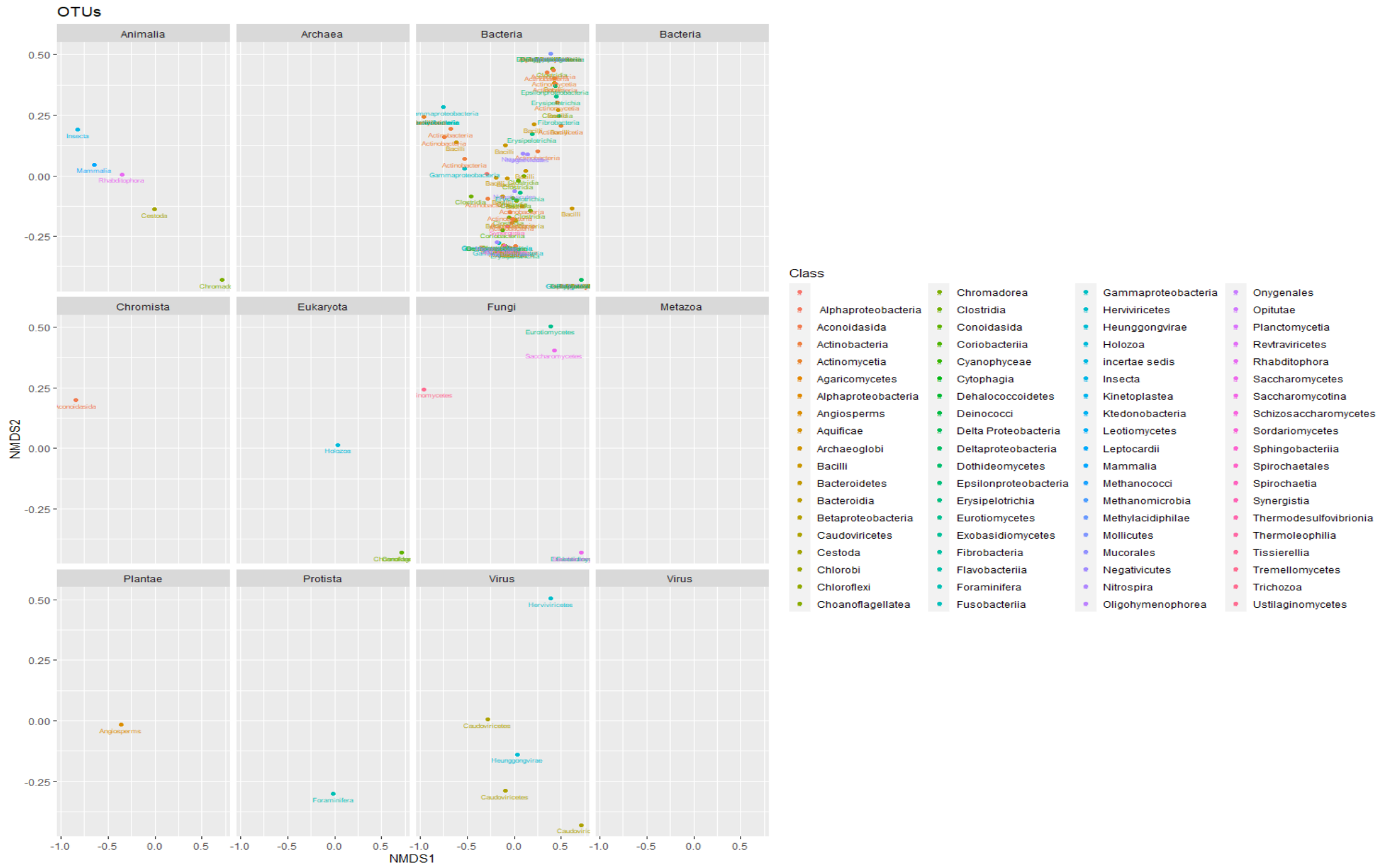
Figure vi. NMDS ordination plot of day 7 samples from patients. The bacterial classes were virtually the same in terms of their distance from each other compared to that of day 2 whilst the distances between classes of other Kingdoms were virtually the same, showing the little effect of antibiotics on other Kingdoms except on bacteria.
