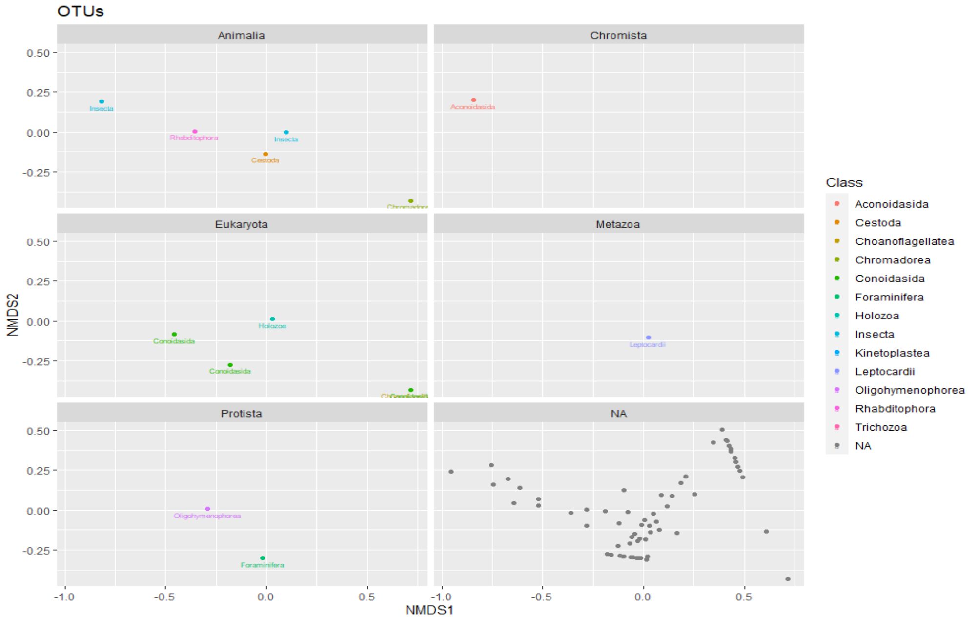
Figure viii. NMDS ordination plot of parasites. The classes of parasites were distant from each other on the plots, with Eukaryota and Animalia Divisions having more member.
