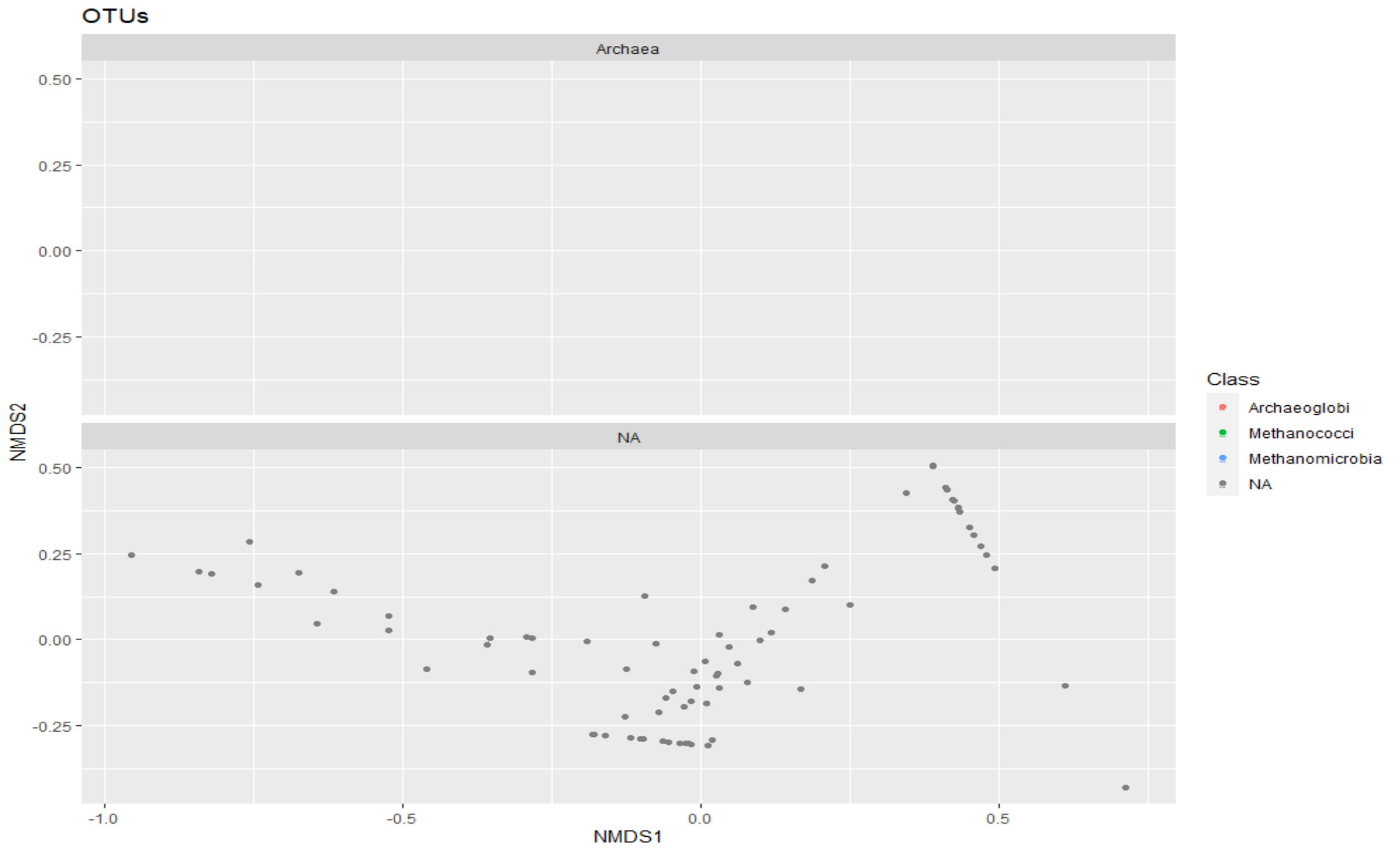
Figure i. Ordination plots (non-metric multidimensional scaling, NMDS) of Archaea.
