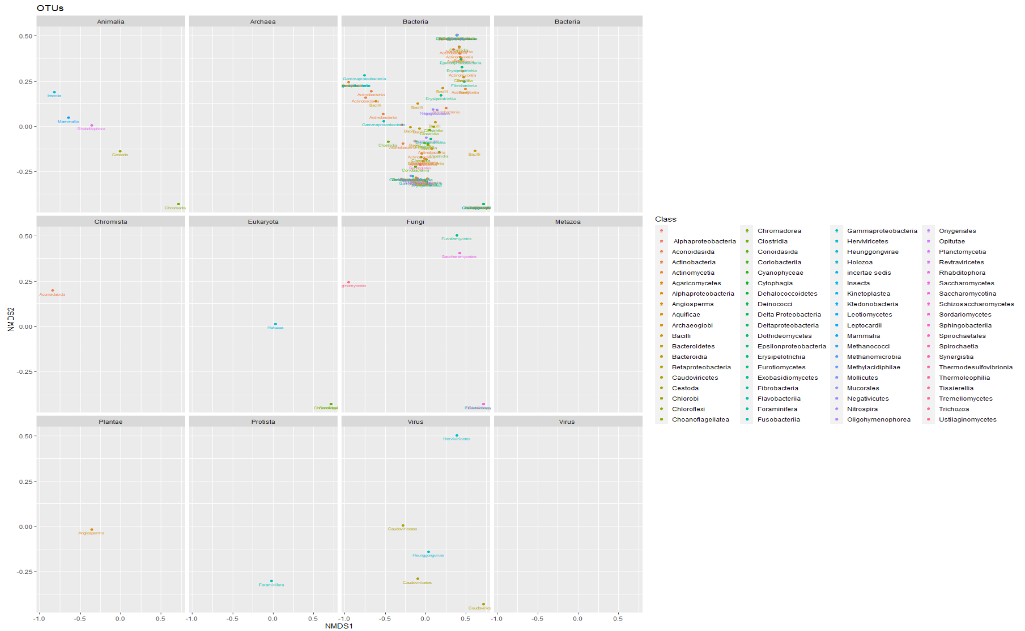
Figure v. NMDS ordination plot of day 2 samples from patients. Whilst the bacterial classes spaced out from each other, there were hardly any obvious change in the classes of other Kingdoms/Divisions. This suggests a change in the bacterial diversity during antibiotic therapy and lack of substantial antibiotic effect on the other Kingdoms.
