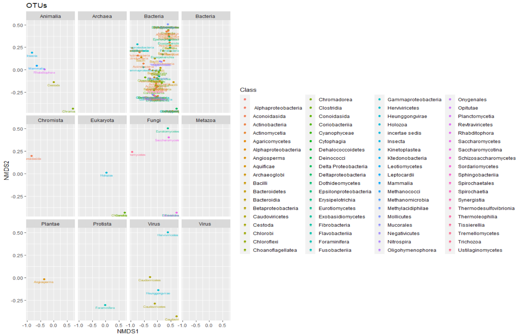
Figure iv. NMDS ordination plots for day 1 samples. The greatest change in ordination was seen in bacterial classes compared to the baseline ordination plots. The day 1 ordination was closer to each other than the baseline plots. Virtually no change was observed between the classes of other Kingdoms in day 1 and baseline.
