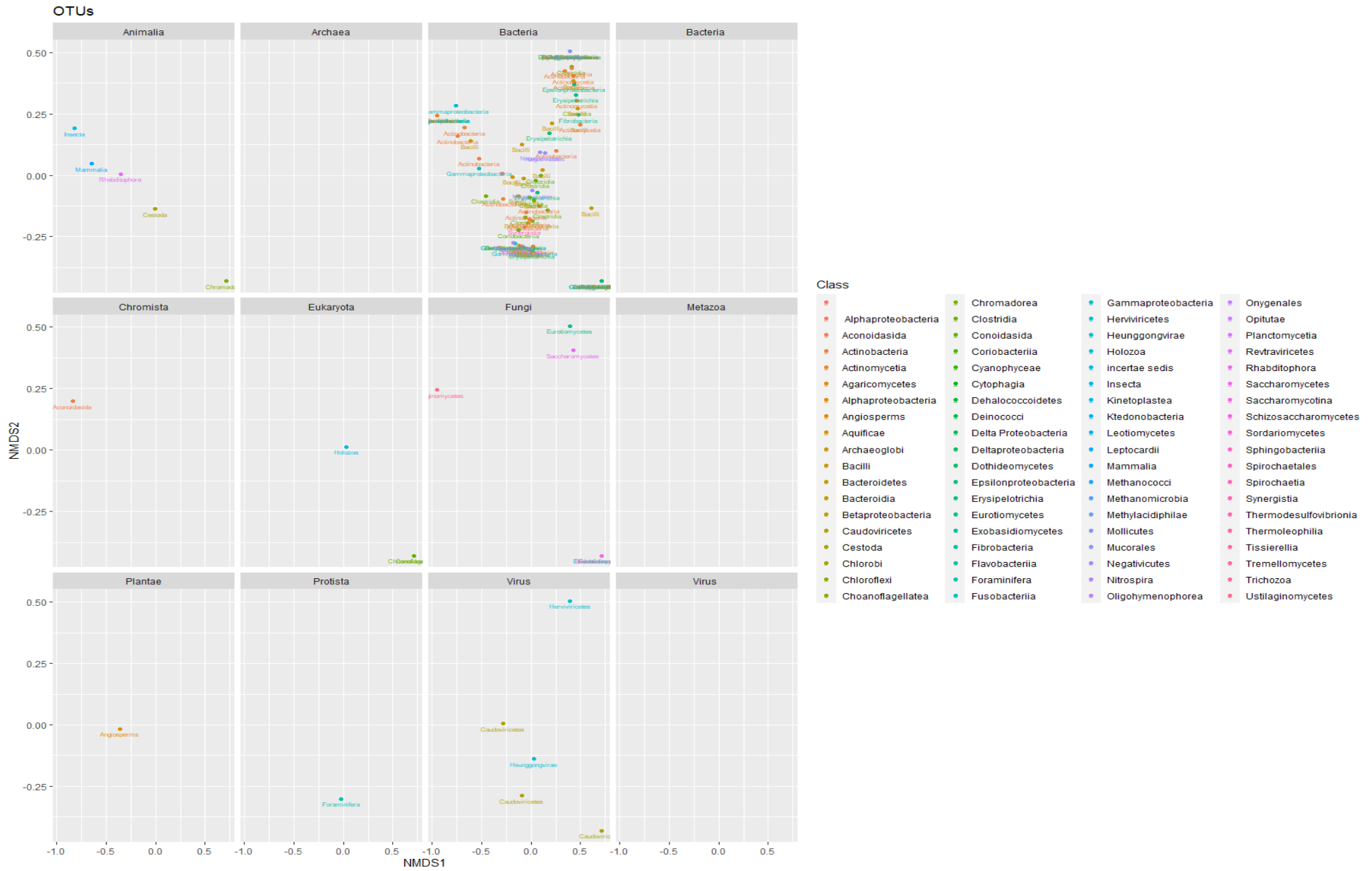
Figure iii. NMDS ordination plots for baseline samples. The NMDS ordination plots of the various classes from baseline samples. Bacterial classes were closely knit together, whilst classes of other Kingdoms (Plantae, Protista, Virus, Fungi, Eukaryota, Animalia) were separated from each other.
