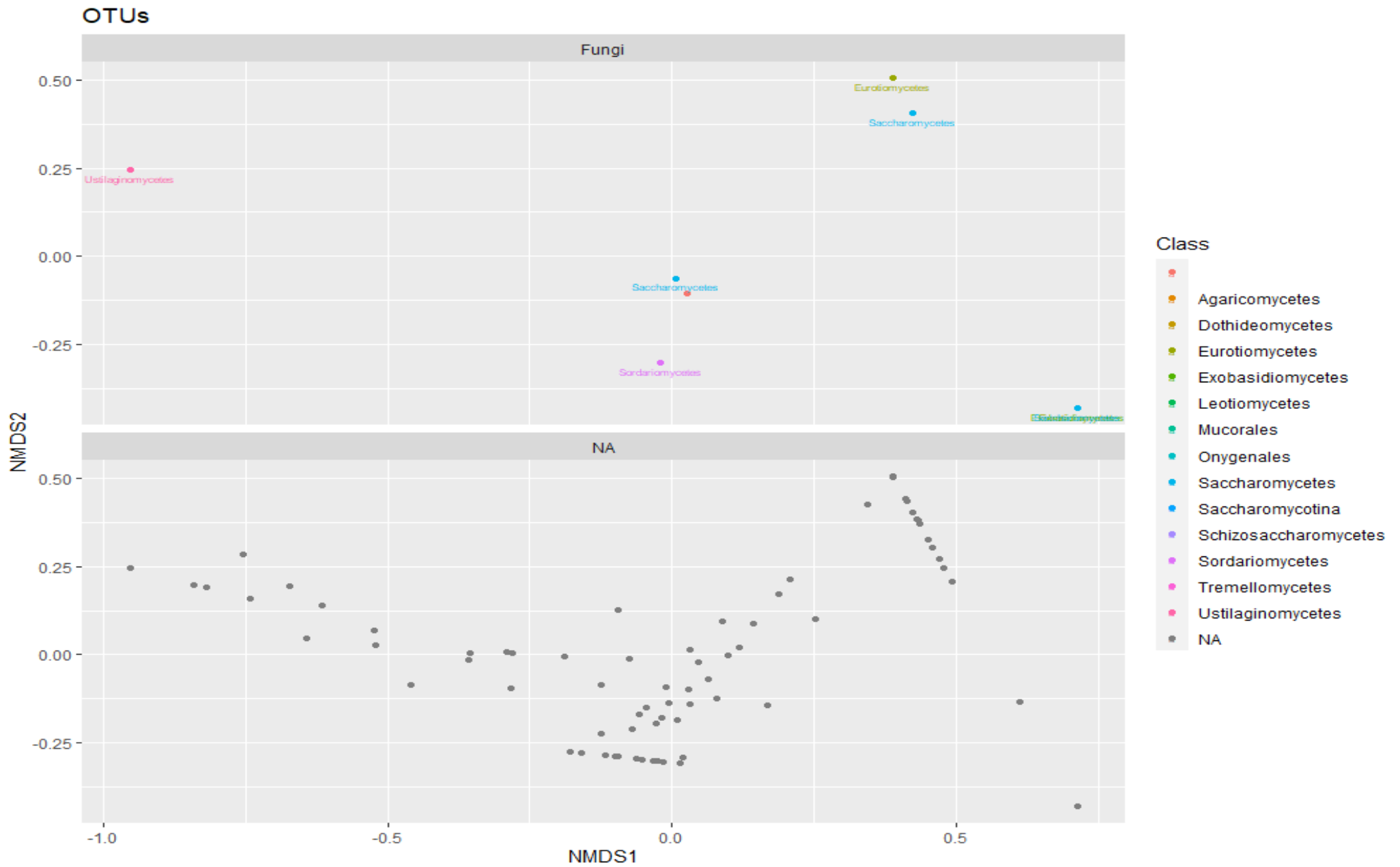
Figure vii. NMDS ordination plot of fungi. The fungi classes were very distant from each other on the plots.
