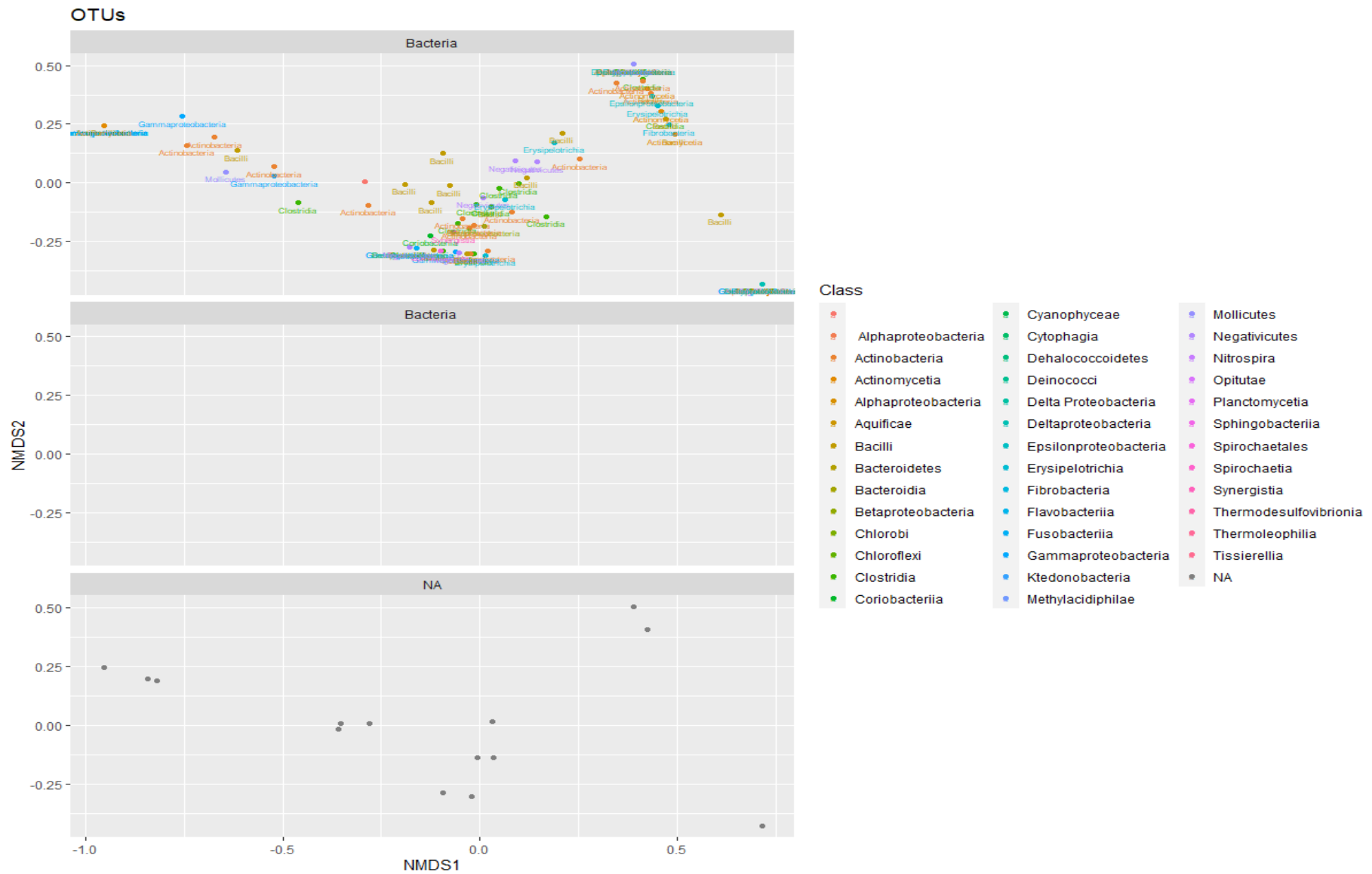
Figure ii. Bacteria ordination (NMDS) plots. Gammaproteobacteria, Bacilli, Erysipelotrichia, Clostridia, and Actinomycetes, filled distinct spaces distant from other classes that clustered together.
