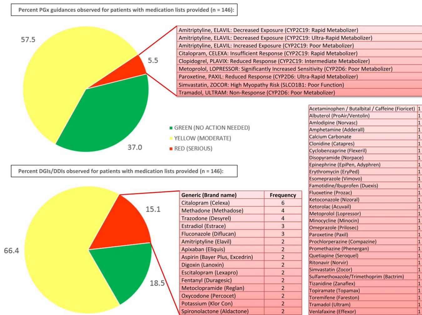
Fig 3. Percent genetic (PGx) dosing guidance, DGI (drug-gene-interactions) and DDI (drug-drug-interactions) observed for patients with medication lists provided (n = 146) sorted by expected normal response to a drug based on PGx, or no interaction observed for DGIs/DDIs. GREEN – no action required, YELLOW (moderate) or RED (serious) interactions prompting actionable PGx or
