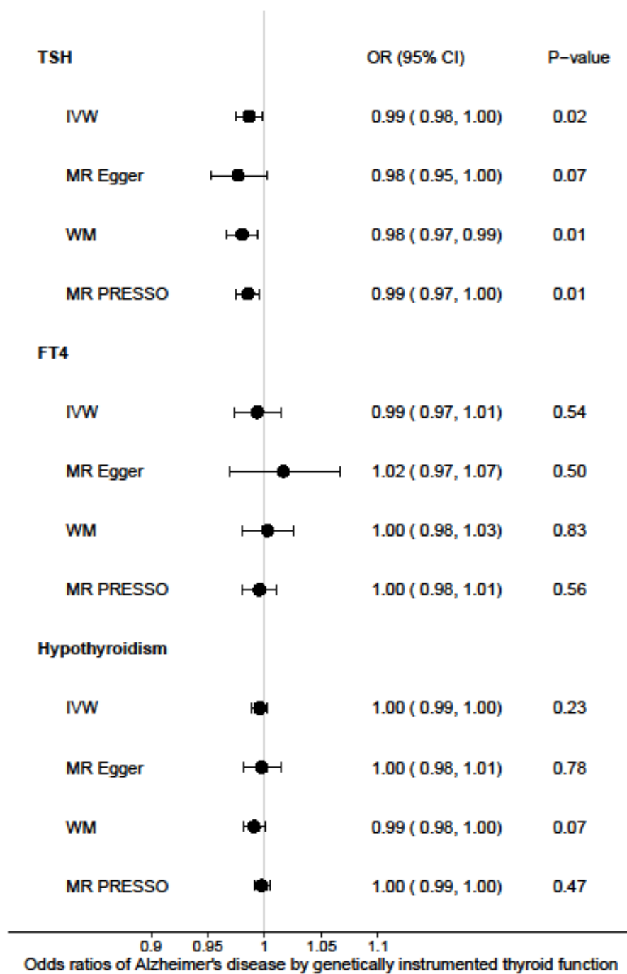
Figure 1. Forest plot = Odds ratios for the effect of genetically determined TSH, FT4 and hypothyroidism on Alzheimer's disease risk.
