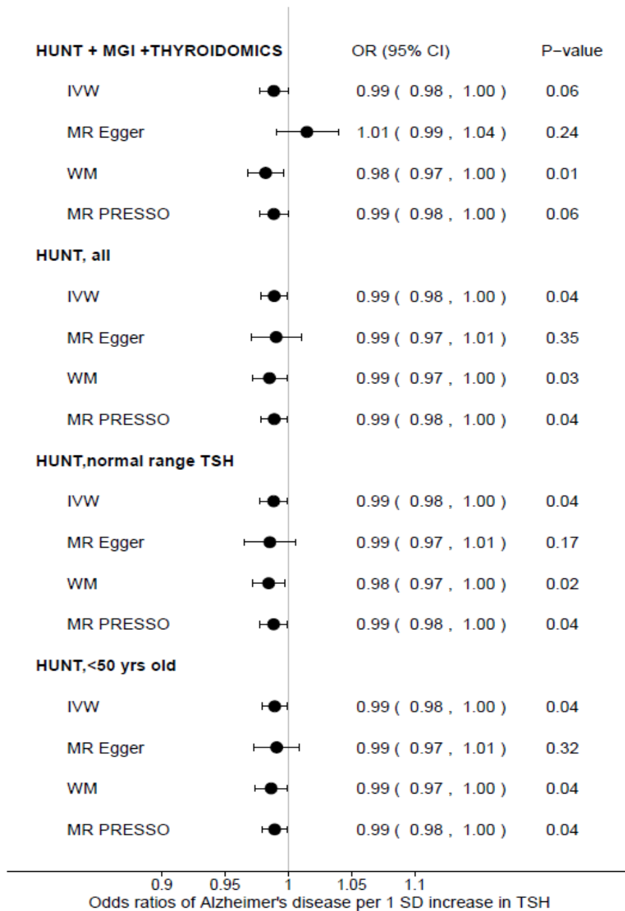
Figure 2. Forest plot for the effect of genetically determined TSH on Alzheimer's disease risk using summary statistics for full range TSH levels (HUNT + MGI + ThyroidOmics meta-analysis), full range TSH levels (HUNT study), TSH within the normal rang in the HUNT study, and TSH levels in individuals younger than 50 years old (HUNT study)
