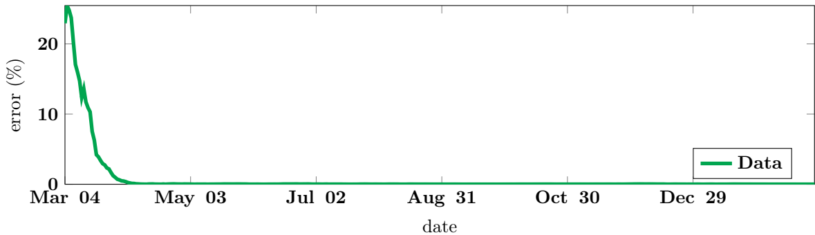
Figure 14: Relative error between the data and the model for California State, expressed in percent.
