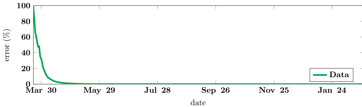
Figure 16: Relative error between the data and the model for India, expressed in percent.
