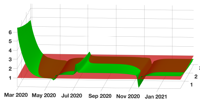
Figure 6: In this figure we plot (t, \kappa) \rightarrow R_e(t) defined in (1.9) when t varies from January 03 2020 to January 04 2021 and \kappa varies from 0.1 to 3.
