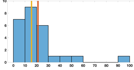
Figure 22: In this Figure we plot the histogram for the estimated values 1/(\chi\theta) (see Appendix E). The red vertical line is mean value which is equal to 21 days. The yellow vertical line is median value which is equal to 15.61 days.
