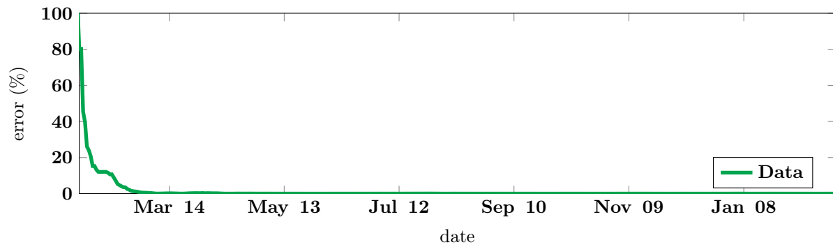
Figure 18: Relative error between the data and the model for Japan, expressed in percent.
