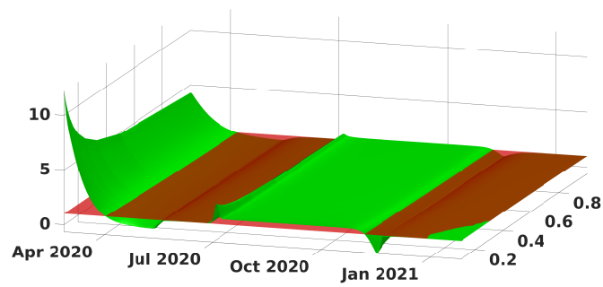
Figure 8: In this figure we plot (t, \nu) \rightarrow R_e(t) defined in (1.9) when t varies from January 03 2020 to January 04 2021 and \nu varies from 0.1 to 1 (or equivalently 1/\nu varies from 10 days to 1 day).
