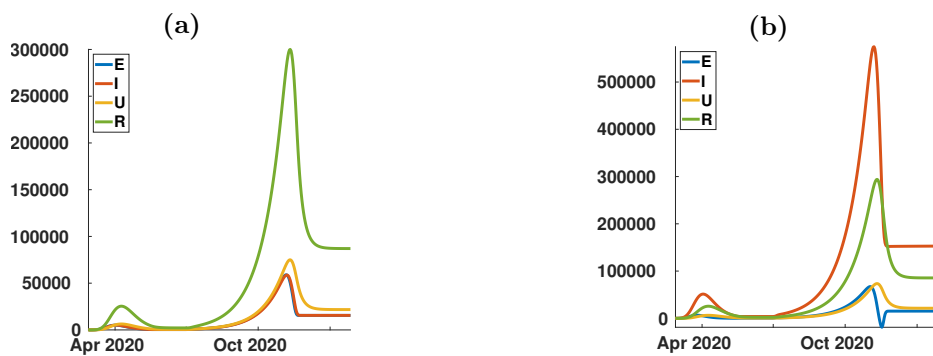
Figure 9: In this figure we explore the influence of the parameter 1/\nu on the solution of model (1.1). The figure (a) corresponds to 1/\nu = 1 and figure (b) corresponds to 1/\nu = 10 . The remaining parameters are unchanged.
