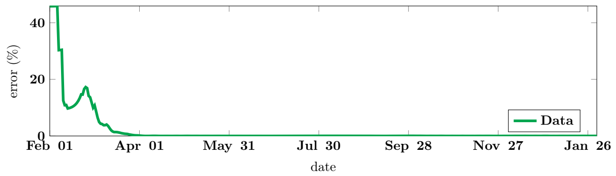
Figure 21: Relative error between the data and the model for UK, expressed in percent.
