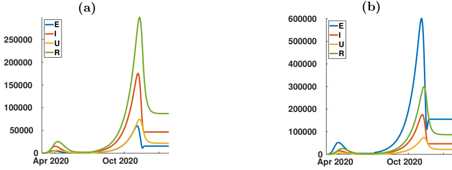
Figure 13: In this figure we explore the influence of the parameter f on the solution of model (1.1). The figure (a) corresponds to 1/\alpha = 1 days and figure (b) corresponds to 1/\alpha = 10 days. The remaining parameters are unchanged.
