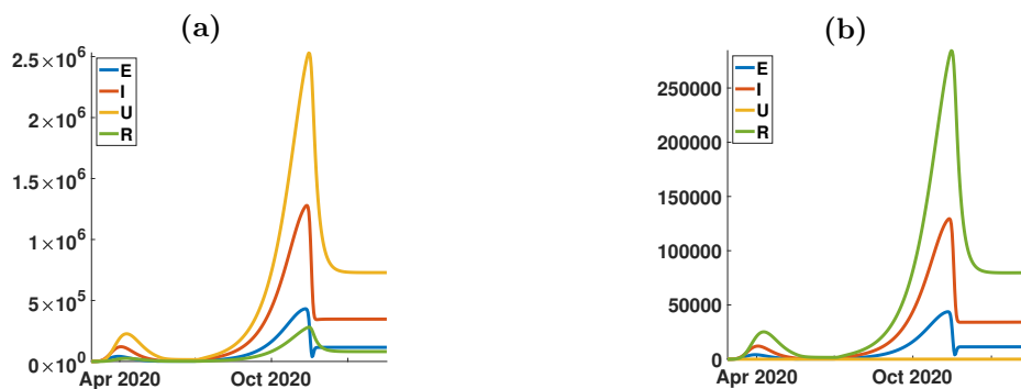
Figure 5: In this figure we explore the influence of the parameter f on the solution of model (1.1). The figure (a) corresponds to f = 0.1 and figure (b) corresponds to f = 1 . The remaining parameters are unchanged.
