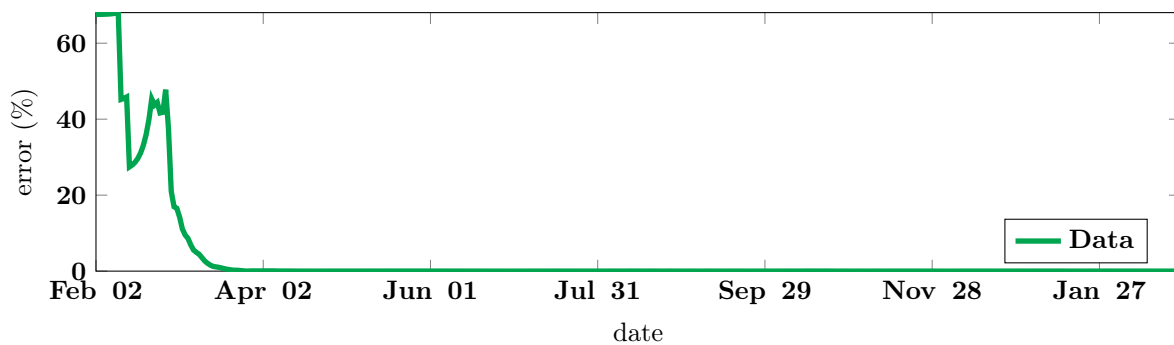
Figure 20: Relative error between the data and the model for Spain, expressed in percent.
