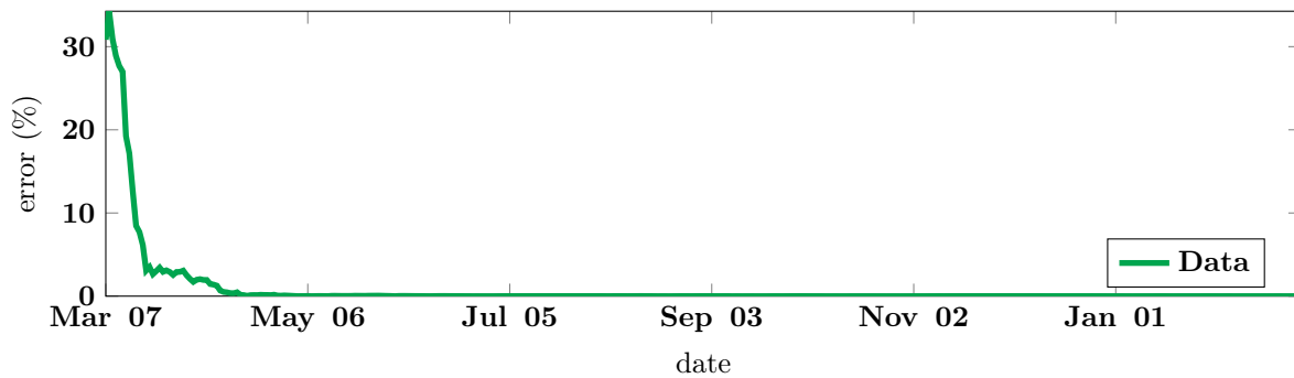
Figure 19: Relative error between the data and the model for Peru, expressed in percent.
