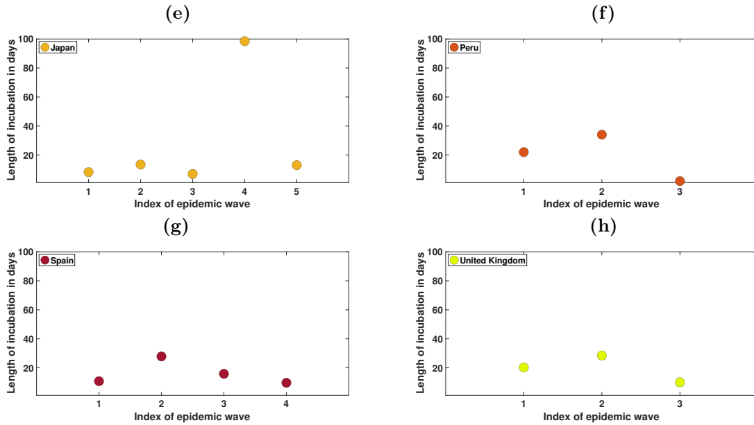
Figure 24: In this figure we plot the values of the parameter 1/(\chi\theta) estimated for each epidemic wave and for Japan (e), Peru (f), Spain (g) and United Kingdom (h). This parameter represents the maximal length of the incubation period. In each figure, we plot this parameter for each epidemic wave and for each country.
