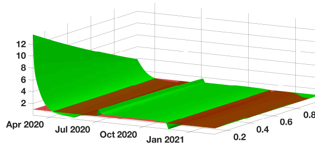
Figure 4: In this figure we plot (t, f) \rightarrow R_e(t) defined in (1.9) when t varies from January 03 2020 to January 04 2021 and f varies from 0.1 to 1.
