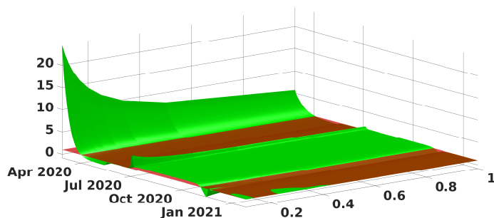
Figure 12: In this figure we plot (t, \alpha) \rightarrow R_e(t) defined in (1.9) when t varies from January 03 2020 to January 04 2021 and \alpha varies from 0.1 to 1 (or equivalently 1/\alpha varies from 10 days to 1 day).
