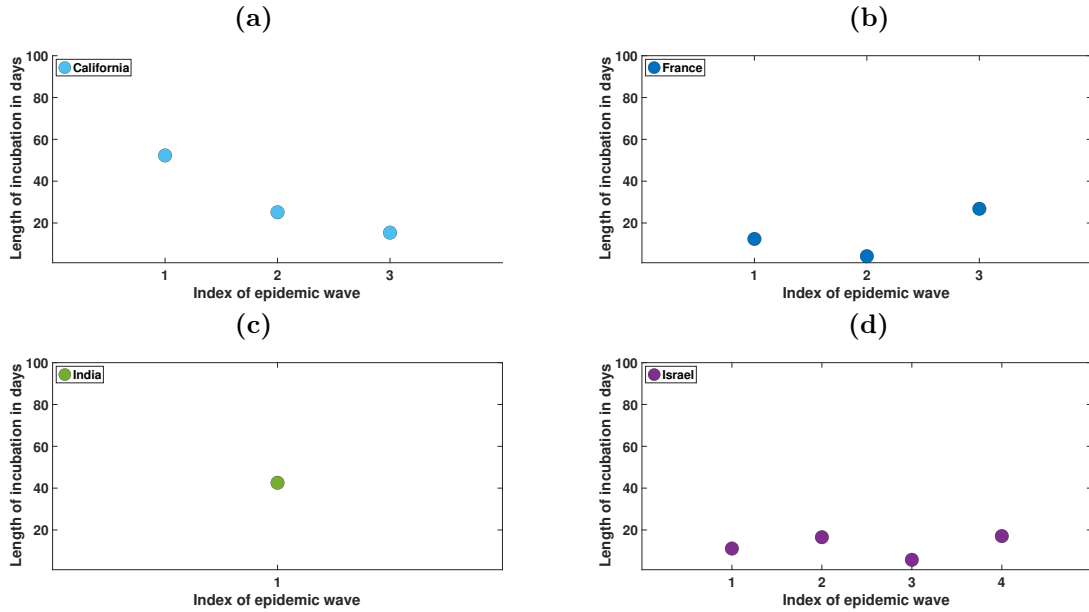
Figure 23: In this figure we plot the values of the parameter 1/(\chi\theta) estimated for each epidemic wave and for California (a), France (b), India (c), Israel (d). This parameter represents the maximal length of the incubation period. In each figure, we plot this parameter for each epidemic wave and for each country.
