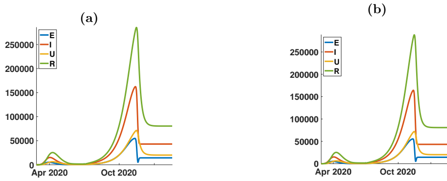
Figure 7: In this figure we explore the influence of the parameter f on the solution of model (1.1). The figure (a) corresponds to \kappa = 0.1 and figure (b) corresponds to \kappa = 3 . The remaining parameters are unchanged.
