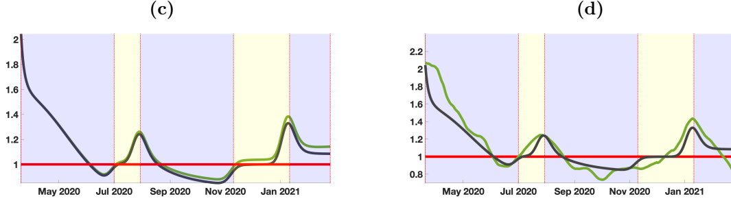
Figure 2: In figure (c) we plot the instantaneous reproduction number R_e(t) defined in (1.9) (in black) and the quasi instantaneous reproduction number R_e^0(t) defined in (1.10) (in green) starting from the beginning of the first epidemic wave. In the figure (d), we plot the instantaneous reproduction number R_e(t) defined in (1.9) (in black) and the one obtained by the standard method [8, 18] (in green). The transmission rate \tau(t) is obtained by using the formula (1.5)-(1.8) together with the phenomenological model plotted in blue in Figure ??-(a). The parameters values used for the simulation are listed in Table 1 and Table 7.
