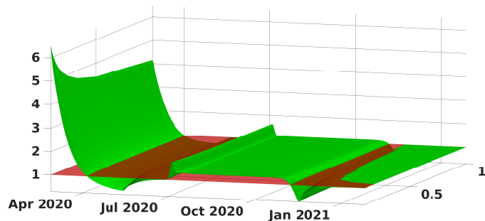
Figure 10: In this figure we plot (t, \eta) \rightarrow R_e(t) defined in (1.9) when t varies from January 03 2020 to January 04 2021 and \eta varies from 0.1 to 1 (or equivalently 1/\eta varies from 10 days to 1 day).
