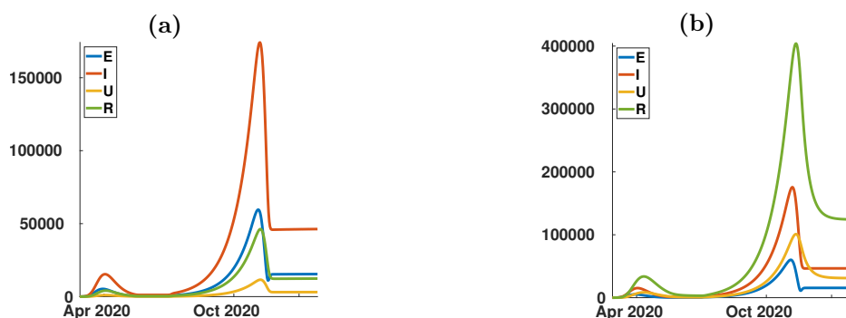
Figure 11: In this figure we explore the influence of the parameter f on the solution of model (1.1). The figure (a) corresponds to 1/\eta = 1 days and figure (b) corresponds to 1/\eta = 10 days. The remaining parameters are unchanged.
