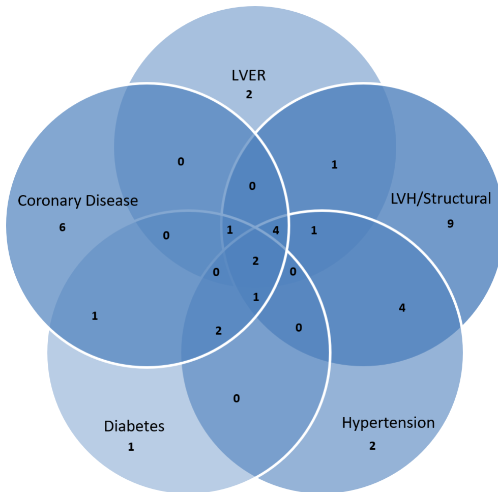
Figure 3. Venn diagram of varying diagnostic groups
