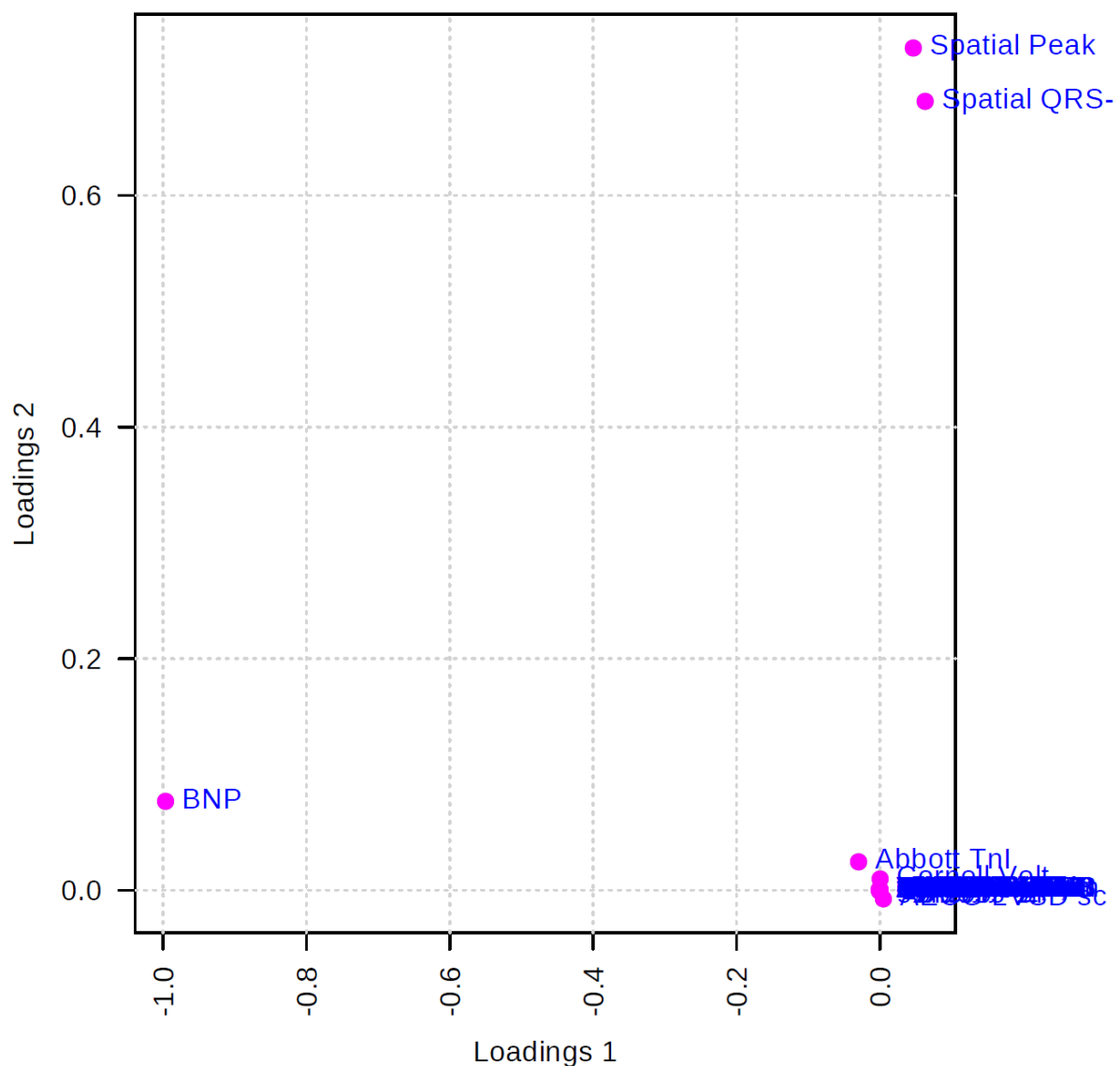
Fig. 1. Loadings plot for the selected Principle Components in the study of left ventricular hypertrophy.
