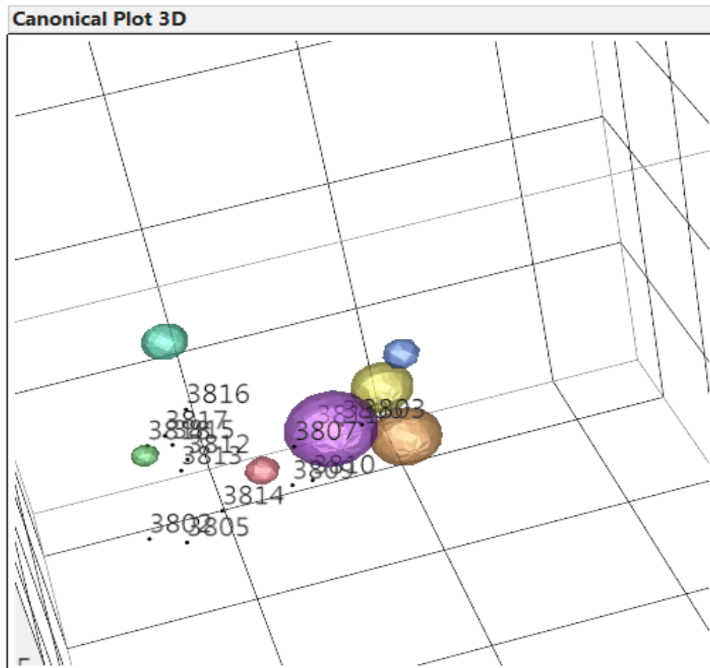
Figure 4. 3D Canonical plot of A-ECG LDA patterns. The lime-green, red and purple spheres represent the 95% confidence intervals for the locations of groups of pre-existing patients with normal heart health, coronary artery disease and left ventricular electrical remodelling, respectively. Numbers represent certain individual patients.
