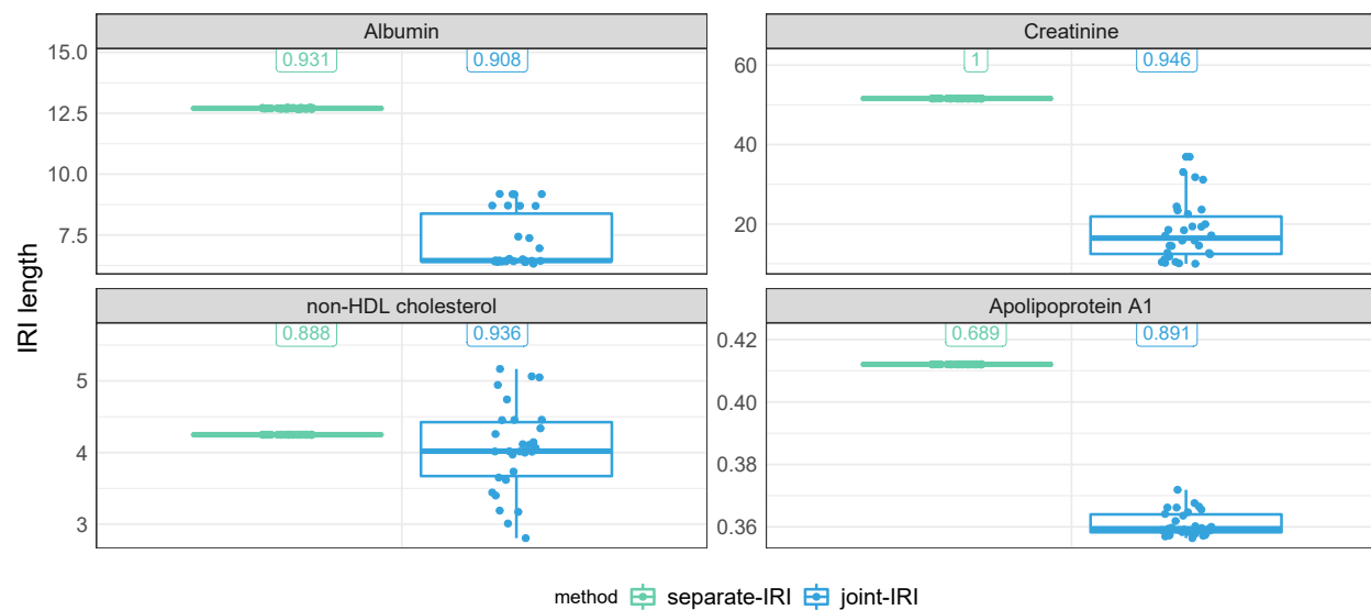
Figure S3: The IRI length distributions of four outcomes measured in the VITO IAM Frontier metabolomics data. The green and blue boxplots refer to IRI lengths estimated by the LQMM method (separate-IRI) and the PJQM method (joint-IRI), respectively. The values on top of each boxplot refer to the corresponding OECs. Extremely small variabilities were observed on the length of separate-IRI due to the limitation of the algorithm to converge at the extreme value of quantile level (e.g. 0.975 or 0.025).
