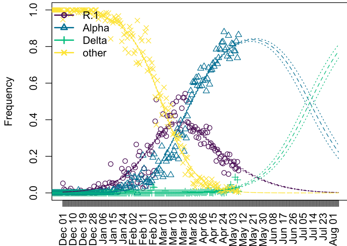
Figure 1. Temporal changes in variant frequencies of R.1 (purple), Alpha (blue), Delta (green), and others (yellow) circulating in Japan from December 1, 2020 to August 6, 2021. The circles, triangles, pluses, and crosses respectively indicate daily frequencies of SARS-CoV-2 sequences of R.1, Alpha, Delta, and others collected in Japan from December 1 2020 to May 8, 2021. The solid lines indicate the maximum likelihood estimates of frequencies of the variants using sequence data collected in Japan from December 1, 2020 to May 8, 2021. The dashed lines represent the predicted variant frequencies after May 8, 2021. Dotted lines indicate lower and upper bounds of 95% CI of estimated variant frequencies.
