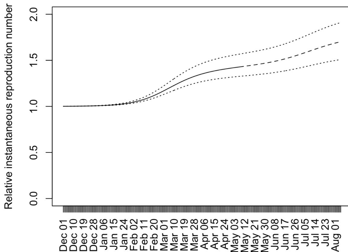
Figure 2. Temporal changes in the population average of the relative instantaneous reproduction numbers with respect to strains circulating before December 1 in Japan. The solid line (until May 8, 2021) and dashed line (after May 8, 2021) indicate the population average of the relative instantaneous reproduction numbers when s_{R,1} = 0.256 , s_{Alpha} = 0.449 , and s_{Delta} = 0.776 , which are calculated by assuming the lognormal serial interval distribution with \mu = 1.38 and \sigma = 0.563 . The lower dotted line indicates the population average of the relative instantaneous reproduction numbers when s_{R,1} = 0.198 , s_{Alpha} = 0.342 and s_{Delta} = 0.557 , which are the lower bounds of s_{R,1} , s_{Alpha} , and s_{Delta} calculated based of the 95% confidence area of the lognormal serial interval distribution. The upper dotted line indicates those when s_{R,1} = 0.335 , s_{Alpha} = 0.596 and s_{Delta} = 1.00 , which are upper bounds calculated in the same way (Figure 2).
