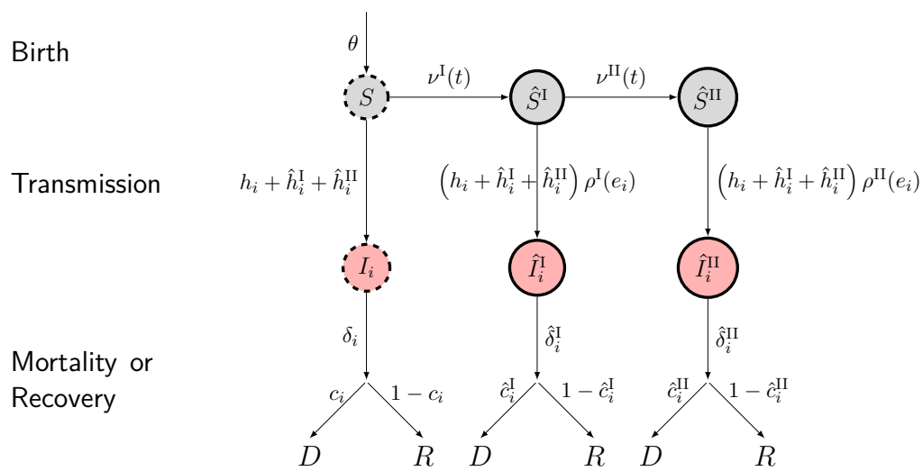
Figure A.2: A schematic representation of the second scenario. Naive and uninfected hosts ( S hosts) are introduced at a rate \theta and are vaccinated at rate \nu^I later on. Hosts vaccinated with one dose ( \hat{S}^I ) receive a second dose at rate \nu^{II} . Uninfected hosts ( S , \hat{S}^I and \hat{S}^{II} ) die at a rate d (unshown) while infected hosts ( I_i , \hat{I}_i^I and \hat{I}_i^{II} ) die at rates \delta_i , \hat{\delta}_i^I and \hat{\delta}_i^{II} respectively, where i refers to the virus genotype: the wild type ( i = w ) or the escape mutant ( i = m ). The rate of infection of naive hosts by the genotype i depends on the forces of infection h_i , \hat{h}_i^I and \hat{h}_i^{II} (see text for details). Vaccination reduces the force of infection and e_i refers to the ability of the genotype i to escape the immunity triggered by vaccination (we assume e_m > e_w ). After infection, hosts can either die or recover, with probabilities c_i , \hat{c}_i^I and \hat{c}_i^{II} .
