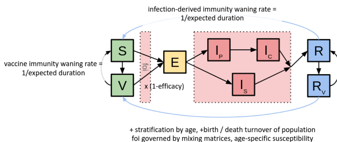
Figure S1: Model diagram.
