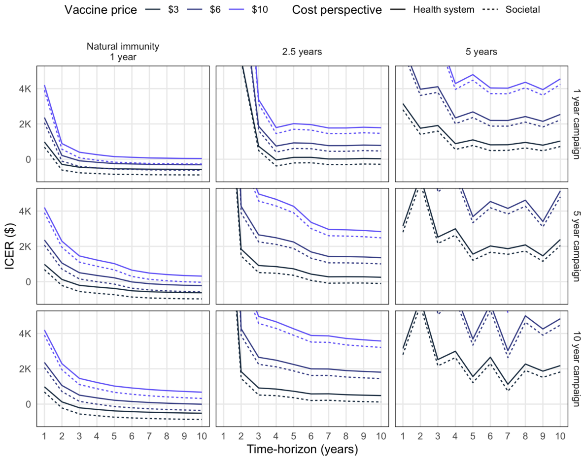
Figure S6: Sensitivity of ICER to time-horizon under different assumptions about vaccine price, costs, campaign duration and duration of natural immunity.
