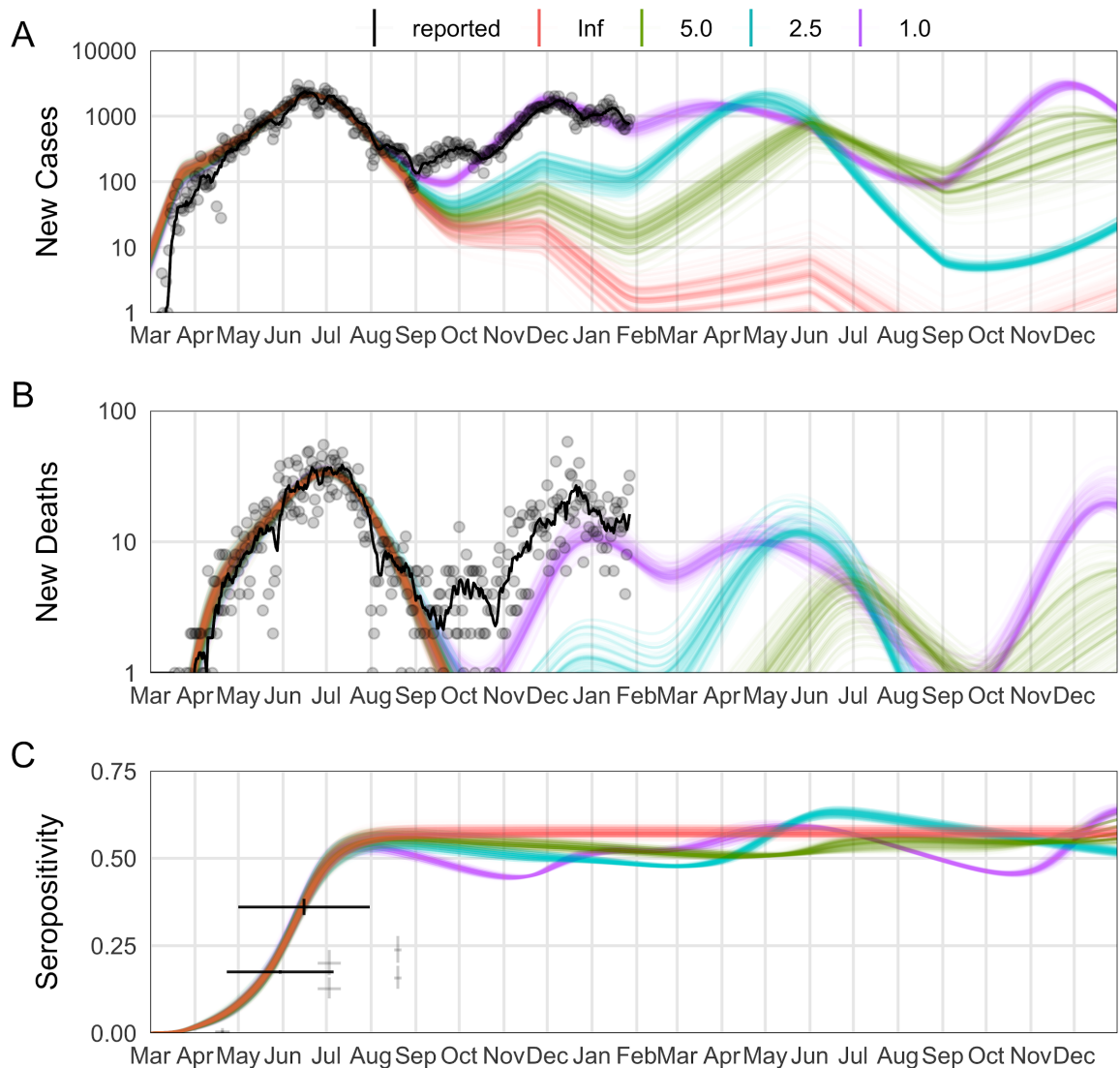
Figure S3: Alternative Infection-Induced Protection Durations.
