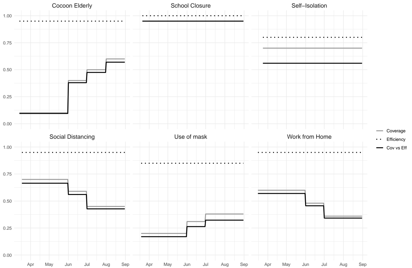
Fig. 2: Diagram of coverage, efficiency and their product for each of the considered non-pharmaceutical interventions considered in the standard model and the model with percolation. The diagrams for the standard model with 30% more NPI coverage would be similar, only 30% higher values.
