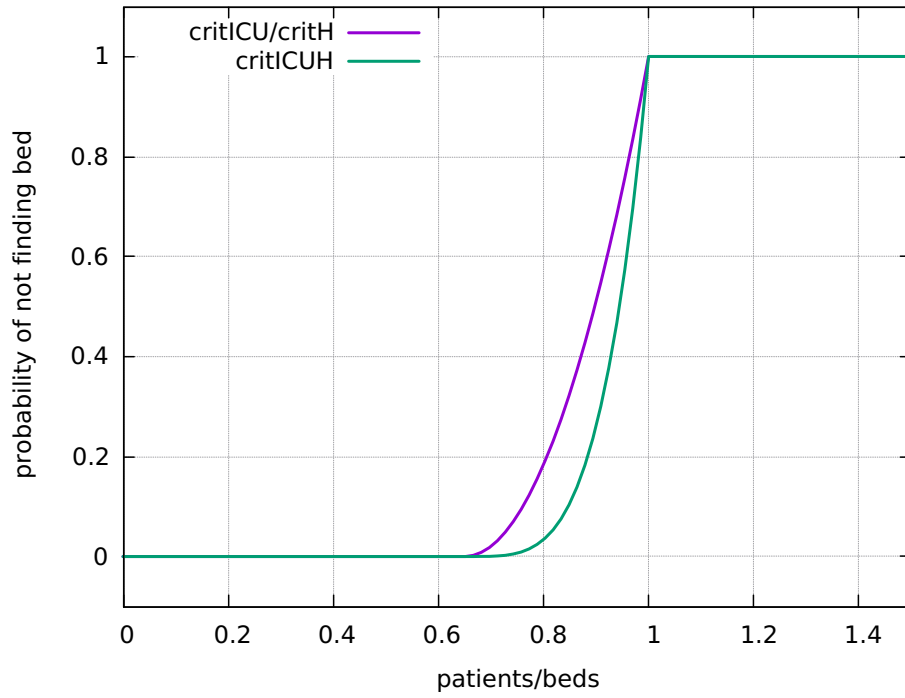
Fig. 1: Probability of not finding a bed as function of the current occupancy. q = 0.65 .
