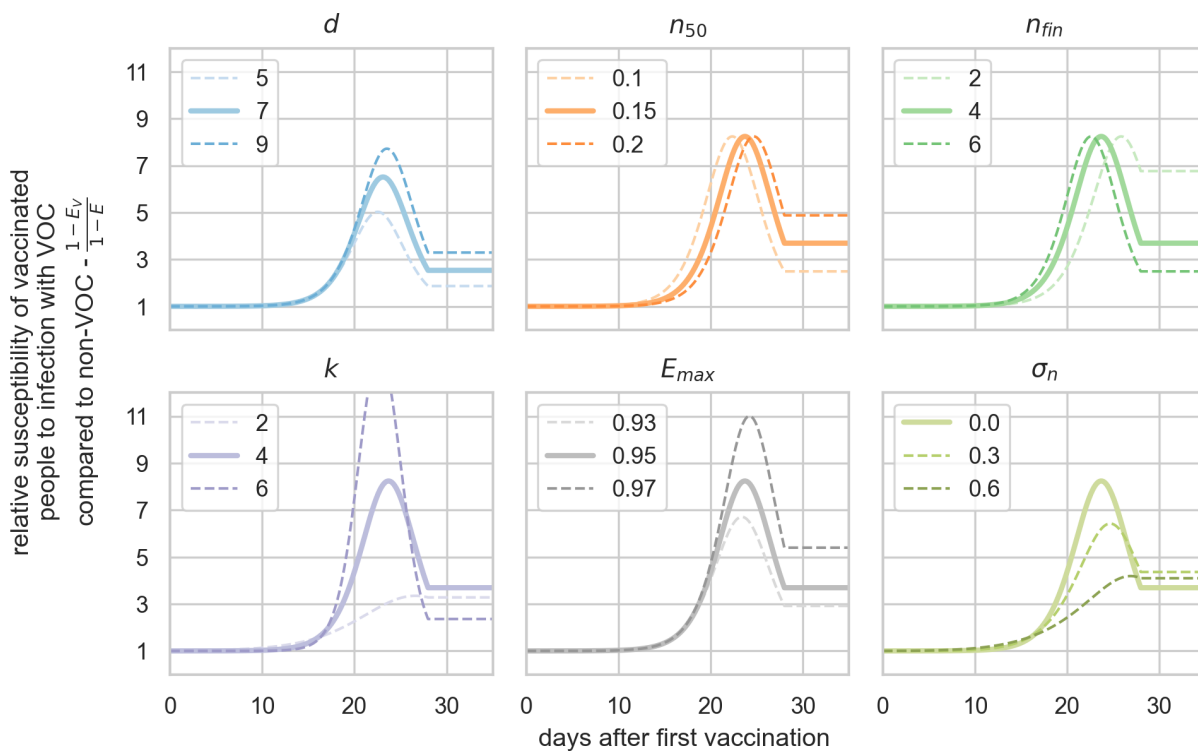
Figure S4 - Sensitivity analysis for the time dependence of the relative susceptibility of vaccinated people to infection with VOC compared to non-VOC. In each panel, we change the value of one of the model parameters to test its influence on our results. For each parameter, the middle value represents the value used in our main analysis, except in the case of \sigma_n (where the default value is 0).
