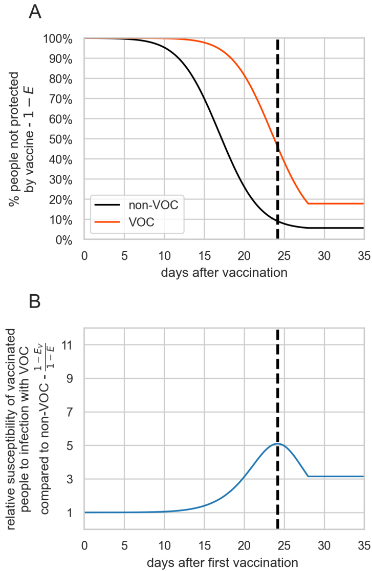
Figure S3 - The effect of adding variability in neutralization levels on the results of Figure 2. The figure is the same as Figure 2 in the main text, except that a standard deviation of 0.3 \log_{10} transformed neutralization levels is used. The other parameter values used are N_{fin}=4 ; d=7 ; K=1.7 ; E_{max}=95\% ; n50=0.15 .
