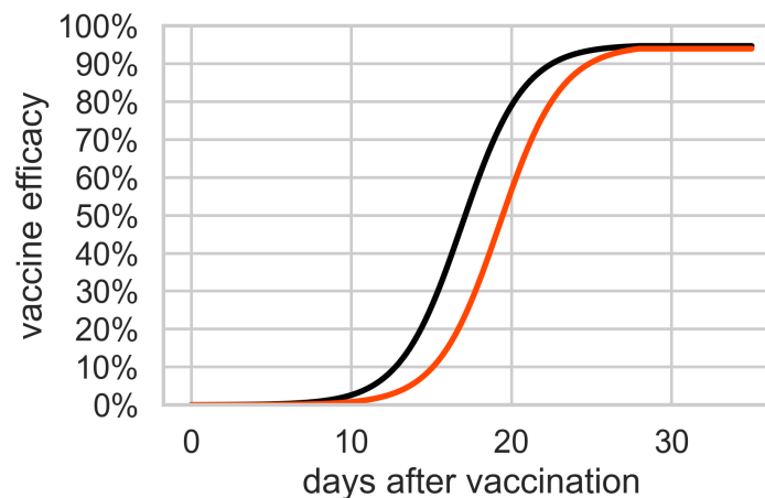
Figure S1 - Estimates of the vaccine efficacy against non-VOC and the B.1.1.7 variant. We use the same framework and in Figure 1 but with different parameter values for d . The parameters used for this analysis are: N_{fin}=4 ; d=2 ; K=1.7 ; E_{max}=95\% ; n_{50}=0.15 .
