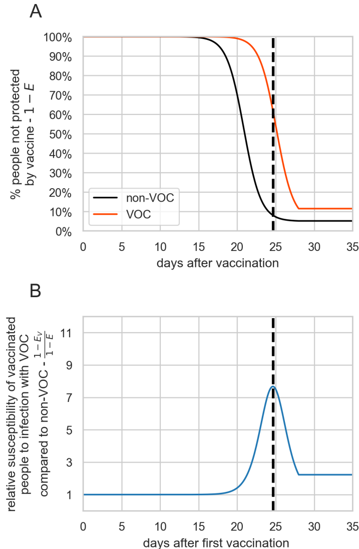
Figure 2 - The relative susceptibility to infection with VOC compared with non-VOC in the vaccinated population. A. The fraction of the vaccinated population not protected by the vaccine, for both the non-VOC strain (in black) and for the VOC strain (in orange) as a function of time since the first vaccine dose. B. The ratio between the susceptibility to infection with VOC and the susceptibility to infection with non-VOC in the vaccinated population, given by \frac{1-E_v}{1-E} and plotted as a function of time since the day of vaccination. The parameter values used to generate the results are: N_{fin}=4 ; d=7 ; K=1.7 ; E_{max}=95\% ; n_{50}=0.15
