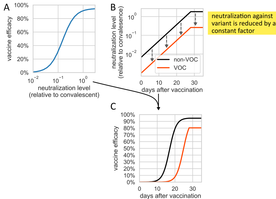
Figure 1 - Schematic representation of the mathematical framework to model vaccine efficacy against VOC versus non-VOC. The model relies on the functional relationship between neutralization levels and vaccine efficacy (A) and the temporal profile of neutralization levels after vaccination (B). Using the functional relationship in A, we can convert neutralization levels into vaccine efficacy and create a temporal profile of vaccine efficacy as a function
