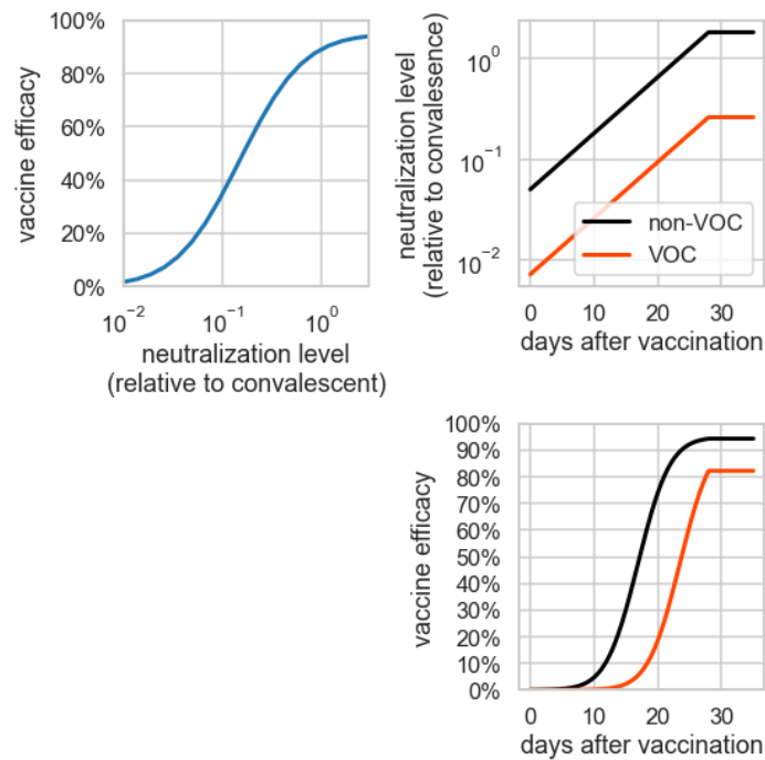
Figure S2 - The effect of adding variability in neutralization levels on the results of Figure 1. The figure is the same as Figure 1 in the main text, except that a standard deviation of 0.3 \log_{10} transformed neutralization levels is used. The other parameter values used are N_{fin}=4 ; d=7 ; K=1.7 ; E_{max}=95\% ; n_{50}=0.15 .
