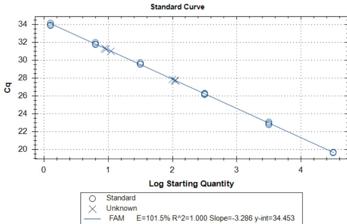
Supplementary Figure S1: Standard curve used in this study: (a) SARS-CoV-2 (N1) (b) BCoV
