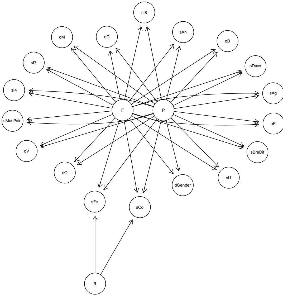
Figure 4: Structure 4 - Model with Cold and rhinitis.
