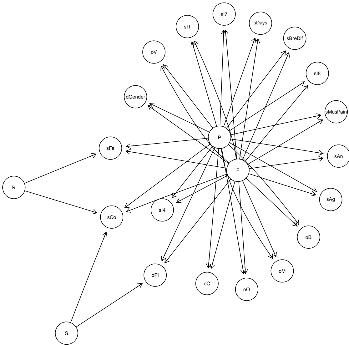
Figure 5: Structure 5 - Model with Cold, smoking and rhinitis.
