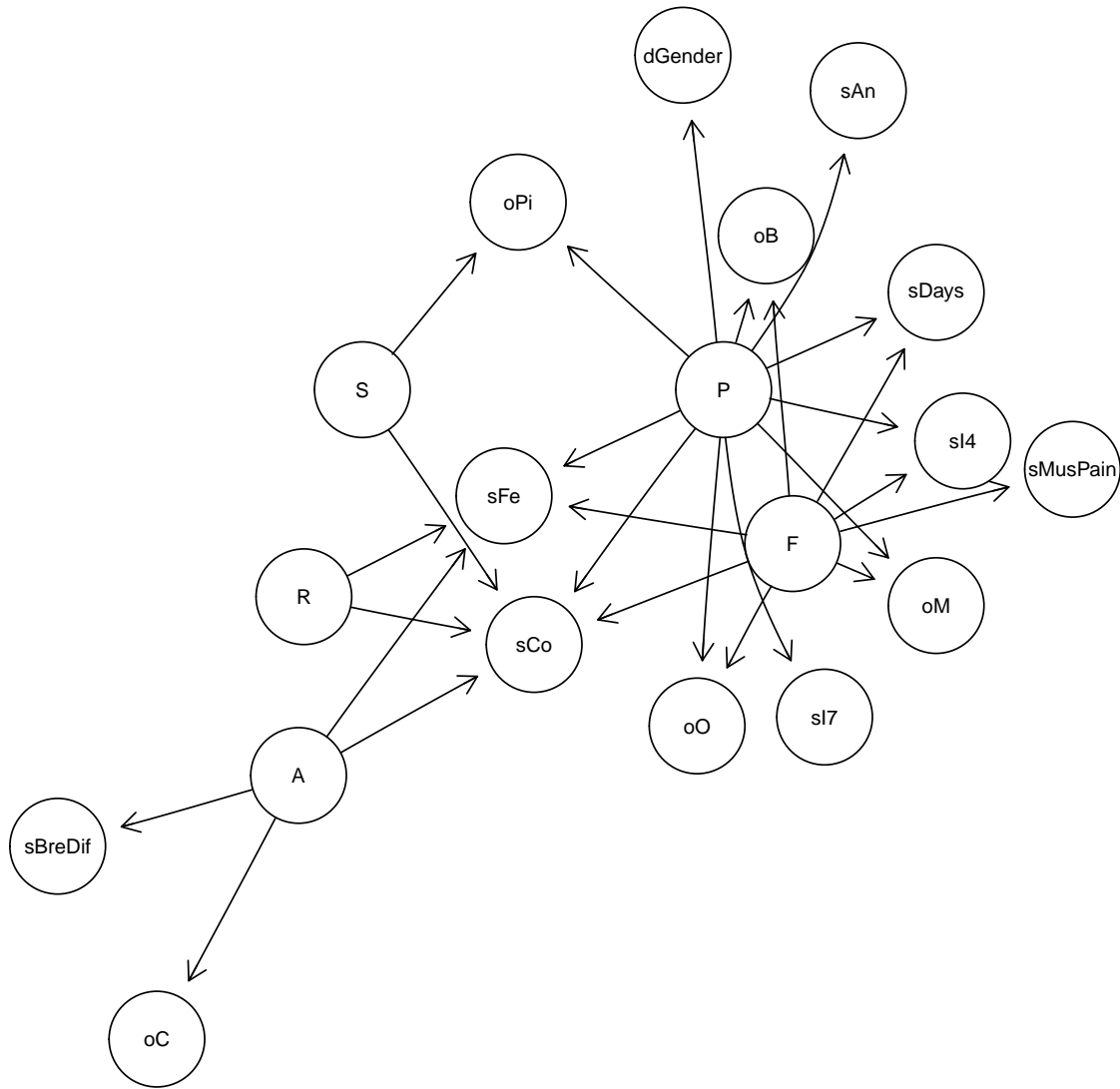
Figure 8: Structure 8 - Model without Cold and only significant covariates.
