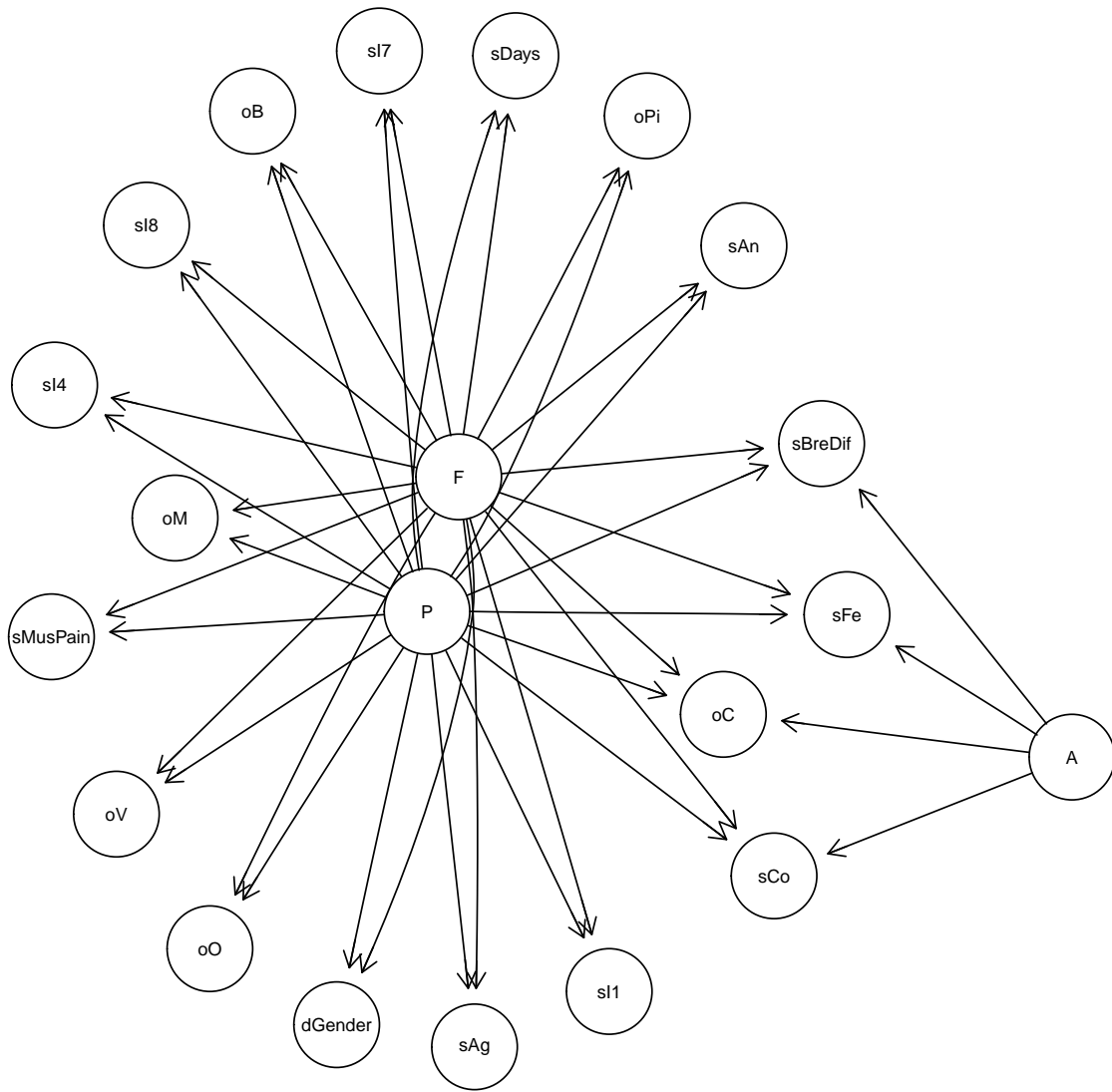
Figure 2: Structure 2 - Model with Cold and allergies.
