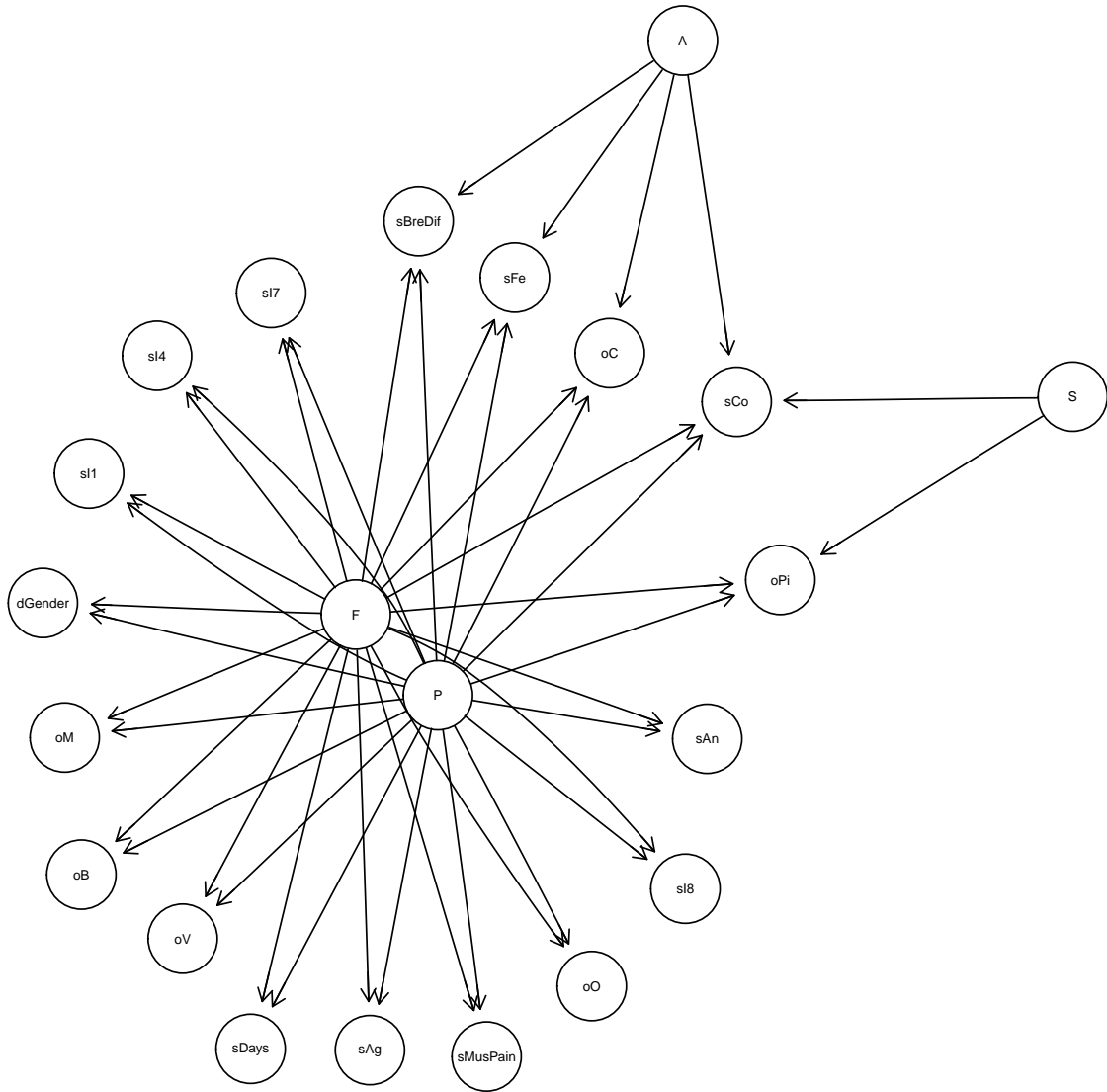
Figure 6: Structure 6 - Model with Cold, smoking and allergies.
