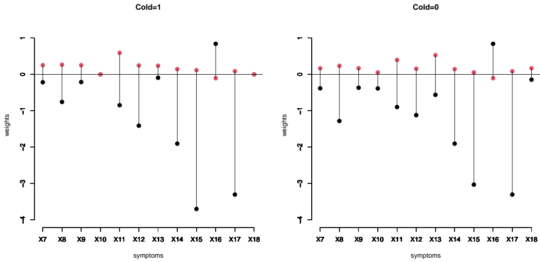
Figure 10: Weights contribution of the symptoms to the risk of a positive PCR result for COVID-19. Red dots represent the weights when there is absence of the symptom or condition, whereas black dots represent the opposite, i.e., presence of the symptom or condition. Cough ( X_7 ), fever ( X_8 ), muscular pain ( X_9 ), breathing difficulty ( X_{10} ), self-reported anosmia ( X_{14} ), ageusia ( X_{15} ), five indicator variables ( X_{11}, X_{12}, X_{13}, X_{16}, X_{17} ) and gender X_{18}
