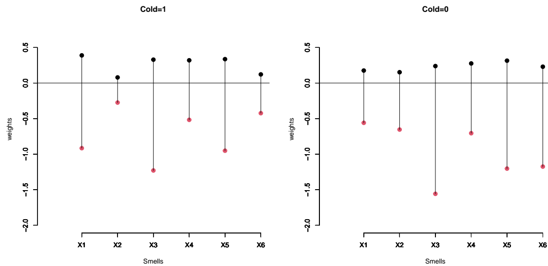
Figure 9: Weights contributions of the recognized odors to the risk of a positive PCR result for COVID-19. Red dots represent the weights when the individual fail to recognize an odor, whereas black dots represent the opposite. X1 = Banana, X2 = Caramel, X3 = Mint, X4 = Orange, X5 = Pineapple, X6 = Vanilla
