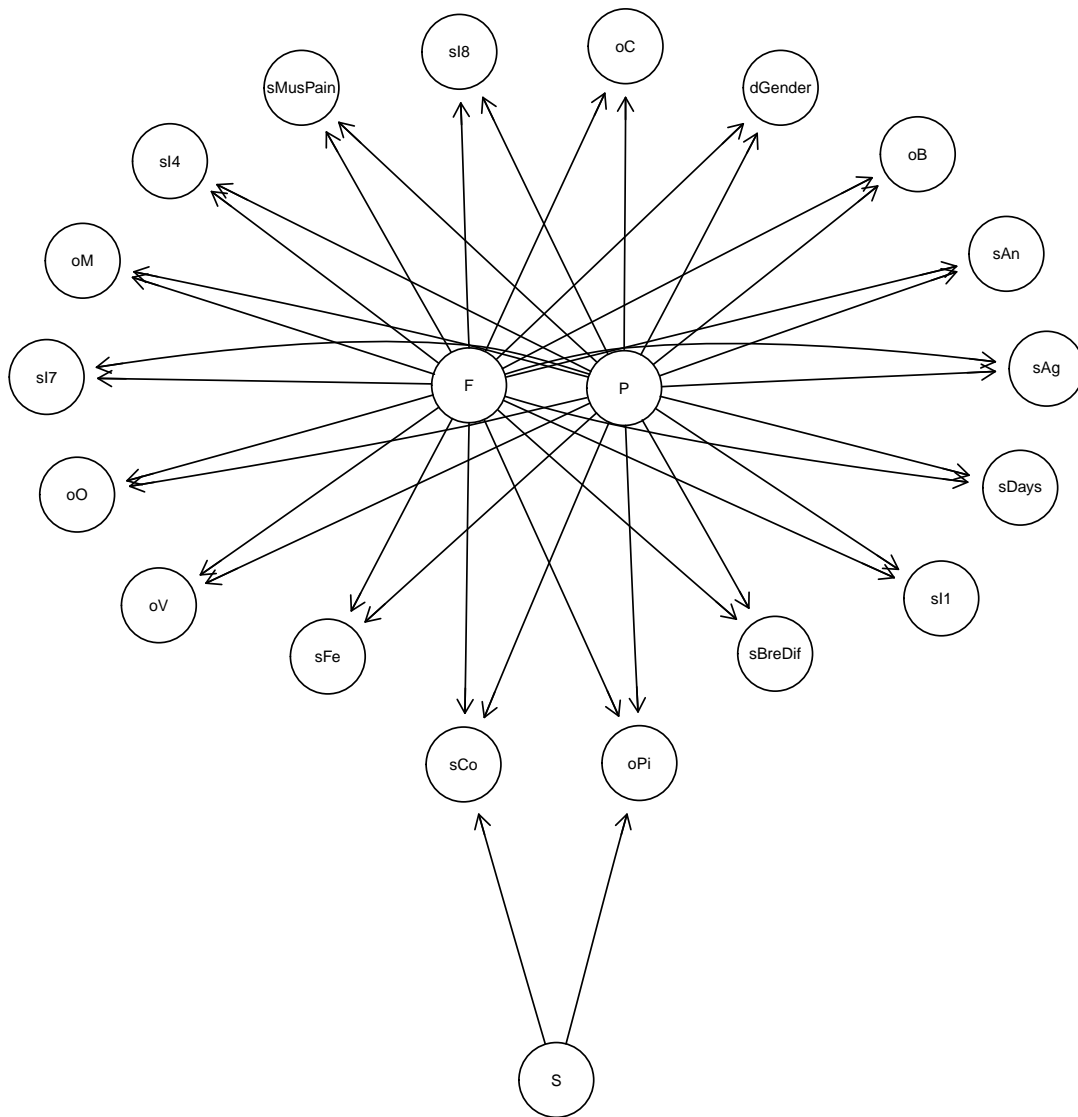
Figure 3: Structure 3 - Model with Cold and smoking.
