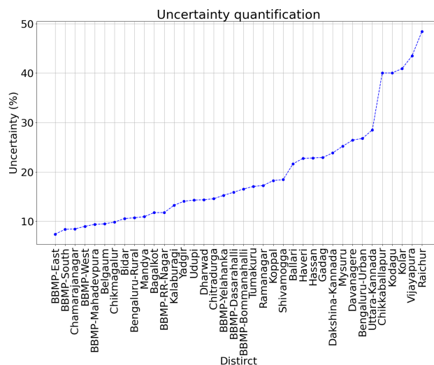
Figure 5: Uncertainty quantification for the validation period in each unit of Karnataka. More than one-half of the units have a root mean squared error of less than 20%. Five districts have errors between 40-50% which are due to the sudden change in trends in the reported cases not captured by the model.
