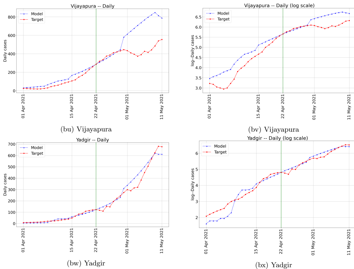
Figure 13: Validation plots for each unit. Calibration has been performed from 08–22 April 2021 and validated during 23 April – 11 May 2021. The vertical line separates the calibration and the validation phases.
