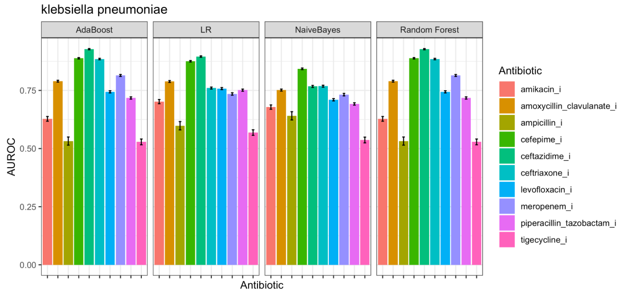
Supp Fig 2.2: AUROC for the antibiotic susceptibility prediction for the Klebsiella pneumoniae
