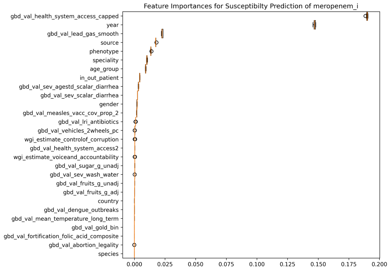
Supp Fig 3: Feature Importance for the Prediction of Meropenem Susceptibility against E.Coli obtained from best performing the Random Forest.
