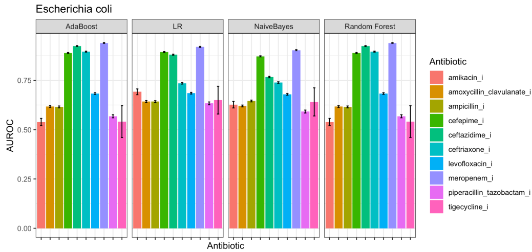
Supp Fig 2.4 AUROC for the antibiotic susceptibility prediction for the E.coli
