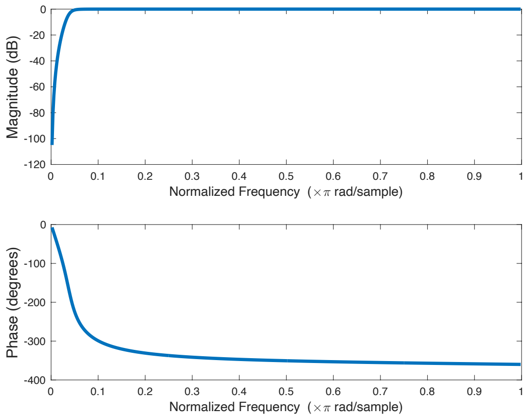
Fig. S9. Bode plot of filter used in accelerometry processing. ( top ) Magnitude response and ( bottom ) phase response of the 4 th order Butterworth high-pass filter ( f_c = 0.2 Hz) used to filter out baseline offsets and static orientation from raw accelerometry ( f_s = 10 Hz).
