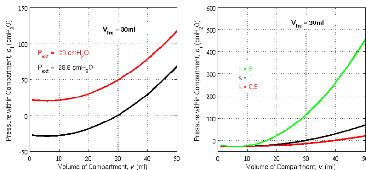
Figure S1.2 The effect of varying the parameters of Equation (18) on the pressure volume relationship of the model ( P_{INSP} = 0 ) and under mechanical ventilation
