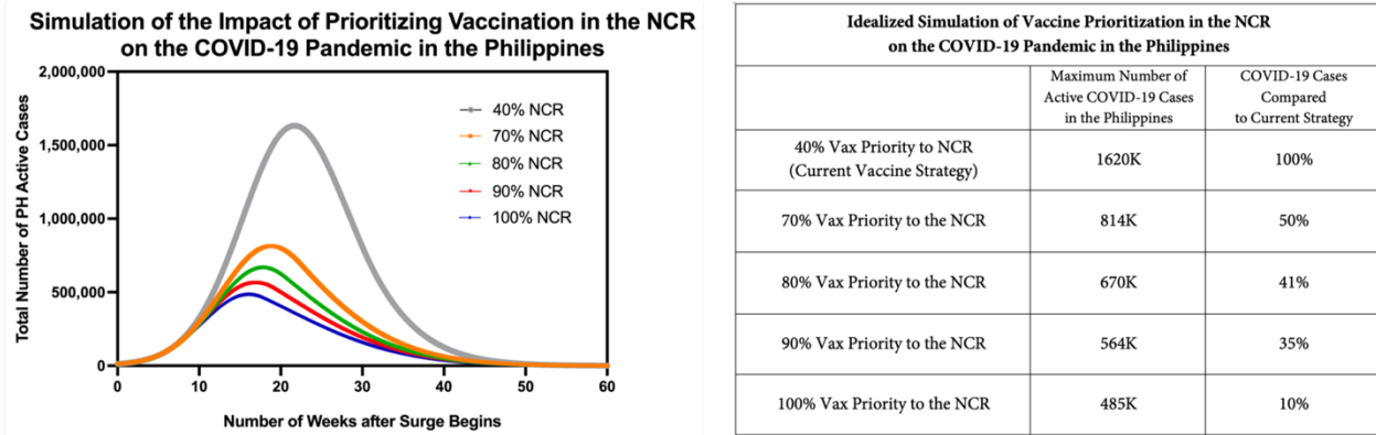
400 Figure 4: Idealized Simulation of the Impact of Prioritizing Vaccination in the NCR 401 on the COVID-19 Pandemic in the Philippines. Forecasted dynamics for the spread of 402 the pandemic in the Philippines after the second surge of COVID-19 without any 403 nonpharmaceutical interventions (NPI) like masking or social distancing in place. We 404 modeled the impact of varying the proportion of 1M vaccines deployed per week in the 405 NCR. The remaining vaccines would be deployed to the rest of the country.
