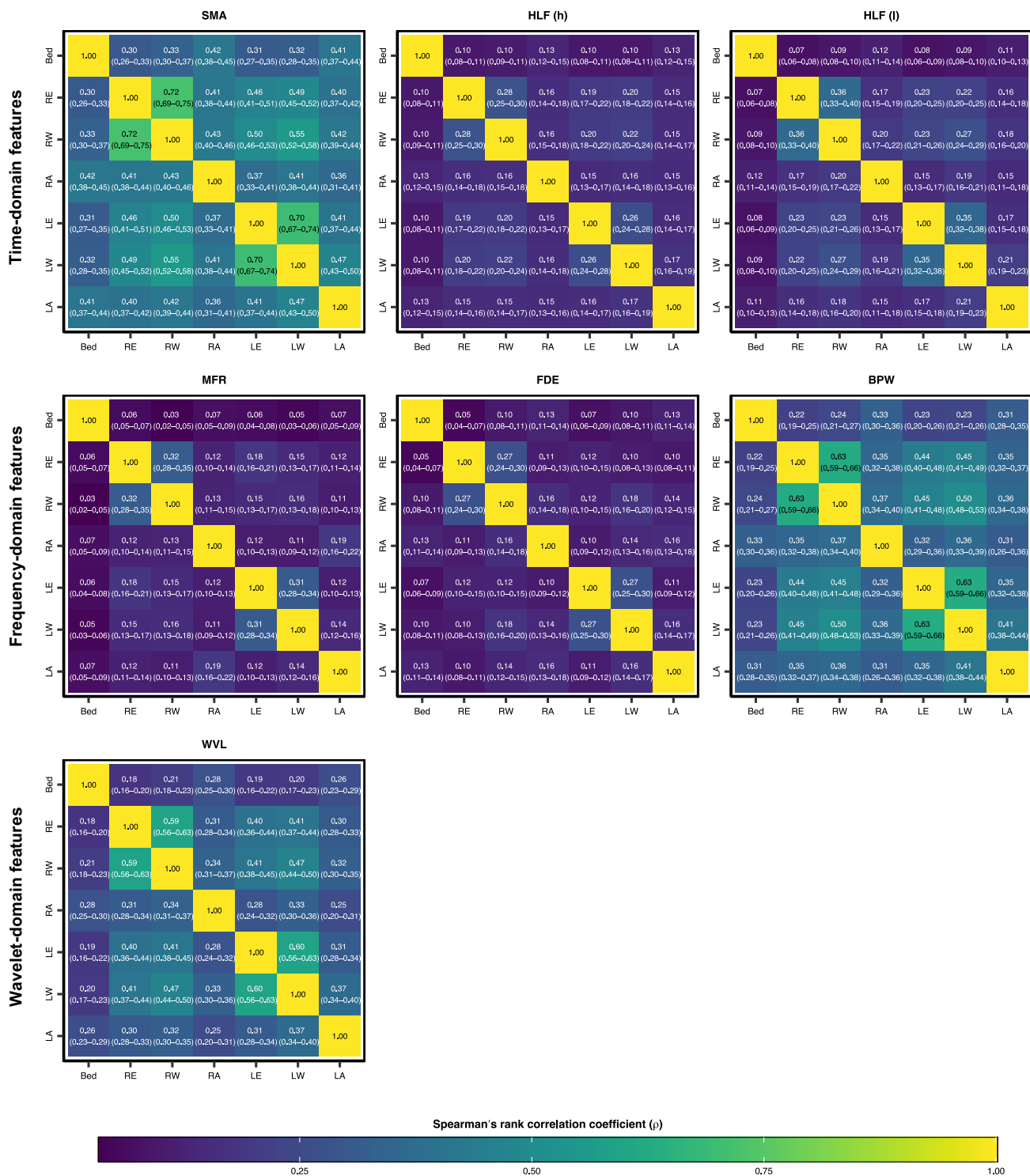
S. Fig. 6. Correlation matrices of extracted motion features across different sensor placements. Each matrix represents a unique feature type and values in each cell of the matrices represent the mean Spearman's rank correlation coefficient ( \rho ) between two sensor placements across the study population ( n = 69 ) with the associated 95% confidence interval (bootstrapped with 10,000 resamples) in parentheses. Sensor placement acronyms correspond to the right and left elbows (RE and LE), the right and left wrists (RW and LW), and the right and left ankles (RA and LE). Feature type acronyms are decoded in Table 4 .
