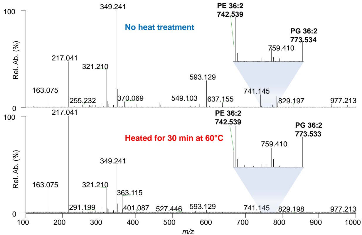
Supplementary Figure 3 Comparison of mass spectra of swabs containing a 10 \mu M PG 36:2 ( m/z 773.533) and PE 36:2 ( m/z 742.539) lipid standard mixture with and without heat inactivation. The mass spectrum on top was obtained from the MasSpec Pen-ESI MS analysis of a swab without heat inactivation while the bottom shows the profile for a swab that had been heat-inactivated at 60°C for 30 min. Both insets are a zoom of m/z 720-800 range to show the detection of the lipid standards.
