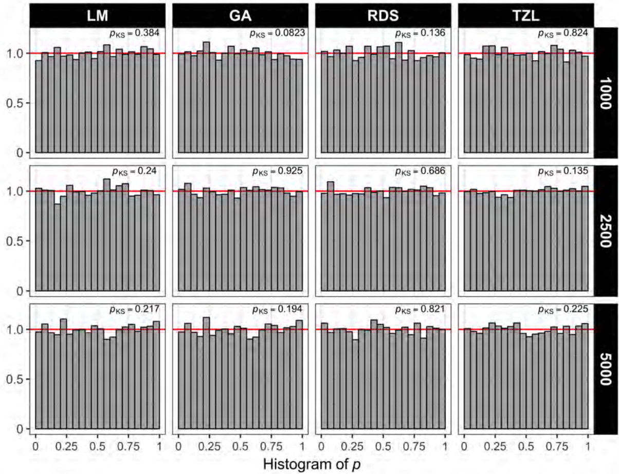
Figure S17: P -value histograms under the null hypothesis and LR test across studied designs in simulation study S4.1 for sample sizes in phases 1 & 2, N = 10000 , when comparing against ranked designs. Column facets correspond to each of the studied designs. Row facets correspond to different phase 2 sample sizes n = 1000, 2500, 5000 ( n/N = 0.10, 0.25, 0.75 ). The top right values in each facet denote the p -value of the Kolmogorov-Smirnov test that the observed p -values follow the expected uniform distribution.
