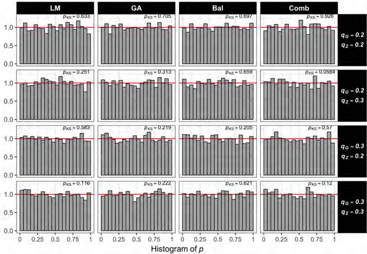
Figure S19: P -value histograms under the null hypothesis and LR test across studied designs in simulation study S4.2 on the joint distribution of G and Z when r = -0.25 and comparing against heuristic designs. Column facets correspond to each of the studied designs. Row facets correspond to four different minor allele frequency combinations for G and Z . The top right values in each facet denote the p -value of the Kolmogorov-Smirnov test that the observed p -values follow the expected uniform distribution.
