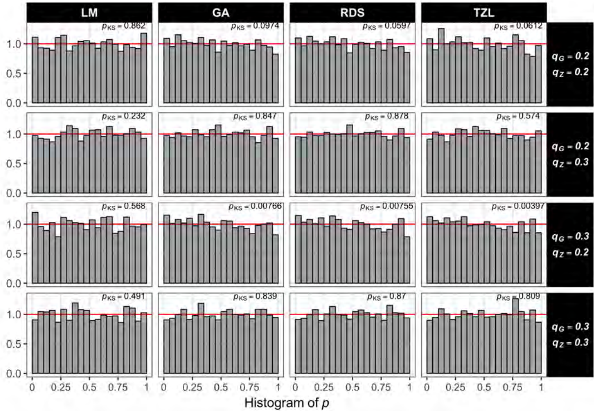
Figure S22: P -value histograms under the null hypothesis and LR test across studied designs in simulation study S4.2 on the joint distribution of G and Z when r = 0.25 and comparing against ranked designs. Column facets correspond to each of the studied designs. Row facets correspond to four different minor allele frequency combinations for G and Z . The top right values in each facet denote the p -value of the Kolmogorov-Smirnov test that the observed p -values follow the expected uniform distribution.
