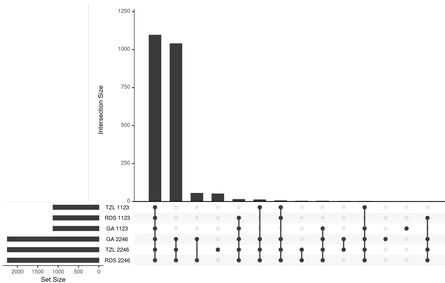
Figure S10: Upset plots for the NFCBB66 data to quantify the intersection sizes across studied designs and phase 2 sample sizes. Each bar denotes the size of a given intersection highlighted in the x-axis.
