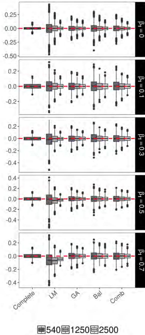
Figure S14: Boxplots for the distribution of the bias across genetic effect estimates ( \hat{\beta}_1 - \beta_1 ) comparing the proposed designs against heuristic designs under a parameter-specific criterion. Row facets denote different true \beta_1 values (0, 0.1, 0.3, 0.5, 0.7). For LM and GA, \mathbb{J}(\Phi)^{-1} was used in the optimization criterion.
