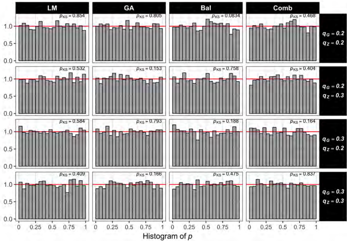
Figure S20: P -value histograms under the null hypothesis and LR test across studied designs in simulation study S4.2 on the joint distribution of G and Z when r = 0.25 and comparing against heuristic designs. Column facets correspond to each of the studied designs. Row facets correspond to four different minor allele frequency combinations for G and Z . The top right values in each facet denote the p -value of the Kolmogorov-Smirnov test that the observed p -values follow the expected uniform distribution.
