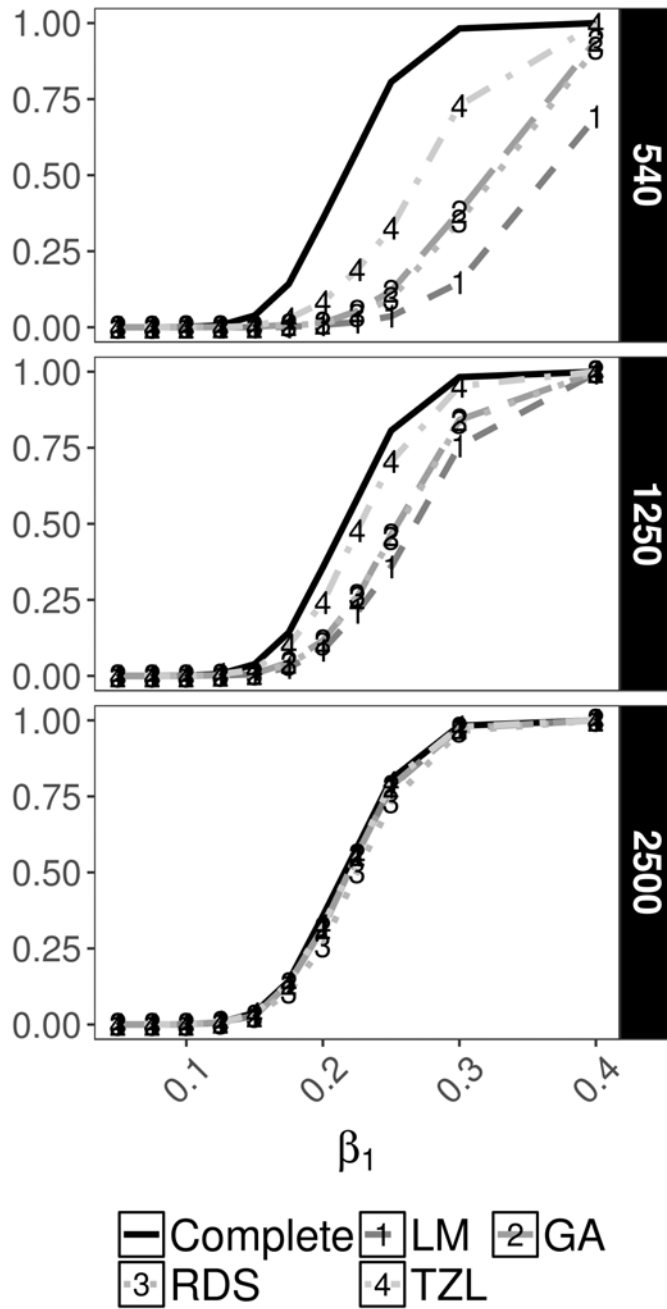
Figure S2: Power curves under the alternative \beta_1 \neq 0 at \alpha = 1 \times 10^{-8} for testing H_0 : \beta_1 = 0 under the LR test and parameter-specific criterion comparing designs across phase 2 sample sizes. Row facets denote different phase 2 sample sizes n = 540, 1250, 2500 .
