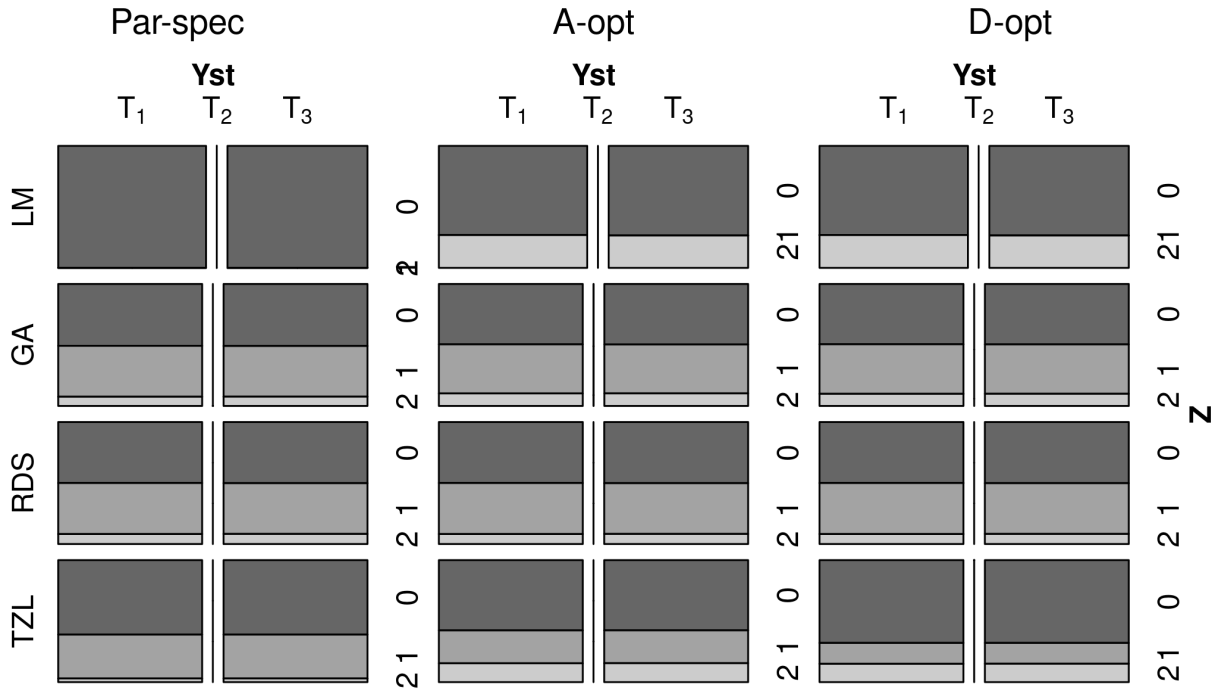
Figure S4: Mosaic plots with the average strata sizes across replicates of the resulting designs in the realistic simulation across optimality criteria (parameter-specific, A-/D-optimality) for n = 1250 .
