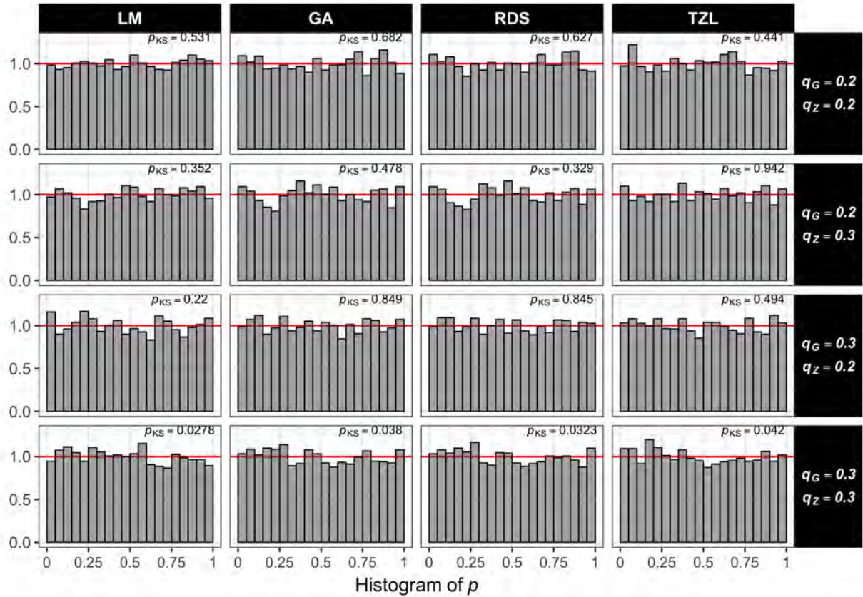
Figure S21: P -value histograms under the null hypothesis and LR test across studied designs in simulation study S4.2 on the joint distribution of G and Z when r = -0.25 and comparing against ranked designs. Column facets correspond to each of the studied designs. Row facets correspond to four different minor allele frequency combinations for G and Z . The top right values in each facet denote the p -value of the Kolmogorov-Smirnov test that the observed p -values follow the expected uniform distribution.
