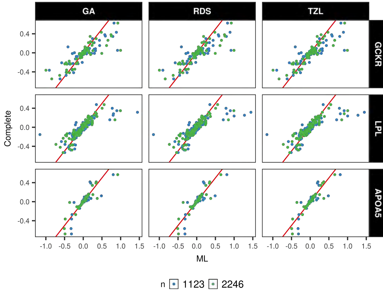
Figure S11: Beta-Beta plots for the ML analyses under the studied designs compared to the complete data analysis in the NFCBB66 data. Column facets shows one studied design whereas row facets denote each loci of interest.
