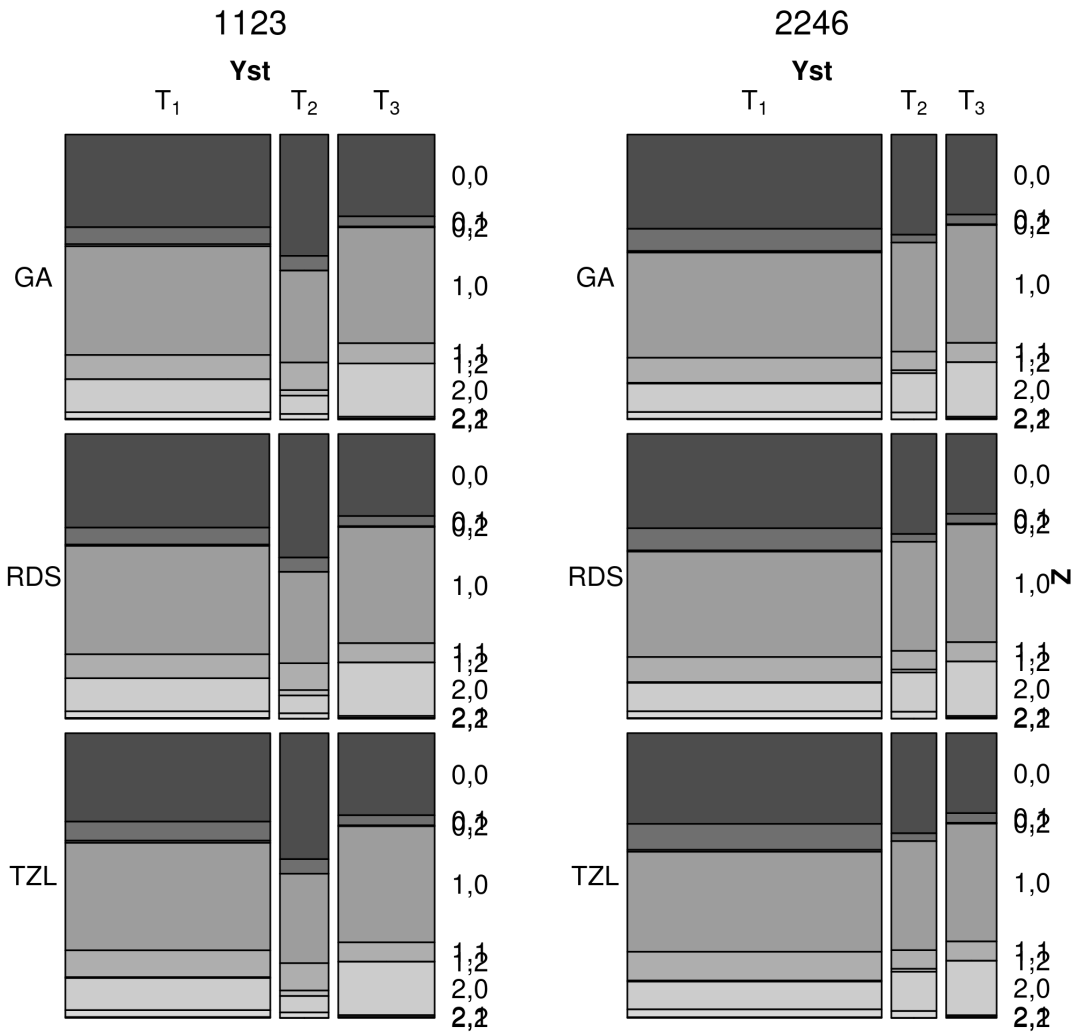
Figure S9: Mosaic plots for the strata distribution across studied designs GA, RDS, and TZL in NFBC66 data across different phase 2 sample sizes. Each column shows the corresponding designs for each phase 2 sample size.
