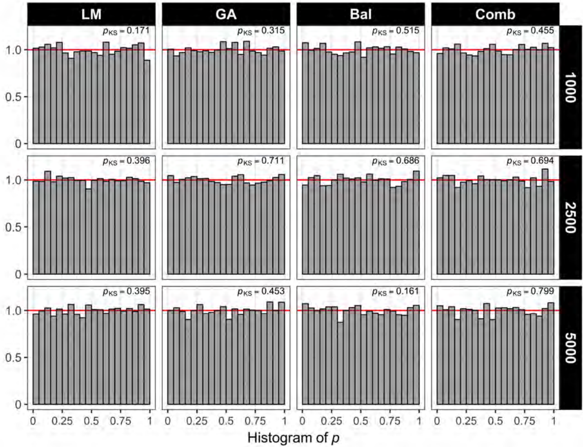
Figure S16: P -value histograms under the null hypothesis and LR test across studied designs in simulation study S4.1 for sample sizes in phases 1 & 2 when comparing against heuristic designs. Column facets correspond to each of the studied designs. Row facets correspond to different phase 2 sample sizes n = 1000, 2500, 5000 ( n/N = 0.10, 0.25, 0.75 ). The top right values in each facet denote the p -value of the Kolmogorov-Smirnov test that the observed p -values follow the expected uniform distribution.
