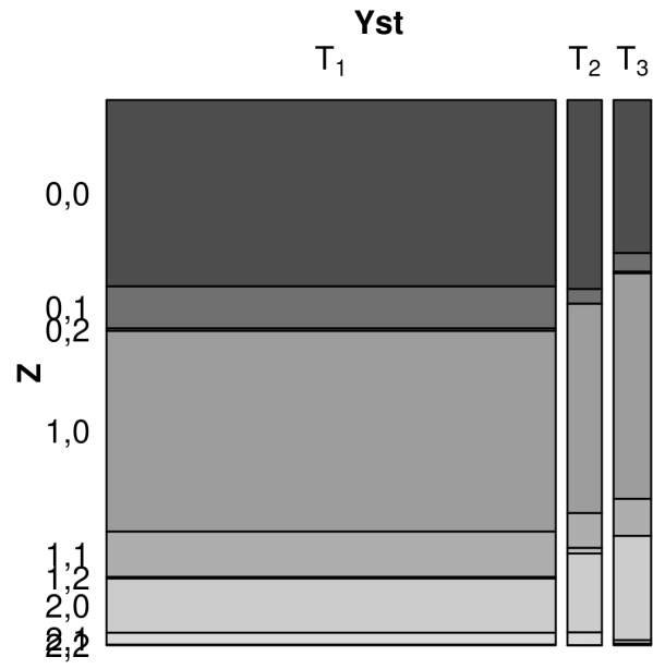
Figure S8: Mosaic plots for the strata distribution in NFBC66 phase 1 data.
