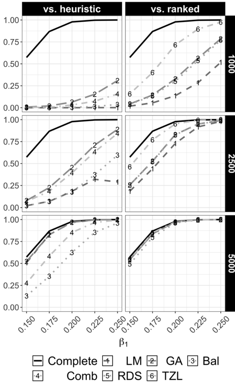
Figure S18: Power curves under the alternative \beta_1 \neq 0 at \alpha = 5 \times 10^{-8} for testing H_0 : \beta_1 = 0 under the LR test across studied designs in simulation study S4.1 for sample sizes in phases 1 & 2, N = 10000 . Row facets denote phase 2 sample sizes ( n = 1000, 2500, 5000 ) whereas column facets denote the design comparison (vs heuristic or vs. ranked, respectively).
