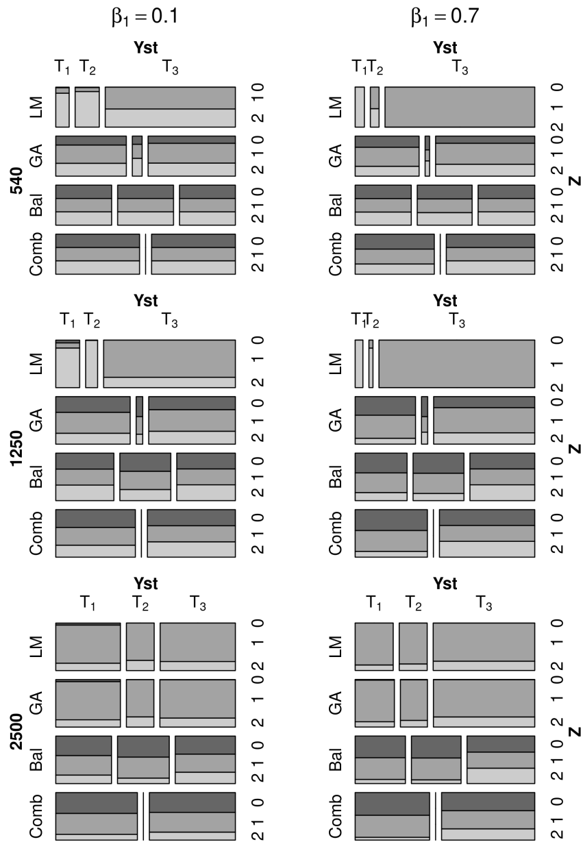
Figure S12: Mosaic plots with the average strata sizes across replicates for the proposed designs against heuristic designs across phase 2 sample sizes ( n = 540, 1250, 2500 ) under the parameter-specific criterion. Averages were taken from the resulting designs in the main simulation study for the two most extreme values of \beta_1 (0.1, 0.7). For LM and GA, J(\Phi)^{-1} was used in the optimization criterion.
