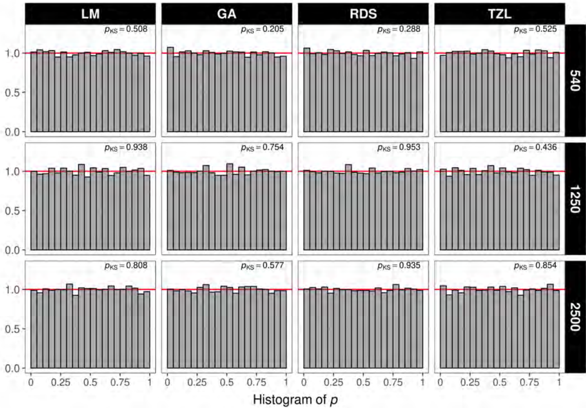
Figure S1: P -value histograms under the null hypothesis and LR test in the comparison against ranked designs across optimality criteria and phase 2 sample sizes ( n = 540, 1250, 2500 ). Column facets correspond to each of the studied designs. Row facets correspond to each phase 2 sample size. The top right values in each facet denote the p -value of the Kolmogorov-Smirnov test that the observed p -values follow the expected uniform distribution.
