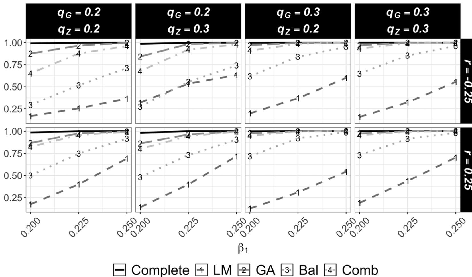
Figure S23: Power curves under the alternative \beta_1 \neq 0 at \alpha = 5 \times 10^{-8} for testing H_0 : \beta_1 = 0 under the LR test across studied designs in simulation study S4.2 for the joint distribution of G and Z when comparing against heuristic designs. Row facets denote the level of linkage correlation between G and Z measured through r ( -0.25, 0.25 ). Column facets denote four different minor allele frequency combinations for G and Z .
