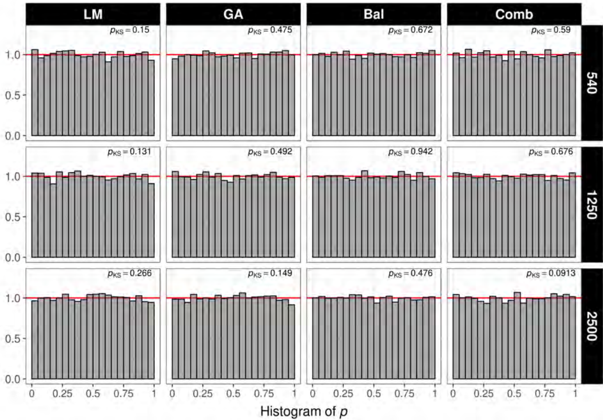
Figure S13: P -value histograms under the null hypothesis and likelihood ratio (LR) test in the comparison against heuristic designs across phase 2 sample sizes ( n = 540, 1250, 2500 ). Column facets correspond to each of the studied designs. Row facets correspond to each phase 2 sample size. The top right values in each facet denote the p -value of the Kolmogorov-Sminrnov test that the observed p -values follow the expected uniform distribution. For LM and GA, \mathbb{J}(\Phi)^{-1} was used in the optimization criterion.
