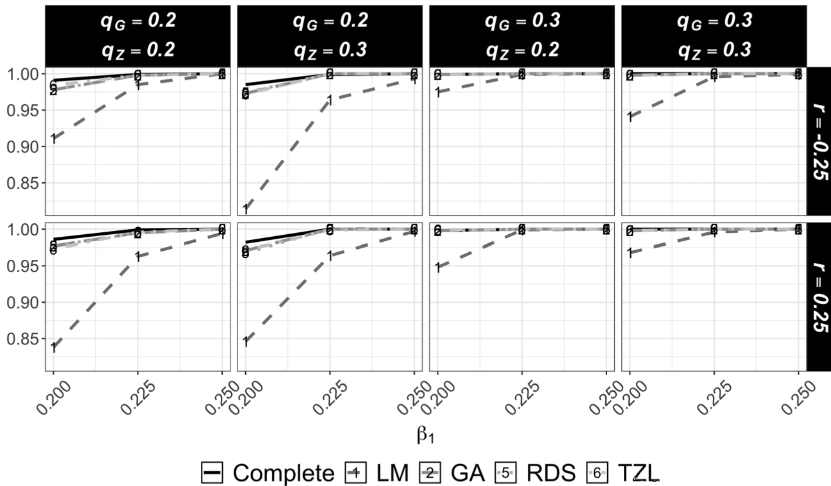
Figure S24: Power curves under the alternative \beta_1 \neq 0 at \alpha = 5 \times 10^{-8} for testing H_0 : \beta_1 = 0 under the score test across studied designs in simulation study S4.2 for the joint distribution of G and Z when comparing against ranked designs. Row facets denote the level of linkage correlation between G and Z measured through r ( -0.25, 0.25 ). Column facets denote four different minor allele frequency combinations for G and Z .
