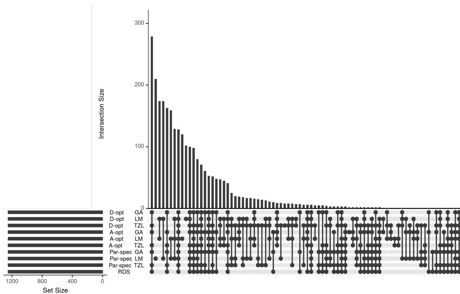
Figure S3: Upset plots for a single replicate in the realistic simulation to quantify the intersection sizes across studied designs and optimality criteria when n = 1250 . Each bar denotes the size of a given intersection highlighted in the x-axis.
