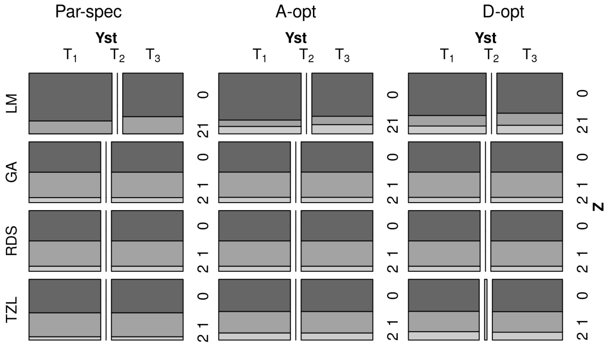
Figure S5: Mosaic plots with the average strata sizes across replicates of the resulting designs in the realistic simulation across optimality criteria (parameter-specific, A-/D-optimality) for n = 2500 .
