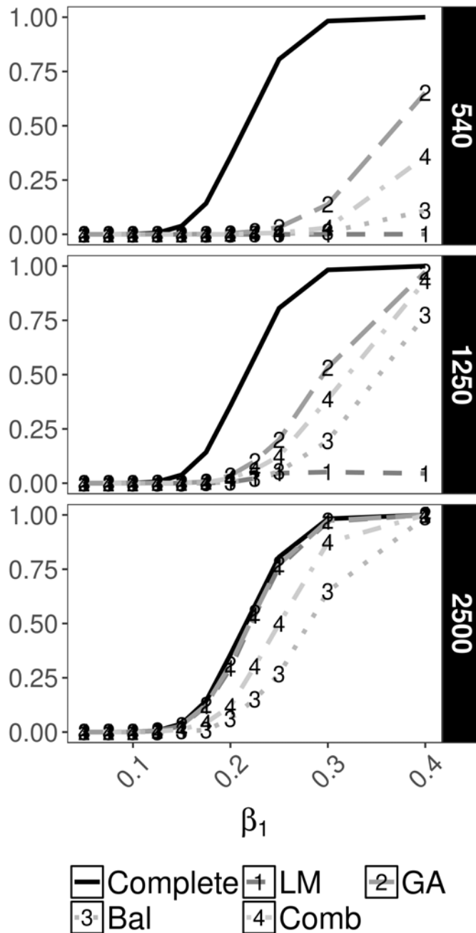
Figure S15: Power curves under the alternative \beta_1 \neq 0 at \alpha = 1 \times 10^{-8} for testing H_0 : \beta_1 = 0 under the LR test and parameter-specific criterion comparing designs (LM,GA,Bal,Comb) across phase 2 sample sizes. Row facets denote different phase 2 sample sizes ( n = 540, 1250, 2500 ). For LM and GA, J(\Phi)^{-1} was used in the optimization criterion.
