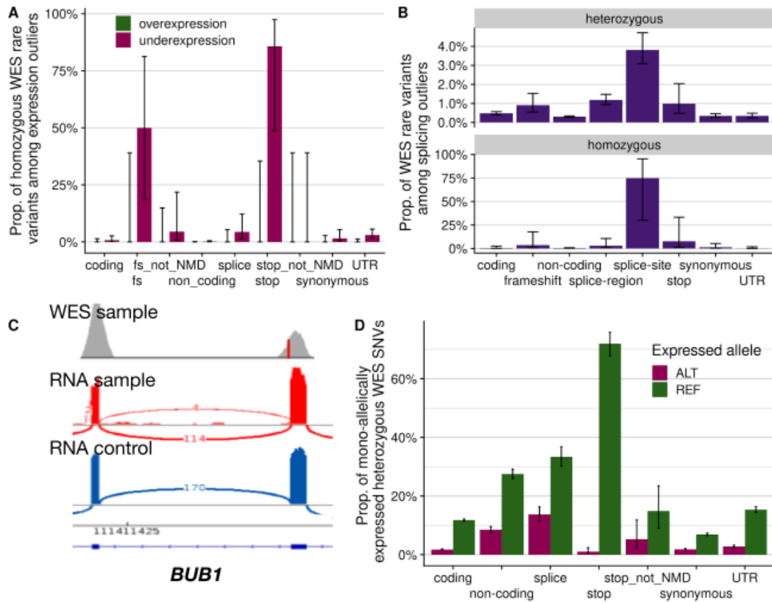
Supplementary figure 9: Rare variants leading to outliers. (A) Proportion of homozygous WES rare variants stratified by VEP class in genes that are aberrantly expressed. Error bars represent 95% confidence intervals of a binomial test (also in panels (B) and (D)). (B) Proportion of WES rare variants (both heterozygous and homozygous) stratified by VEP class in genes with an aberrantly spliced junction. (C) Sashimi plot presenting normal splicing on the gene BUB1 in spite of a homozygous variant in the direct splice-site (shown in red) of a candidate sample. (D) Proportion of rare heterozygous WES SNVs that are mono-allelically expressed towards either the reference or alternative allele, stratified by VEP class. In panels (A) and (D), ‘not NMD’ corresponds to stop or frameshift (fs) variants that are predicted to escape NMD due to being in either the last exon of the gene or in a position that is not expressed in fibroblasts.
