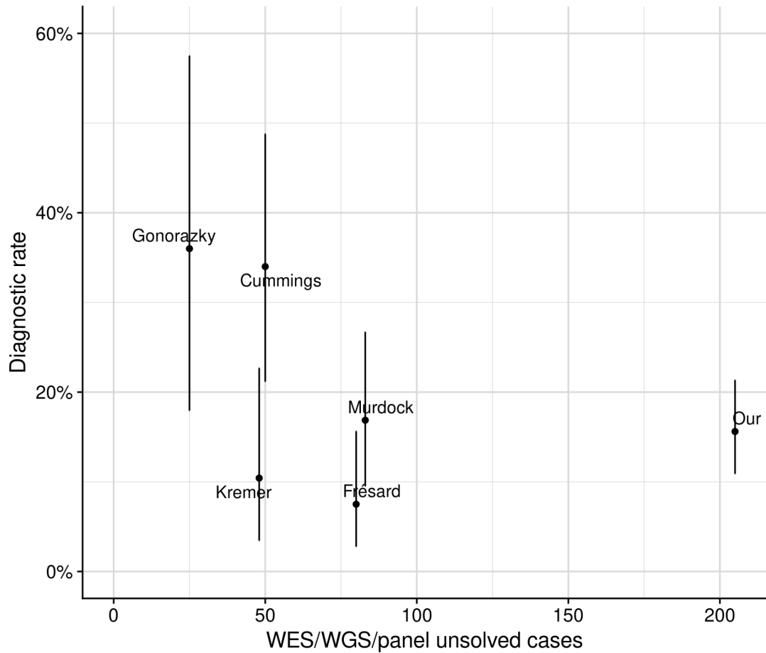
Supplementary figure 10: Diagnostic rate across different cohorts. Diagnostic rate (solved cases / cohort size) vs. cohort size, defined as the number of cases that were unsolved after either WES, WGS, or panel sequencing, across five published cohorts (23-26, 28) and our study. Error bars stretch a 95% confidence interval of a binomial test. A diagnostic rate exceeding 30%, such as in Cummings et al. (24) and Gonorazky et al. (26), could be reached by more stringent inclusion of patients with either variants of uncertain significance in splice regions or unsolved cases where phenotype is a strong predictor of genotype.
