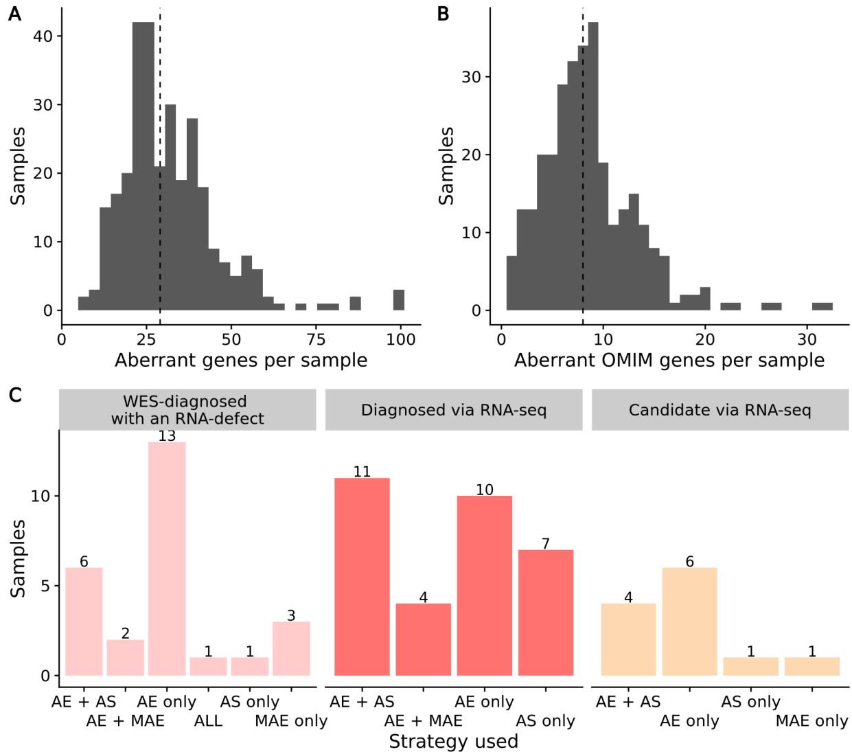
Supplementary figure 4. Aberrant events per sample. (A) Distribution of the number of aberrant genes (union of aberrant expression, aberrant splicing, and MAE). Genes harboring many splice aberrations or rare MAE variants are counted only once. The dashed line corresponds to the median at 29. (B) Same as (A) but for genes known to cause a Mendelian disease (OMIM genes). The dashed line corresponds to the median at 8. These correspond to the genes of clinical relevance. (C) Causative and candidate RNA-seq aberrant events detected by our pipeline across the 26 WES-diagnosed cases with a protein-truncating variant and defect in RNA-seq (Supplementary figure 1), the 32 RNA-seq diagnosed cases, and the 12 RNA-seq candidates cases. AE: aberrant expression, AS: aberrant splicing, MAE: mono-allelic expression.
