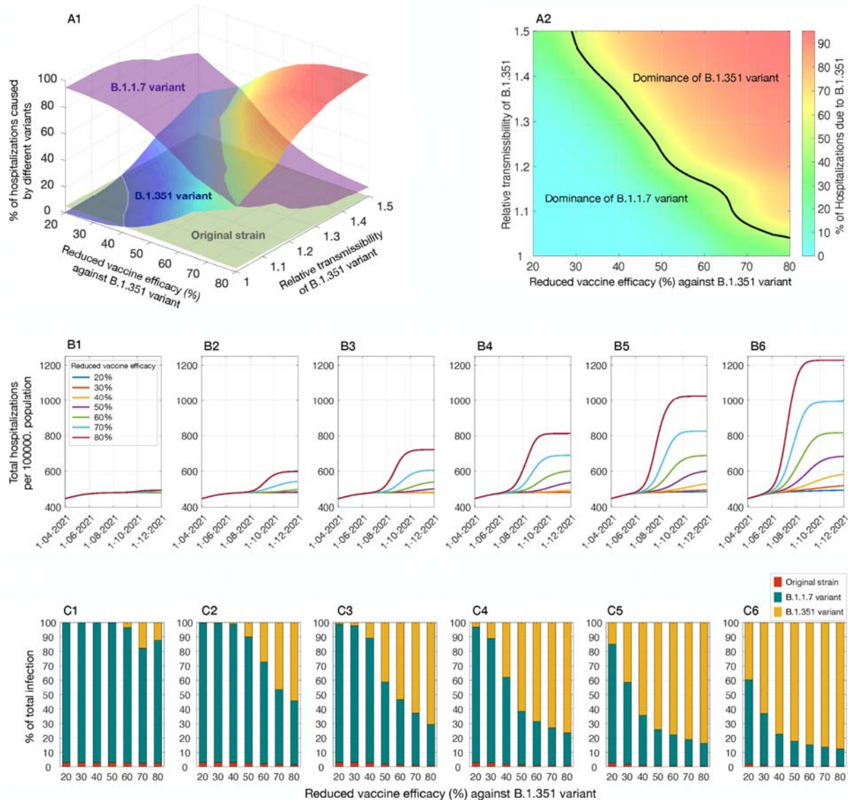
Fig. 1. Projected hospitalizations and infections caused by the variants and the original strain between April 3 to December 31, 2021 (A1) Percentage of hospitalizations due to infections by different variants, with varying transmissibility of B.1.351 relative to the original strain, and reduced efficacy of Moderna vaccines against B.1.351. (A2) Dominance regions in percentage of hospitalizations caused by B1.1.7 and B.1.351 separated by the threshold curve. (B1-B6) Total hospitalizations per 100,000 population for B.1.351 transmissibility increased by a factor of: 1 (B1) , 1.1 (B2) , 1.2 (B3) , 1.3 (B4) , 1.4 (B5) , 1.5 (B6) relative to the original strain. (C1-C6) Percentage of total infections caused by different variants corresponding to the relative transmissibility of B.1.351 in B1-B6.
