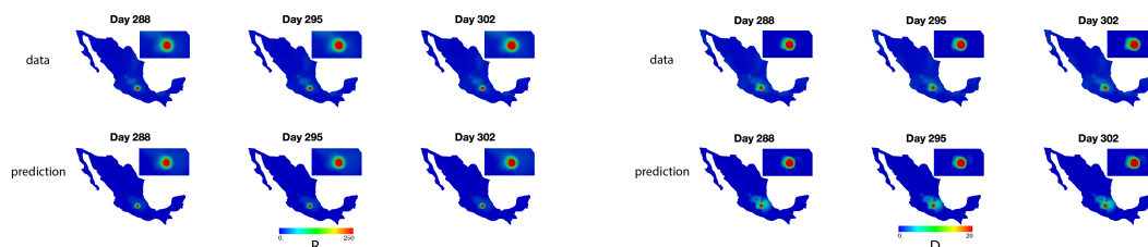
Figure 10: Prediction of the recovered and deceased sub-populations for 3 weeks against with the data at Mexico. The inset in the Mexico plot is a magnified view of Mexico City area.
