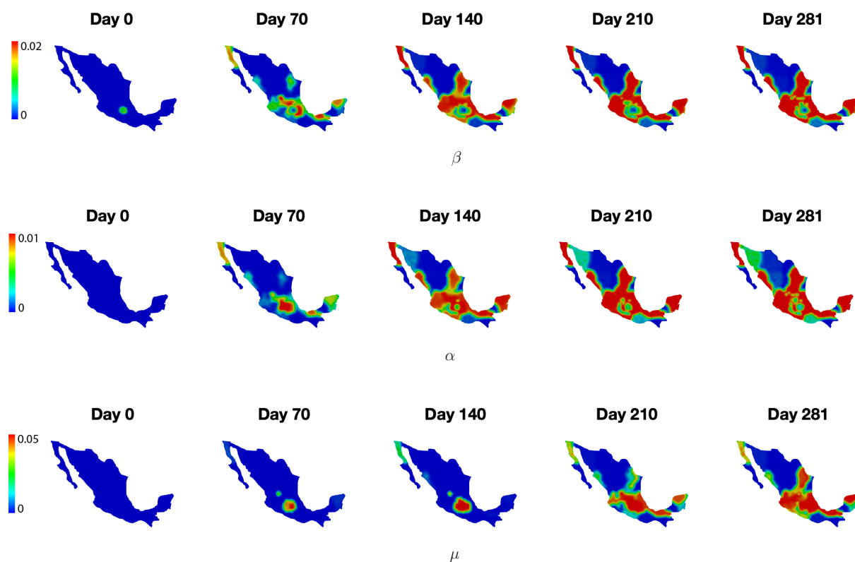
Figure 5: Inferred infection rate ( \beta ), death rate( \alpha ), recovery rate ( \mu ) in Mexico starting from lockdown, March 23, 2020. Time-resolved dynamics may be seen as movies in Supplementary Information: michigan_parameter.mp4.
