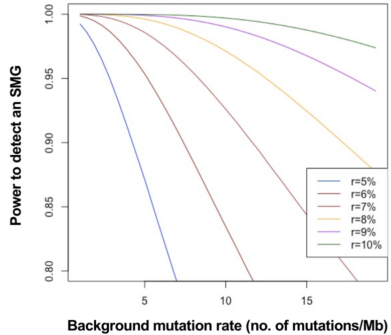
S1 Figure. Power to detect significantly mutated genes (SMGs) in early-stage tumors. Curves show statistical power for different percentages ( r ) of tumors that are somatically mutated. Calculations were performed as described in the text, assuming 270 tumors and 14 gene tests completed.
