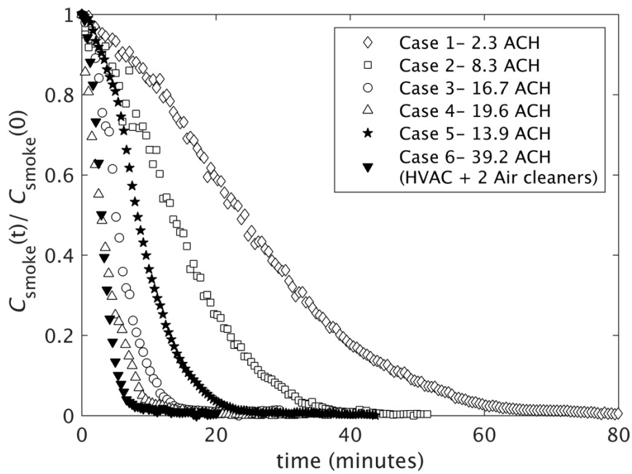
Figure 2: Smoke particle density decay with time. Aerosol particle density, C_{\text{smoke}}(t) , is measured as light intensity of images acquired and normalisation is by the initial light intensity, C_{\text{smoke}}(0) , which is smoke particle density. The white and black symbols indicate the smoke concentration decay rate measured in control room and real hospital room, respectively.
