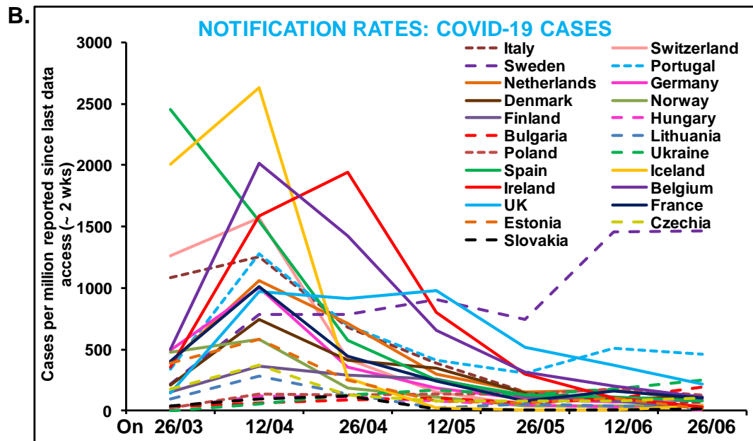
Supplementary Figure 2. The waves of COVID-19 deaths (8 out of 10 were elderly)( A ) as it passed through countries under study and incidence rates (majority younger – without dysregulated Zn homeostasis) ( B ).
